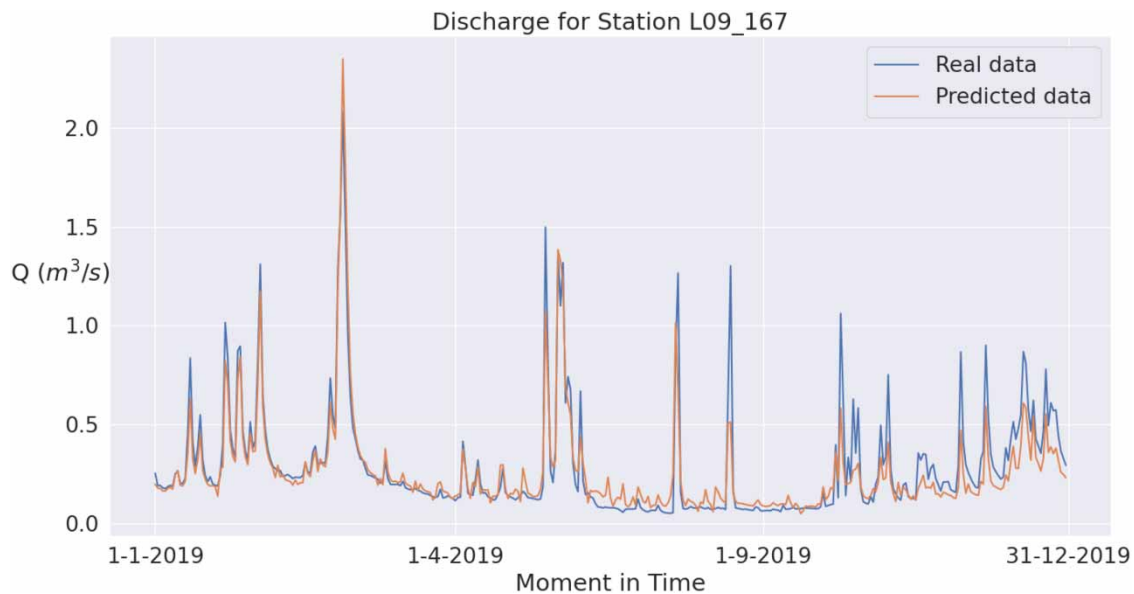
Figure 6 | Plot of the disaggregated data prediction against the measured discharge at station L09_167 for the year 2019.
