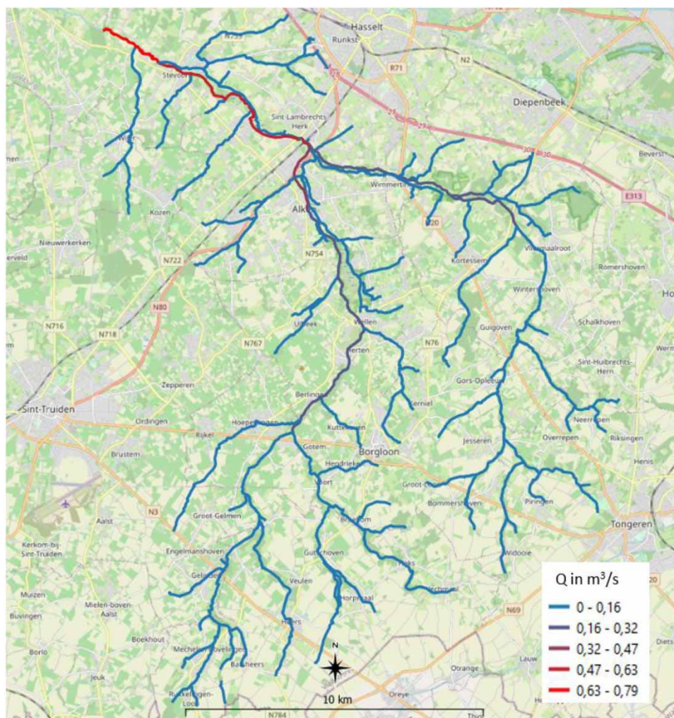
Figure 5 | The result of the disaggregation shown for the Herk case. The discharge is shown for the 31st December of 2019 for each segment separately.
