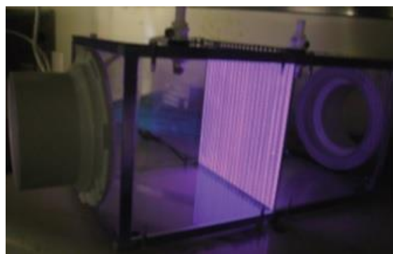
Fig IV.3 Pathogen Detection and Remediation Facility (PDRF): above - general view, below - Dielectric Barrier Grating Discharge (DBGD) with air sterilization chamber. [99]
