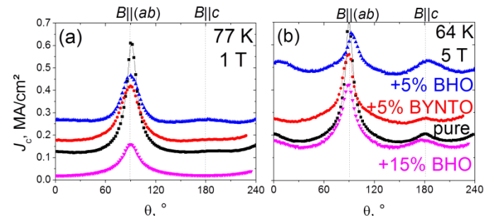
Fig. 8. Angular dependence of J_c at 77 K / 1 T (a) and 64 K / 5 T (b) for pure YBCO, BYNTO, low BHO and highly BHO doped YBCO films deposited at 830^\circ\text{C} on Ni5W, R = 1.6 \text{ nm/s} .
