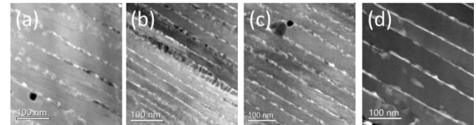
Fig. 10. ADF-STEM images of a 5 mol% BHO:YBCO films deposited at 810°C (a), 10 mol% BHO / 770°C (b), 10 mol% BHO / 810°C (c), 10 mol% BHO / 840°C (d) on ISD-MgO.
