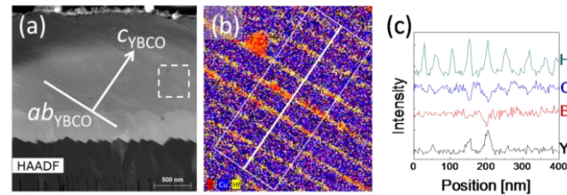
Fig. 9. HAADF-STEM image (a) together with STEM-EDX mapping (b) and integrated element line scan of Hf, Cu, Ba, Y (green, blue, red and black respectively) (c) of 10 mol% BHO:YBCO on ISD-MgO. (HAADF STEM image showing the mapped area by a white square, the composite STEM-EDX mapping showing the area of the integrated line scan by a white rectangle.)
