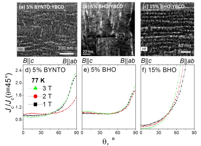
Fig. 7. Spatial distribution of BYNTO and BHO in 5 mol% BYNTO (a), 5 mol% BHO (b) and 15 mol% BHO doped (c) YBCO films, observed as bright contrast in HAADF-STEM (b) and STEM-EDX elemental mappings with respective normalized J_c anisotropy curves at 77 K for several magnetic fields (d)-(f) (All films deposited at 830^\circ\text{C} on Ni5W, R = 1.6 \text{ nm/s} ).
