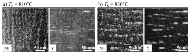
Fig. 3. STEM-EDX elemental mappings of Nb and Y for BYNT0:YBCO samples deposited at 810^\circ\text{C} (a) and 830^\circ\text{C} (b) on ABAD-YSZ using a deposition rate of R = 1.3 nm/s.
