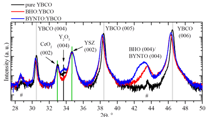
Fig. 1. \theta -2 \theta scans for YBCO, BHO:YBCO and BYNTO:YBCO deposited on ABAD-YSZ at T_s = 810^\circ\text{C} and R = 1.3 \text{ nm/s} (# denote peaks from the underlying metal tape).
