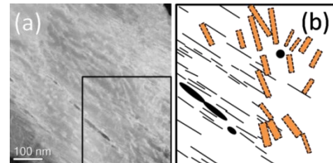
Fig. 11. ADF-STEM image of a 5% BHO:YBCO film on ISD-MgO (a) (deposition conditions T_S = 770^\circ\text{C} , R = 5.4 nm/s). The microstructural features of the inset are sketched (b) including large Y_2O_3 precipitates (black ellipsoids), extra CuO_2 chains (black lines) and short BHO columns (orange rectangles).
