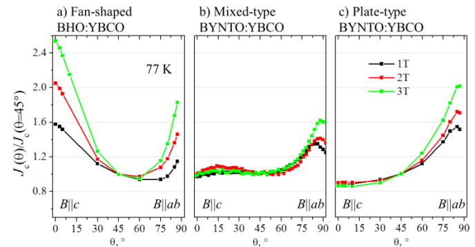
Fig. 6. Angular dependence of the critical current density, J_c(\theta) , of fan-shaped BHO:YBCO (a), mixed-type BYNT0:YBCO (b) and plate-type BYNT0:YBCO samples deposited on ABAD-YSZ. Data for (a) and (c) were obtained by VSM measurements, for (b) by transport measurement. J_c data were taken at 77 K and normalized to J_c(\theta = 45^\circ) .
