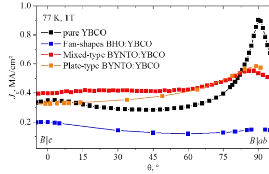
Fig. 5. Angular dependence of the critical current density, J_c(\theta) , at 77 K / 1 T of fan-shaped BHO:YBCO and mixed-type and plate-type BYNT0:YBCO samples deposited on ABAD-YSZ.
