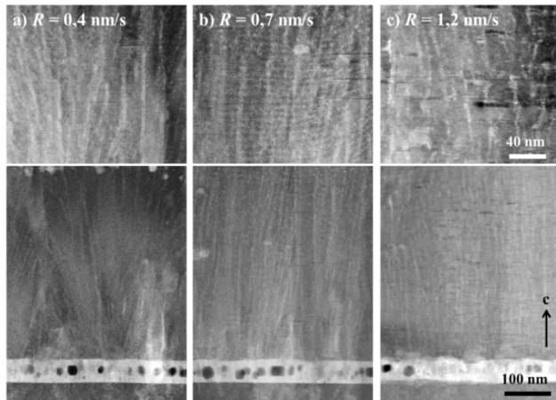
Fig. 2. ADF-STEM images of BHO:YBCO samples on ABAD-YSZ prepared at T_s \sim 800^\circ\text{C} and growth rates of R = 0.4, 0.7 and 1.2 nm/s. Top: BHO:YBCO bulk region (higher magnification). Bottom: BHO:YBCO/tape interface region. The dark spots in the bright \text{CeO}_2 -layer are Ba-rich precipitates.
