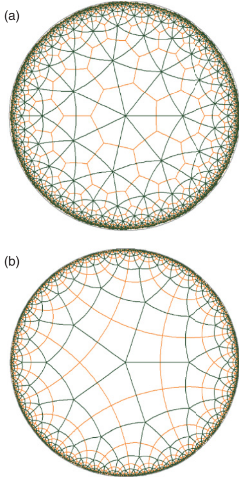
FIG. 1. (Color online) Hyperbolic tessellations in a Poincaré disk. The Shchläfli symbols \{p, q\} describe tessellations where q regular p -gons meet at each vertex: (a) \{3, 7\} and (b) \{4, 5\} (shown by dark green/black lines). The corresponding dual tessellations (a) \{7, 3\} and (b) \{5, 4\} are shown by orange (gray in black and white) lines.
