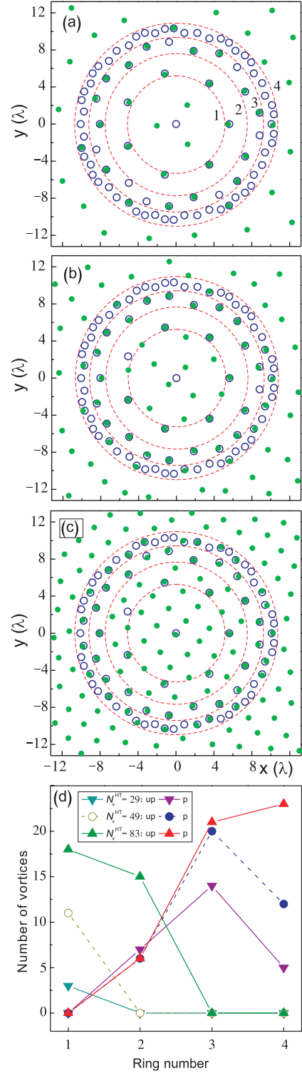
FIG. 2. (Color online) Vortex configurations in a \{3, 7\} hyperbolic-tessellation (HT) APS for varying number of vortices per simulation cell (inside the HT): (a) N_v = 49 ( N_v^{\text{HT}} = 29 ), (b) N_v = 81 ( N_v^{\text{HT}} = 49 ), and (c) N_v = 144 ( N_v^{\text{HT}} = 83 ). Pinning sites are shown by dark blue (black) open circles, vortices by green (gray) dots. Red (gray) dashed lines show the boundaries of concentric rings [numbered 1 to 4 (a)] of the same area containing 1, 7, 21, and 56 pins. (d) Number of pinned (p) and unpinned (up) vortices in the rings, corresponding to N_v^{\text{HT}} in (a)–(c), shown by symbols (lines connecting the symbols are guides for the eye).
