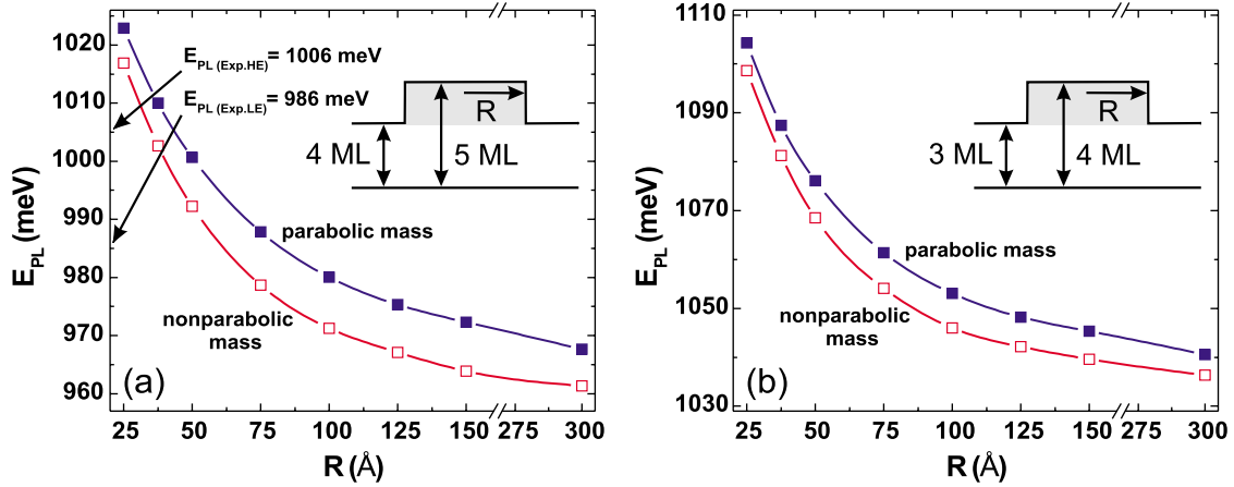
FIG. 8. (Color online) The PL energy as a function of the fluctuation radius R for InAs/InP quantum well with width of 4 ML (a) and 3 ML (b), and fluctuation of 1 ML with the profile shown in the inset of each graph. Symbols are the calculated points and the curves are guides to the eye. The experimental PL energy of the HE and LE peaks is indicated in the inset of graph (a).
