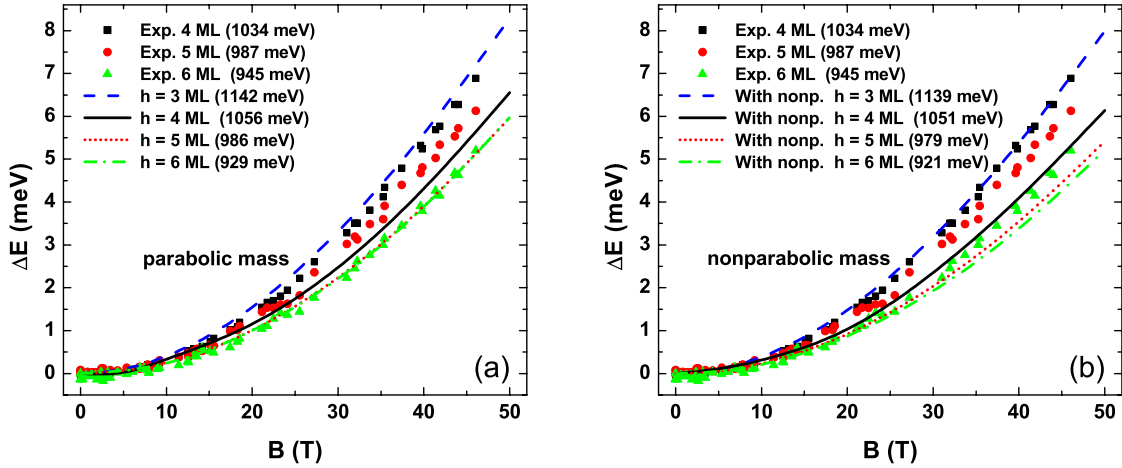
FIG. 3. (Color online) The exciton diamagnetic shift as a function of magnetic field ( B \parallel [110] ) for InAs/InP quantum wires. The dashed (blue), full (black), dotted (red), and short dash-dot (green) curves correspond to our numerical results with parabolic mass of the electron (a) and when the effect of band nonparabolicity is included (b) for different heights of the wire. The full squares (black), circles (red), and triangles (green) represent the experimental data for the wire height 4, 5, and 6 ML, respectively, and width equal to 180 Å. The value of the experimental and the calculated PL energies in the absence of the magnetic field are given in parentheses.
