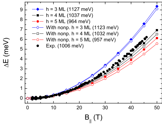
FIG. 4. (Color online) The exciton diamagnetic shift as a function of parallel magnetic field ( \mathbf{B}_{\parallel} \perp \hat{z} ) for InAs/InP quantum wells. The curves with the open and closed symbols correspond to the exciton diamagnetic shift with and without taking into account the effect of band nonparabolicity for the electron, respectively. The curves with the diamonds (blue), squares (black), and circles (red) correspond to the quantum well with width of 3, 4, and 5 ML, respectively. The full circles (black) correspond to the experimental data. The value of the experimental and the calculated PL energies in the absence of the magnetic field are given in parentheses.
