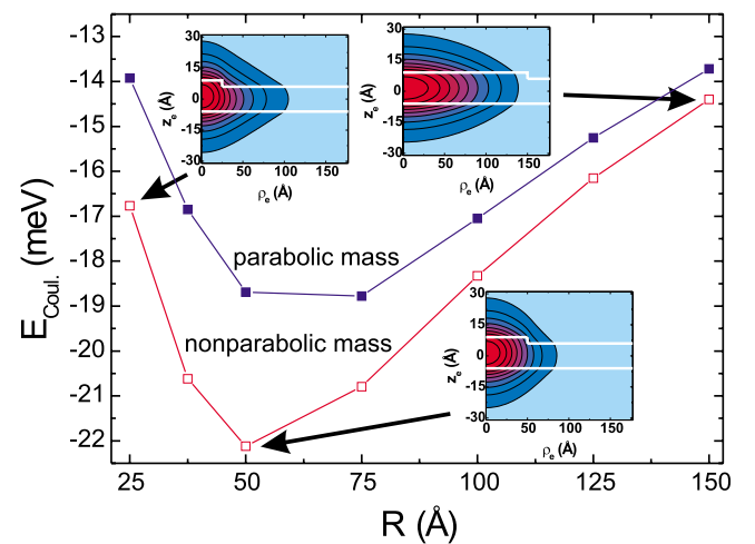
FIG. 9. (Color online) The electron–heavy-hole Coulomb interaction energy as a function of the fluctuation radius R for InAs/InP quantum well with width of 4 ML and fluctuation of 1 ML. The insets show contour plots of the electron density for R = 25 , 50, and 150 Å.
