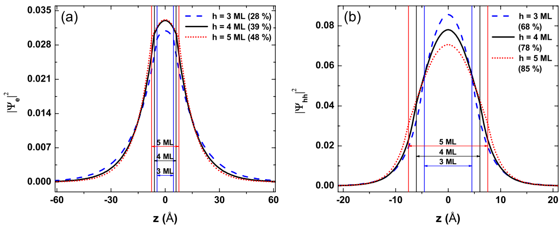
FIG. 5. (Color online) The probability density for the electron (a) and the heavy hole (b) along the growth direction ( z direction) in a InAs/InP quantum well with widths 3, 4, and 5 ML (the dashed (blue), full (black), and dotted (red) curves, respectively). The probability of the electron and the heavy hole to be inside the quantum well is indicated in parentheses.
