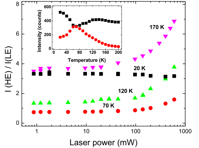
FIG. 6. (Color online) Laser power dependence of the ratio of the intensities of the HE and LE peaks of the quantum well at the different temperatures denoted by the different symbols. At 20 K, this ratio remains constant with varying laser power. With increasing temperature, the laser power dependence becomes more pronounced. The inset shows the temperature dependence of the absolute intensities of the HE [squares (black)] and LE [circles (red)] peaks.
