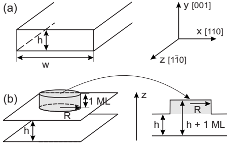
FIG. 1. Schematic drawing of (a) our model of rectangular self-assembled InAs/InP quantum wire with height h and width w , and (b) our model of two-dimensional InAs/InP quantum well with width h . The quantum well width fluctuation of 1 ML and radius R is modeled by the gray area.
