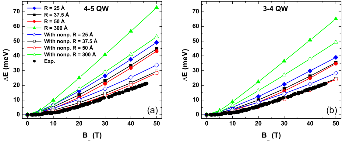
FIG. 10. (Color online) The exciton diamagnetic shift as a function of perpendicular magnetic field ( \mathbf{B}_\perp \parallel \hat{z} ) for InAs/InP quantum well. The curves with the open and closed symbols correspond to the exciton diamagnetic shift with and without taking into account the effect of band nonparabolicity for the electron. The curves with the diamonds (blue), squares (black), circles (red), and triangles (green) correspond to the quantum well with width of 4 ML, fluctuation width of 5 ML (a), and the fluctuation radius of 25, 37.5, 50, and 300 Å, respectively. In graph (b), the same identification of the curves is used as in graph (a), but now for the quantum well with width of 3 ML and fluctuation width of 4 ML. The full circles (black) correspond to the experimental data.
