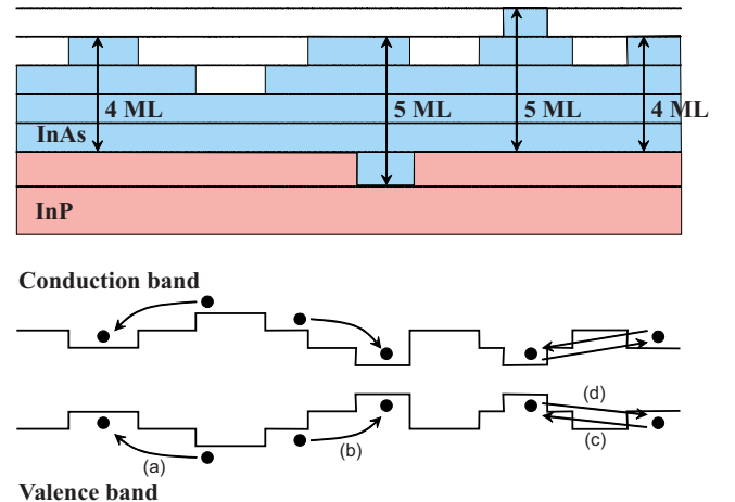
FIG. 7. (Color online) Schematic diagram of the thickness fluctuations within the quantum well (top) and the band structure (bottom). Most excitons can freely move to the most abundant 4 ML fluctuation at all temperatures (a), and some excitons get trapped by a 5 ML fluctuation (b). At moderate temperature excitons are able to migrate from the 4 ML to the 5 ML state (c). At temperatures above 70 K, thermal redistribution causes excitons to migrate from the 5 ML to the 4 ML state (d).
