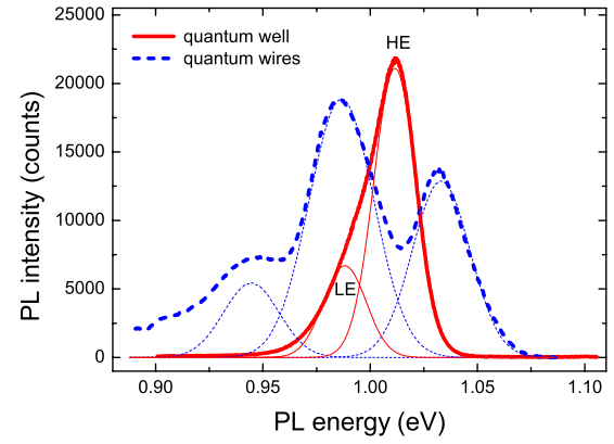
FIG. 2. (Color online) Photoluminescence spectra of the InAs/InP quantum well and wires at 20 K. The thick full (red) and dashed (blue) curves correspond to the PL energies of the well and wires, respectively. The thin full and dashed lines are Gaussian fits to the spectrum.
