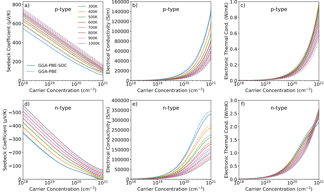
FIG. 10: Electronic transport properties of \text{BaIn}_2\text{Te}_4 calculated with GGA-PBE-SOC (full lines) and GGA-PBE (dashed lines) as a function of carrier concentration with temperatures in the range of 300-1000 K. (a) Seebeck coefficient, (b) electrical conductivity, (c) electronic thermal conductivity for p -type system and (d) Seebeck coefficient, (e) electrical conductivity, (f) electronic thermal conductivity for n -type system.
