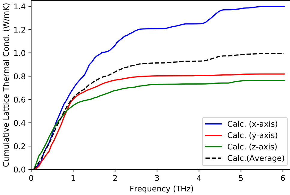
FIG. 6: The cumulative lattice thermal conductivity calculated at 300 K for \text{BaIn}_2\text{Te}_4 along x , y , and z directions together with the average value.
