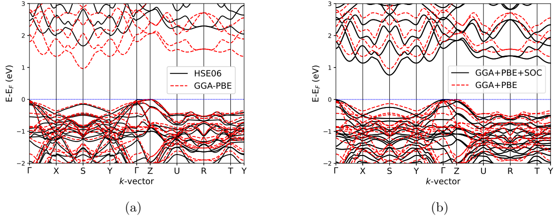
FIG. 7: Electronic band structure of \text{BaIn}_2\text{Te}_4 calculated with (a) HSE06 (full lines) and GGA-PBE (dashed lines) (b) GGA-PBE-SOC (full lines) and GGA-PBE (dashed lines).
