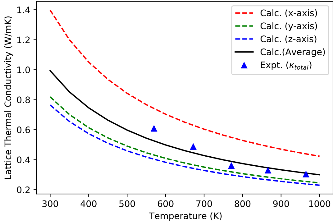
FIG. 4: Lattice thermal conductivity of \text{BaIn}_2\text{Te}_4 along x , y , and z directions together with the average value. The experimental measurement is taken from Ref.[27].
