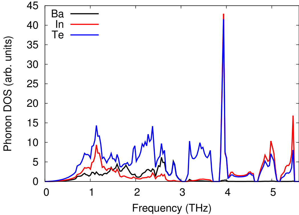
FIG. 3: Total and partial phonon density of states of \text{BaIn}_2\text{Te}_4 .
