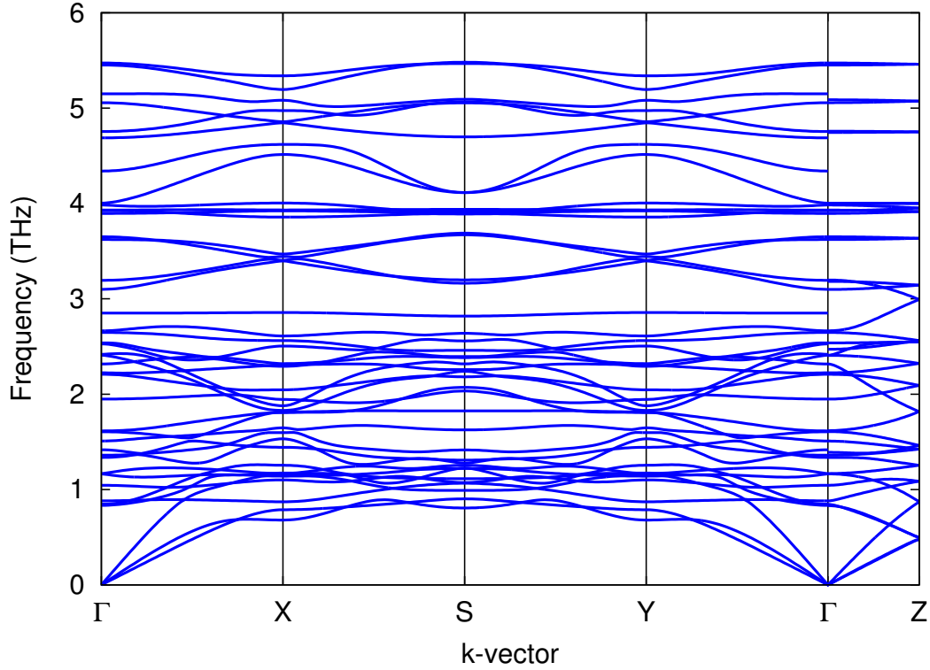
FIG. 2: Phonon dispersion relations of BaIn 2 Te 4 .
