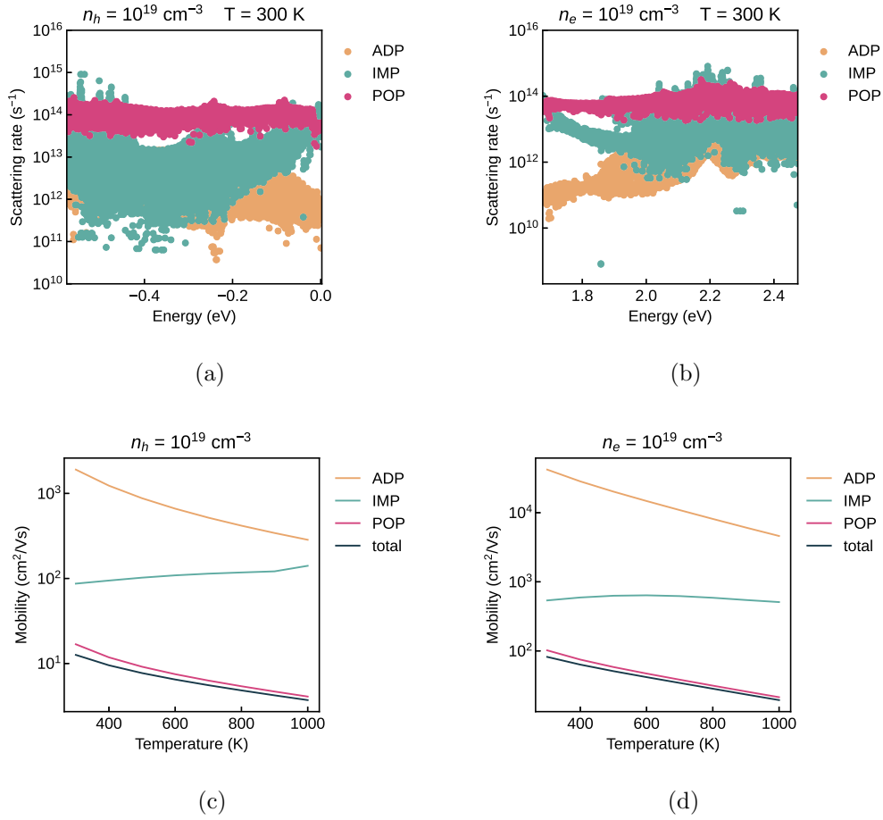
FIG. 9: The total and scattering mechanism resolved room temperature electronic scattering rates for (a) hole doping and for (b) electron doping calculated with GGA-PBE-SOC. The total and scattering mechanism resolved mobility as a function of temperature for (c) hole doping and for (d) electron doping. All the results are given at 10^{19} \text{ cm}^{-3} carrier concentration.
