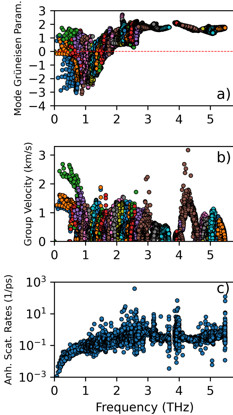
FIG. 5: The calculated (a) mode Grüneisen parameters, (b) phonon group velocities, and (c) anharmonic scattering rates of \text{BaIn}_2\text{Te}_4 .
