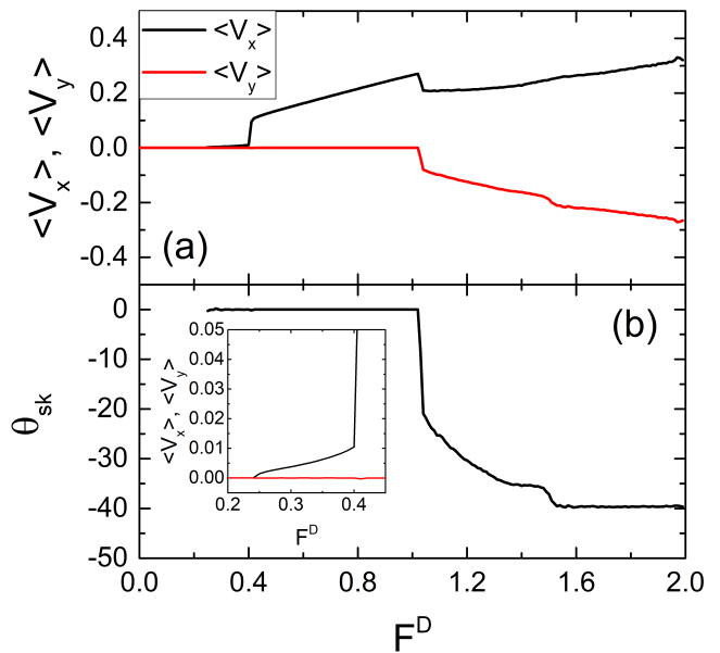
FIG. 8. (a) \langle V_x \rangle (black) and \langle V_y \rangle (red) versus F^D for the 2D sample from Fig. 1(b) with N_{sk}/N_p = 0.99 , \alpha_m/\alpha_d = 1.0 , and \rho_p = 0.373\xi^2 . (b) The corresponding skyrmion Hall angle \theta_{sk} versus F^D . Inset: a blowup of panel (a) over the range 0.2 < F^D < 0.45 .
