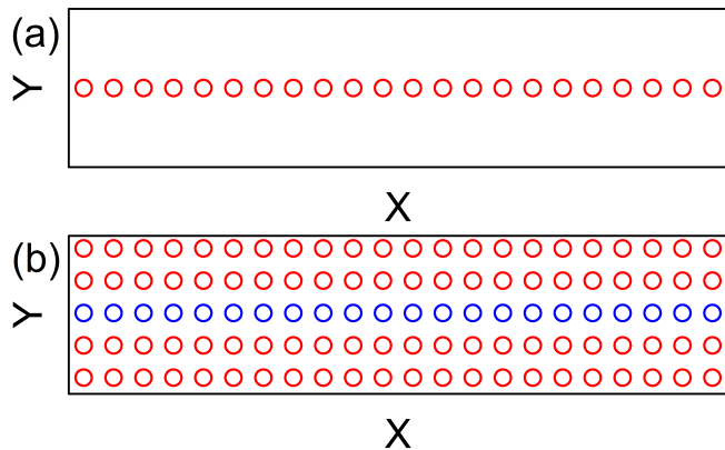
FIG. 1. Illustration of the samples used in this work. (a) The quasi-one dimensional system where the skyrmion motion is confined to a line of Gaussian pinning potentials (circles) by repulsive barriers at y = 0 and y = L_y . (b) The two-dimensional system with a square array of pinning centers and no repulsive barriers. All pinning sites are modeled using Gaussian pinning potentials. Red circles indicate stronger pinning centers and the blue circles are the weaker pinning potentials.
