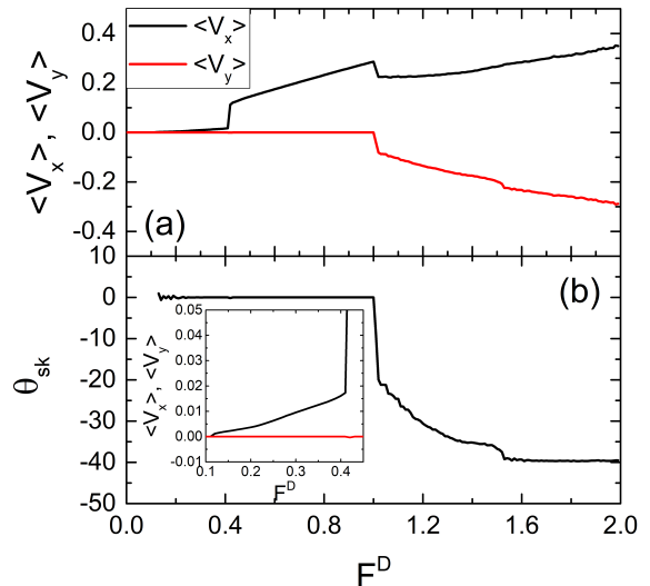
FIG. 6. (a) \langle V_x \rangle (black) and \langle V_y \rangle (red) versus F^D for the 2D sample illustrated in Fig. 1(b) with N_{sk}/N_p = 1.01 , \alpha_m/\alpha_d = 1.0 , and \rho_p = 0.373\xi^2 . Inset: a blowup of panel (a) over the range 0.1 < F^D < 0.45 . (b) The corresponding skyrmion Hall angle \theta_{sk} versus F^D .
