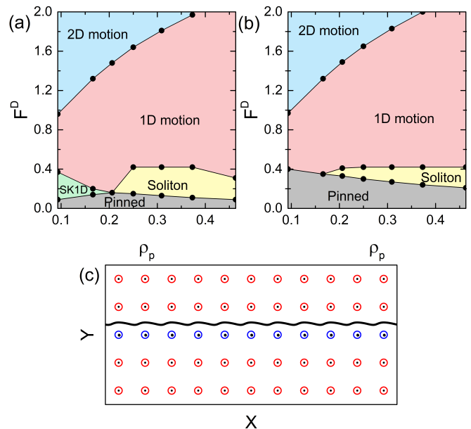
FIG. 11. (a, b) Dynamic phase diagrams as a function of F^D versus pinning density \rho_p for the samples from Fig. 1(b) with \alpha_m/\alpha_d = 0.5 , weak pinning of U_p = 0.15 , and strong pinning of U_p = 1.0 for (a) N_{sk}/N_p = 1.01 and (b) N_{sk}/N_p = 0.99 . Pinned phase: gray; soliton phase: yellow; 1D motion: red; 2D motion: blue; single skyrmion 1D motion (SK1D): green. (c) Pinning site positions (red circles: strong pins; blue circles: weak pins) and the skyrmion trajectories (black lines) for the N_{sk}/N_p = 1.01 sample at F^D = 0.2 and \rho_p = 0.093\xi^2 .
