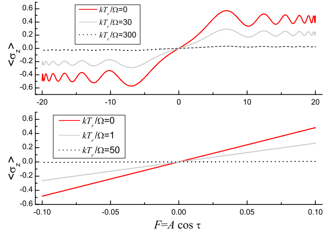
FIG. 6. (Color online) Quasistationary magnetization curves for different parameter values ( \Delta = 1.5 , A = 20 for the upper, \Delta = 0.6 , A = 0.1 for the lower curve) and temperatures. Note that for small values of A , the Floquet states have only a few Fourier components that are not negligible, but this number increases for stronger driving.
