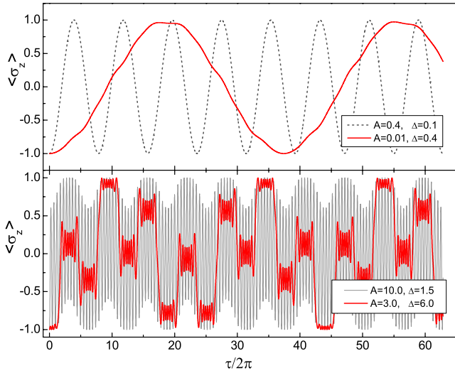
FIG. 2. (Color online) Decoherence-free time evolution of the expectation value \langle \sigma_z \rangle for different parameter values. The initial state is the lower eigenstate of \sigma_z , \rho_s(0) = |-\rangle\langle -| .
