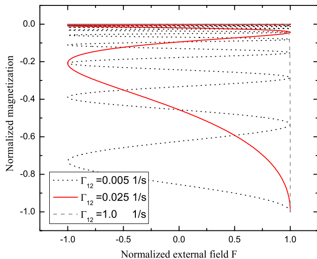
FIG. 9. (Color online) Hysteresis curves for slowly oscillating external fields calculated with assuming incoherent transitions as a consequence of dephasing. The figure corresponds to the seventh resonance (around 3.67 T) of the molecular nanomagnet \text{Mn}_{12} driven by an external field with amplitude of 0.25 T and \Omega = 0.1 1/s. The ladderlike curve for the weakest phonon induced effect (dotted line) reflects qualitatively the results of Ref. [47].
