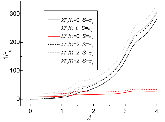
FIG. 5. (Color online) The rate of the decoherence \tau_d^{-1} as a function of the driving field amplitude for different system-environment coupling operators and temperatures.
