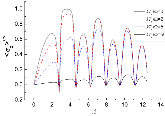
FIG. 3. (Color online) The quasistationary expectation value \langle \sigma_z \rangle^{qs} = \text{Tr}_s(\rho^{qs} \sigma_z) vs the driving field amplitude for \Delta = 1.5 and different temperatures.
