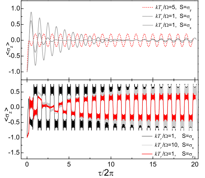
FIG. 4. (Color online) Time evolution of the expectation value \langle \sigma_z \rangle for different parameters and decoherence rates ( A = 0.1 , \Delta = 0.5 , \kappa = 1.0 for the upper, and A = 10 , \Delta = 0.4 , \kappa = 10^{-4} for the lower graph), system-environment coupling operators, and temperatures. The initial state is the lower eigenstate of \sigma_z , \rho_s(0) = |-\rangle\langle -| . Note the emergence of solutions with the same periodicity as that of the driving field.
