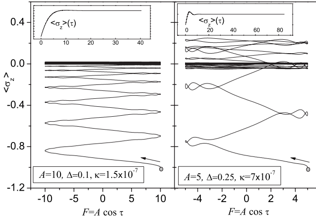
FIG. 7. Convergence toward the quasistationary magnetization curves at high temperatures ( kT_r/\Omega=600 ). The gray dot and the arrow indicate the starting point [corresponding to \rho_s(0)=|-\rangle\langle -| ] and the initial direction. The right panel shows the case of weak decoherence, while environment induced effects are moderate for the left panel. (Note that according to Fig. 5, the same value of \kappa means faster decoherence for larger driving field amplitudes.) The insets show \langle\sigma_z\rangle as a function of \tau/2\pi .
