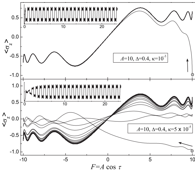
FIG. 8. Convergence toward the quasistationary magnetization curves at low temperatures ( kT_r/\Omega=1 ). The gray dot and the arrow indicate the starting point [corresponding to \rho_s(0)=|-\rangle\langle -| ] and the initial direction. The insets show \langle\sigma_z\rangle as a function of \tau/2\pi .
