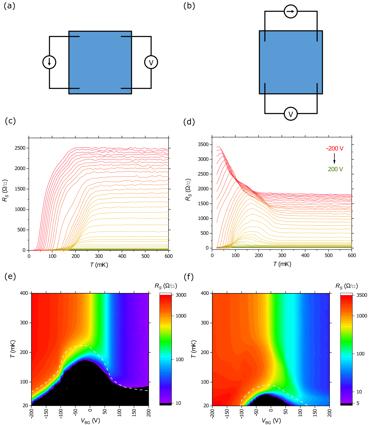
Figure 5. Behavior of the sheet resistance R_S as function of temperature T and back gate voltage V_{BG} for two VDP contact geometries called (a) ‘vertical’ and (b) ‘horizontal’. R(T) curves at different gate voltage with step of 10 V for (c) vertical and (d) horizontal configurations. The same data visualized in color map form for (e) vertical and (f) horizontal configurations.
