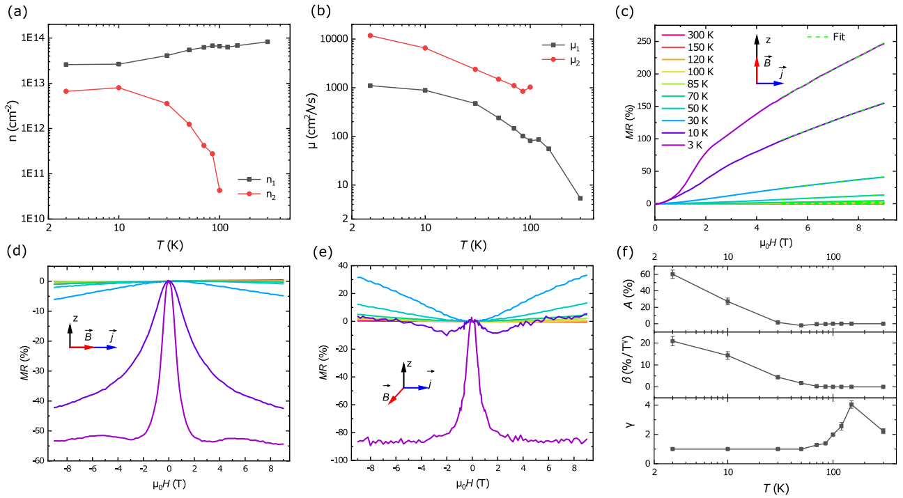
Figure 2. (a) Carrier concentration and (b) mobility versus temperature obtained from a two-band analysis of Hall resistance measurements (given in the supplement). (c)–(e) The MR with magnetic field oriented (c) perpendicular to the sample plane, (d) in-plane parallel to the current direction, and (e) in-plane perpendicular to the current direction. (f) Temperature dependence of the parameters to describe the non-linear out-of-plane MR by fitting equation (2).
