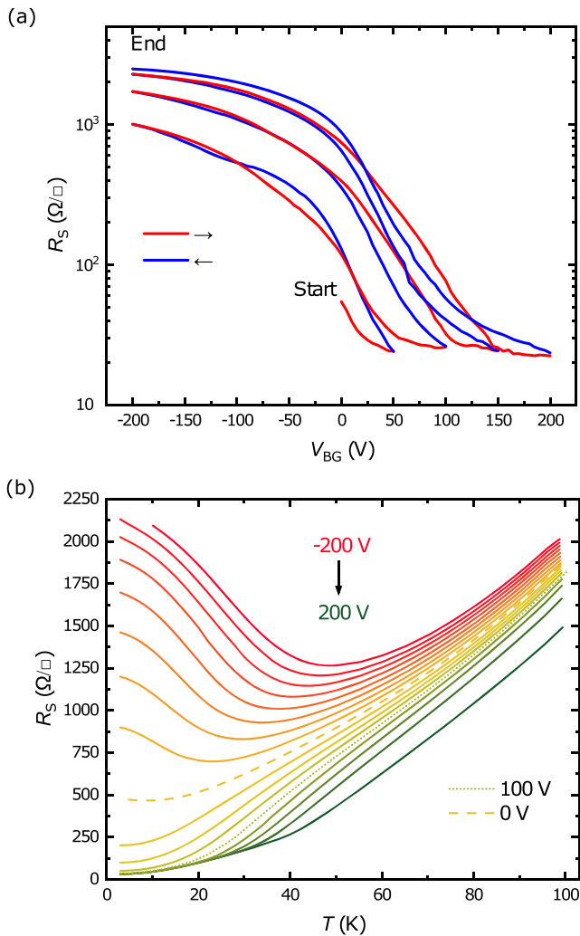
Figure 3. (a) Dependence of the sheet resistance R_S on the back gate voltage. (b) Temperature dependence of R_S for gate voltages from 200 to -200 V with steps of 25 V.
