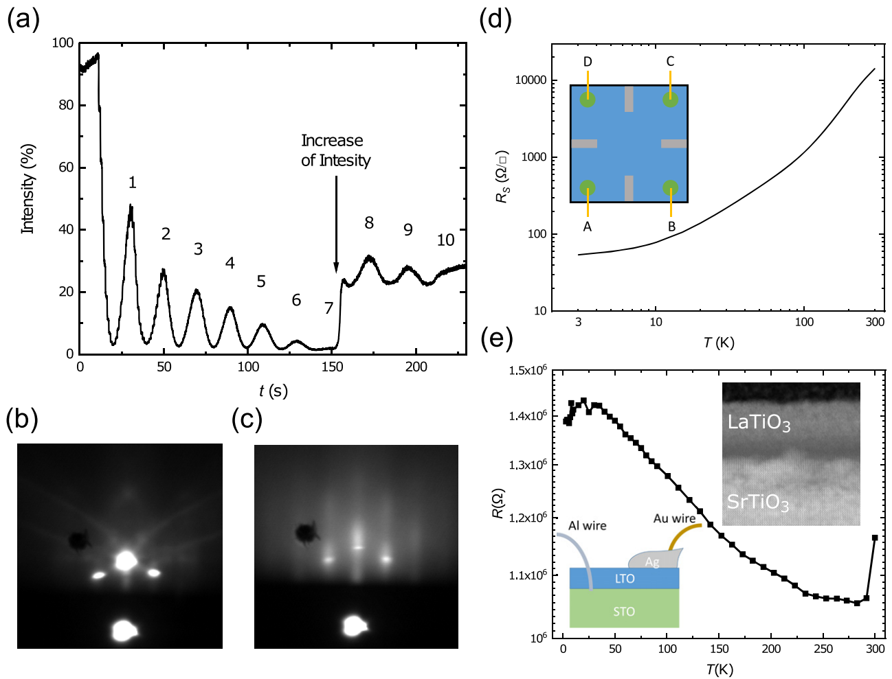
Figure 1. (a) RHEED intensity monitoring during grown 10 u.c. of LTO. RHEED patterns (b) before and (c) after deposition. (d) Temperature dependence of sheet resistance. Insert: sketch of VDP measurements. (e) Temperature dependence of the two-probe measured resistance of the LTO layer. Schematics of two-probe measurement and STEM scan of the LTO/STO interface are shown in the inserts.
