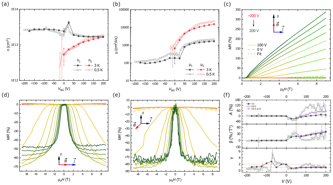
Figure 4. (a) Carrier concentration and (b) mobility versus gate voltage at the temperatures 3 K and 0.5 K as indicated, obtained from a two-band analysis of Hall resistance measurements. (c)–(e) The MR at 3 K with magnetic field oriented (c) perpendicular to the sample plane, (d) in-plane parallel to the current direction, and (e) in-plane perpendicular to the current direction. Note that -200 V is not shown for out-of-plane magnetic field measurements. (f) Temperature dependence of the parameters to describe the non-linear out-of-plane MR by fitting equation (2). Note that near transition from negative to positive high field MR in the range [-110, -80] parameter \gamma and, for some values, \beta were fixed.
