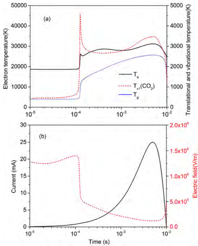
Figure 5. Time evolution of the electron temperature T_e (left axis), the vibrational temperature of the asymmetric mode T_{v_1}(\text{CO}_2) and the gas (translational) temperature T_g (right axis) (a), as well as the discharge current ( I = 25\sin(2\pi 50t) mA) and the electric field (dashed line) (b) at the centre of the arc, at a characteristic frequency of convective cooling of 2.5 kHz.
