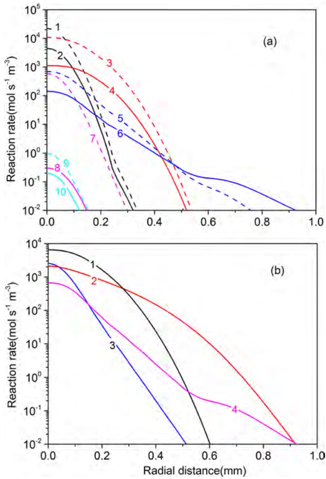
Figure 8. Radial distributions of the reaction rates for CO 2 loss (a) and formation (b) by the most important processes for the quasi-steady state condition, at the same conditions as in figure 2. The numbers of the curves correspond to the reactions listed in tables 7 and 8, for the CO 2 loss and formation mechanisms, respectively. The reactions from the CO 2 vibrational levels are indicated with dashed lines in (a), while the reactions with the CO 2 ground state are plotted with solid lines.
