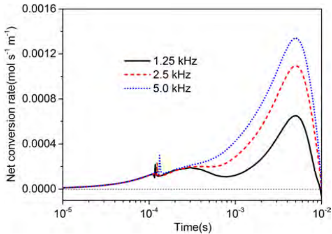
Figure 12. Time evolution of the spatially integrated net conversion rate of CO 2 for different frequencies of convective cooling, at the same condition as in figure 10.
