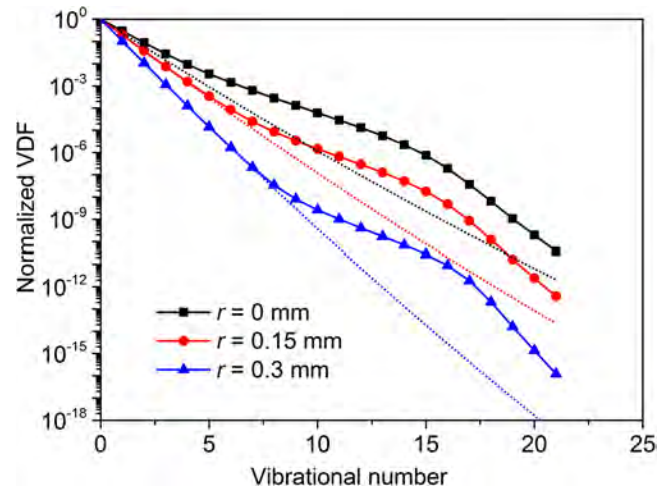
Figure 4. VDFs at different radial positions in the discharge channel, at the same conditions as in figure 2. The dotted lines show the thermal distribution assuming the vibrational temperature equal to the gas temperature.
