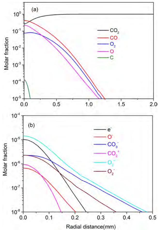
Figure 3. Radial distributions of the molar fractions of the neutral species (a) and charged species (b) in the \text{CO}_2 gliding arc, at the same conditions as in figure 2.
