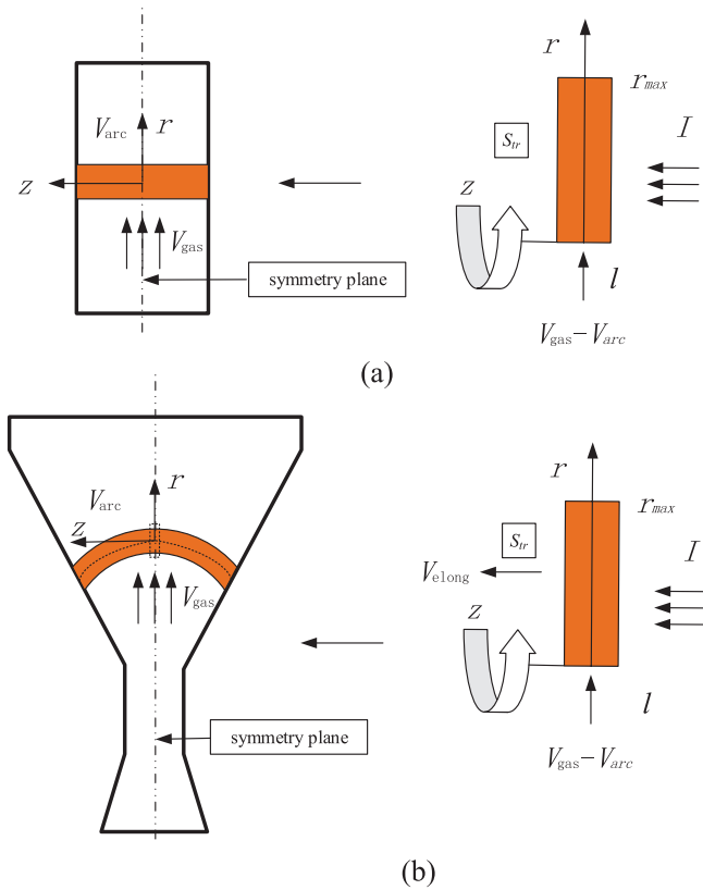
Figure 1. Schematic illustration of the gliding arc geometry, with indication of the quasi-cylindrical arc (left) and the 1D simulation region (right) for the parallel plate gliding arc reactor (a) and diverging electrodes gliding arc reactor (b).
