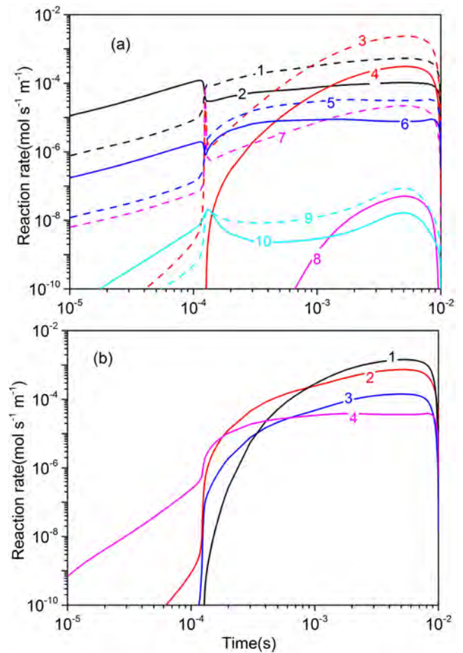
Figure 9. Time evolution of the spatially-integrated rates over the entire arc, for CO 2 loss (a) and formation (b) by the most important processes, at the same conditions as in figure 5. The numbers of the curves correspond to the reactions listed in tables 7 and 8 for the CO 2 loss and formation mechanisms, respectively. The reactions from the CO 2 vibrational levels are indicated with dashed lines in (a), while the reactions with the CO 2 ground state are plotted with solid lines.
