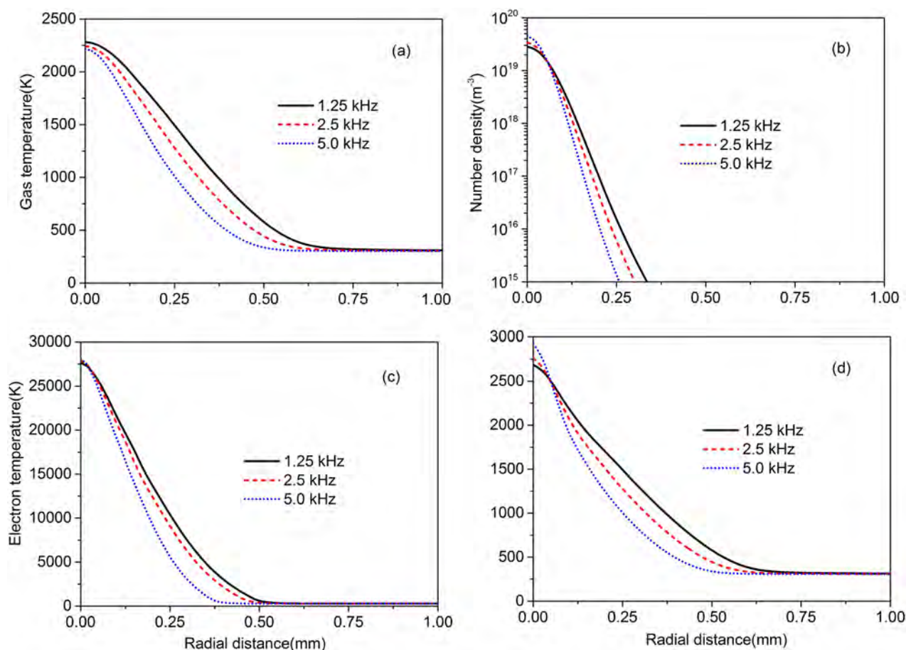
Figure 10. Radial distribution of the gas temperature (a), electron number density (b), electron temperature (c), and vibrational temperature of the asymmetric mode T_{v_1}(\text{CO}_2) (d) for the transient condition, at t = 10^{-3} s and different frequencies of convective cooling.
