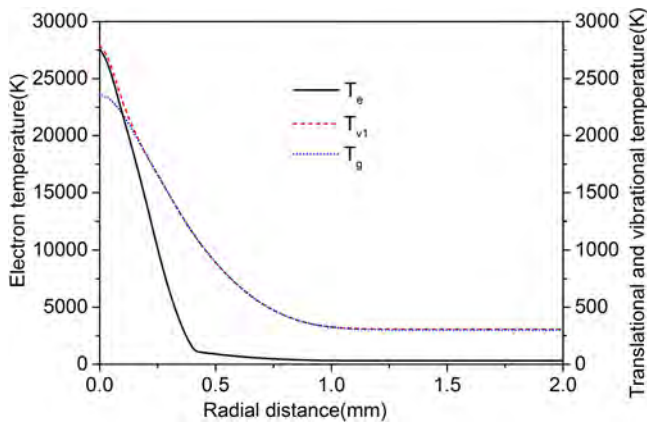
Figure 2. Radial distributions of the electron temperature T_e (left axis), the vibrational temperature of the asymmetric mode T_{v1}(\text{CO}_2) and the gas (translational) temperature T_g (right axis) in the \text{CO}_2 gliding arc, at a discharge current of 10 mA, and a characteristic frequency of convective cooling of 2.5 kHz.
