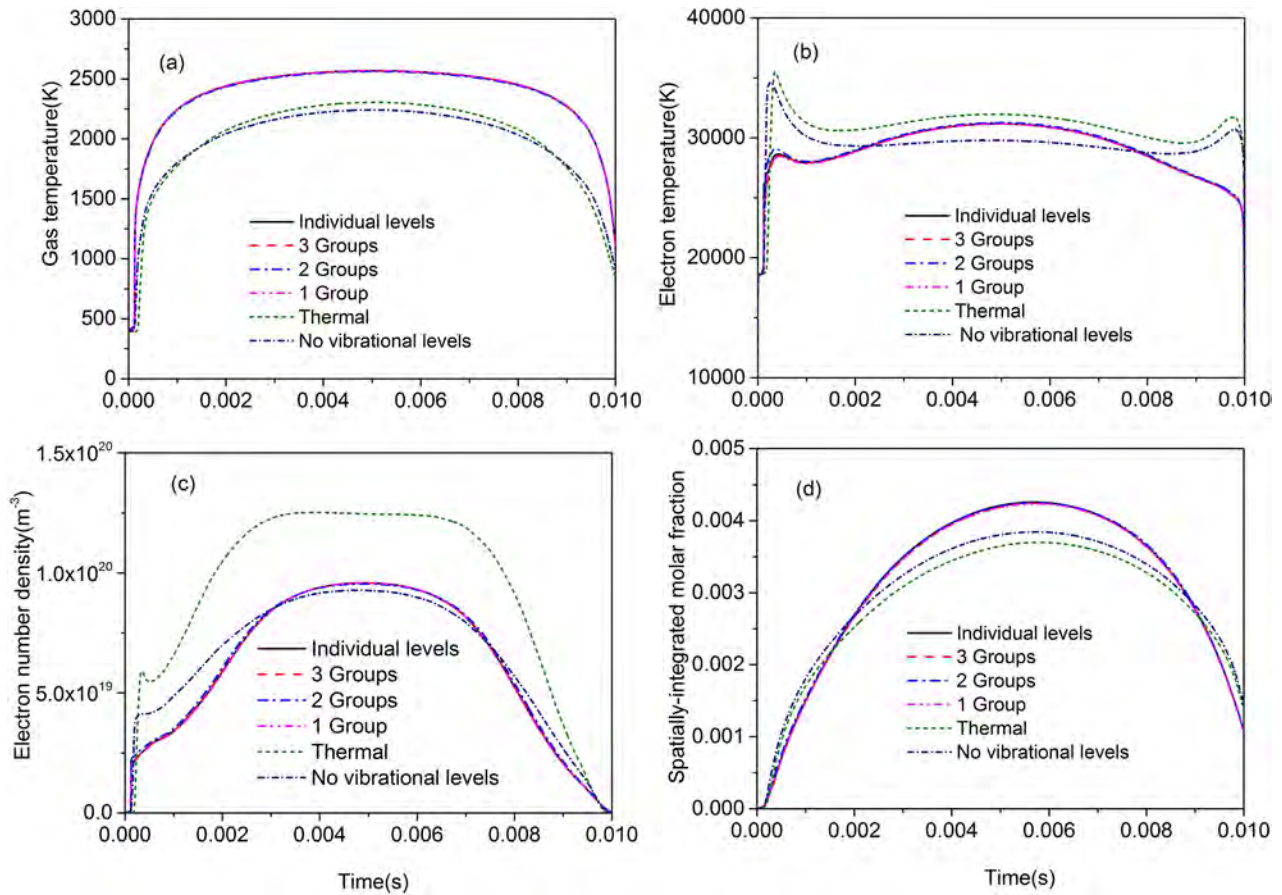
Figure 14. Time evolution of the gas temperature (a), electron temperature (b), electron number density (c) at the center of the arc and the spatially-integrated molar fraction of CO over the whole discharge channel (d), calculated with the different models (see legend).
