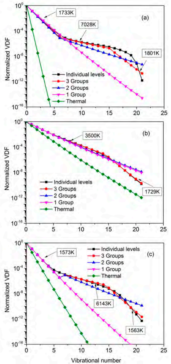
Figure 13. VDFs at t = 1.2 \times 10^{-4} s (a), 5 \times 10^{-3} s (b) and 9.9 \times 10^{-3} s (c), which correspond to the time of gliding arc discharge initiation, the time of the peak current and of the arc extinction stage, respectively (see figure 5(a) above). Comparison is made between the VDFs predicted by the full model, the different lumped-levels models and the thermal distribution model.
