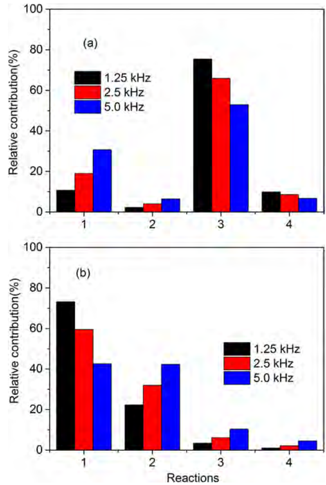
Figure 11. Relative contribution of the most important processes for CO 2 loss (a) and formation (b), at different characteristic frequencies of convective cooling for the transient condition at t = 10^{-3} \text{ s} . The reaction numbers in the x-axis of (a) and (b) correspond to the numbers in tables 7 and 8, respectively. Note that only the four main loss processes are illustrated in (a).
