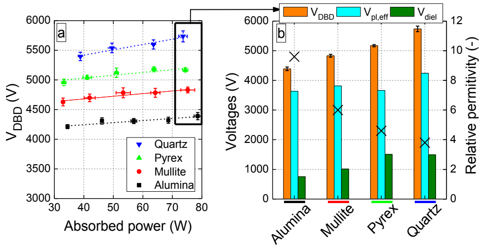
Figure 6 : (a) RMS applied voltage ( V_{DBD} ) as a function of absorbed power for four different dielectric materials at f=27 kHz, and (b) RMS voltage components as a function of the dielectric material at a given absorbed power P_{abs}=75 W; \Phi(CO_2)=200 mL _n .min ^{-1} . The relative permittivities of the materials are indicated with crosses, referring to the right y-axis.
