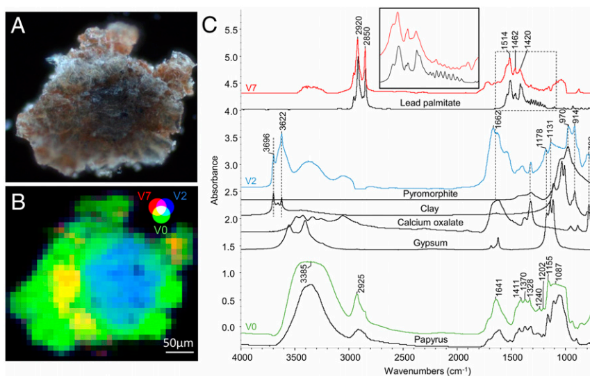
Fig. 6. \mu -FTIR mapping on a section from sample 4. (A) Visible light image of the sample. (B) RGB display of 3 NNMA vectors from the FTIR map (red = V7; green = V0; blue = V2). Beam size: 20 \mu m horizontal \times 20 \mu m vertical. Area size: 380 \mu m horizontal \times 330 \mu m vertical. Step size: 10 \mu m horizontal \times 10 \mu m vertical. (C) NNMA components superimposed on spectra of reference materials: Lead palmitate, pyromorphite, clay (kaolinite), calcium oxalate, gypsum, papyrus (average spectrum acquired on a section of sample 4 far from the ink region).
