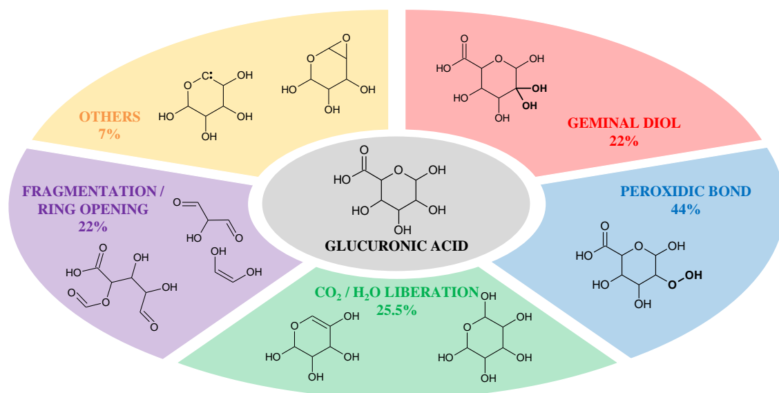
Figure 6. Summary of the main outcomes and associated probabilities obtained from reactive MD simulations. The sum of all the percentages is higher than 100% because some events occur together.
