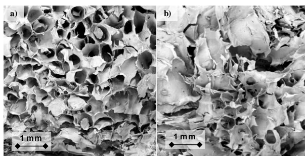
Figure 3. SEM images of the fracture of untreated (a) and 10 min NTP-treated (b) cross-linked alginate from 5 \text{ g L}^{-1} alginate solutions.
