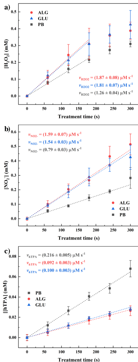
Figure 4. Quantification of NTP-generated reactive species as function of the treatment time in phosphate buffer (PB), 5 g L -1 alginate solution (ALG) and 5 g L -1 (21.7 mM) glucuronate solution (GLU). a) hydrogen peroxide; b) nitrite ions; c) 2-hydroxyterephthalate as indirect measure of OH radicals. The dashed lines are linear fits. The data are expressed as average \pm standard deviation; n = 3. The generation rates of the species, obtained by fitting of the curves, are also listed.
