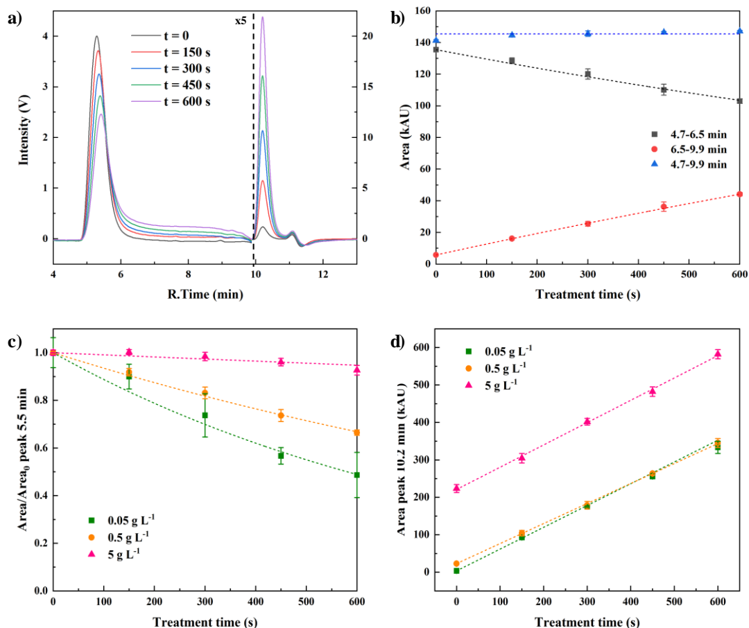
Figure 1. Results of SEC experiments on NTP-treated alginate solutions. a) Chromatograms of 0.5 \text{ g L}^{-1} alginate solutions treated by NTP for different times; the left part of the figure (before the black dashed line) has been enlarged 5 times to emphasize the differences; b) areas of different portions of the chromatograms for 0.5 \text{ g L}^{-1} alginate solutions as function of the treatment time; the dashed lines are exponential (black and red) or linear (blue) fits; c) relative area of the peak centered at 5.5 min as function of the treatment time for 0.05 , 0.5 and 5 \text{ g L}^{-1} alginate solutions; the dashed lines are exponential fits; d) area of the peak centered at 10.2 min as function of the treatment time for 0.05 , 0.5 and 5 \text{ g L}^{-1} alginate solutions; the dashed lines are linear fits. The data in panels b, c and d are expressed as average \pm standard deviation; n = 3 .
