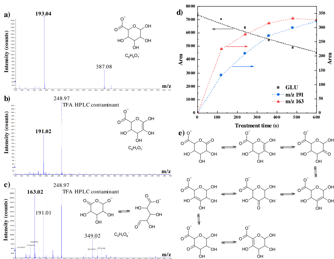
Figure 5. HPLC-ESI-MS analysis of NTP-treated glucuronate. Negative ESI-MS spectra of glucuronate (a) and of the two oxidation products with m/z 191 (b) and m/z 163 (c); intensity of the signal of the 3 compounds as function of the NTP treatment time (d) (the black dashed line is the exponential fit of the
