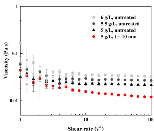
Figure 2. Viscosity profiles of untreated and 10 min-treated alginate solutions. In grey are reported the data for control solutions with higher concentrations (5.5 and 6 g L -1 ) to show the effect of water evaporation.
