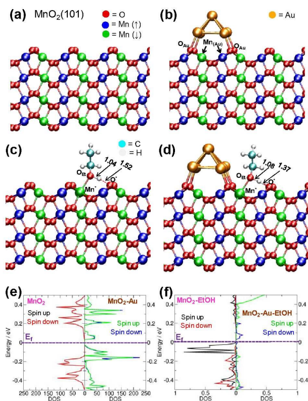
Fig. 4 Graphical representation of: a) bare \text{MnO}_2(101) slab; b) Au-decorated \text{MnO}_2 ; c) EtOH adsorbed on \text{MnO}_2 (c) and \text{Au/MnO}_2 (d) surfaces. Atom colors: O = red; Mn (spin up) = blue; Mn (spin down) = green; Au = orange; C = cyan; H = white. Reported interatomic distances are in Å. e) Density of states (DOS) for bare \text{MnO}_2 (left) and \text{Au/MnO}_2 (right). f) DOS projected on EtOH \text{O}_{2p} -states for EtOH adsorbed on bare \text{MnO}_2 (left) and \text{Au/MnO}_2 (right).
