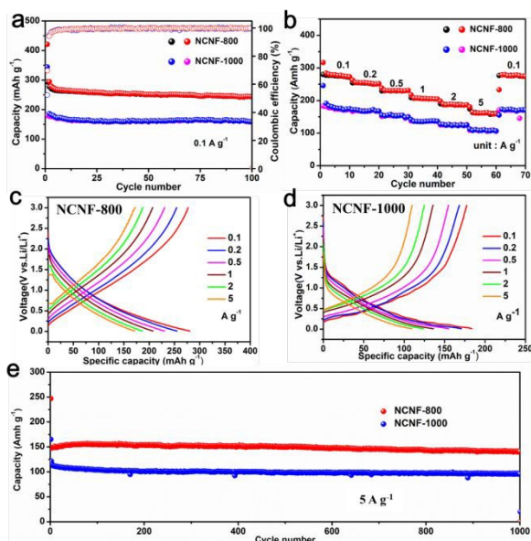
Figure 3. Electrochemical properties of the NCNF-800 and NCNF-1000. (a) Cycling performance of NCNF-800 and NCNF-1000 samples tested at a current density of 100 mA g -1 . (b) Rate performance of NCNF-800 and NCNF-1000 at various current densities from 0.1 to 5 A g -1 . (c, d) The corresponding charge and discharge voltage profiles of NCNF-800 and NCNF-1000 at different current densities. (e) Cycling performance of NCNF-800 and NCNF-1000.
