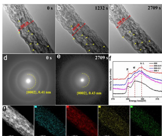
Figure 4. Evolution of morphology and microstructure of NCNF-800 in potassiation. A nanobattery was designed inside the TEM with NCNF-800 as the cathode, potassium metal as the anode, and K_2O grown on the surface of the potassium metal as the solid electrolyte. When a bias of -10 V is applied, a potassiation process is triggered. (a-c) The morphological evolution of NCNF-800 during the potassiation reaction. (d, e) Electron diffraction patterns of NCNF-800 before and after the potassiation reaction. (f) The ex-situ C K-edge spectra from the edge region in different states. (g) STEM-HAADF image and the corresponding STEM-EDS maps of potassiated NCNF-800.
