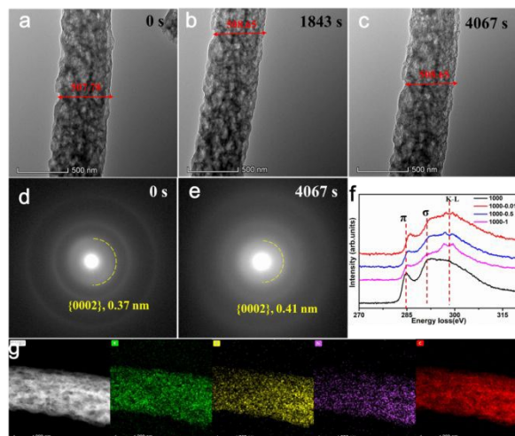
Figure 5. Evolution of morphology and microstructure of NCNF-1000 in potassiation. A nanobattery was designed inside the TEM with NCNF-1000 as the cathode, potassium metal as the anode, and K_2O grown on the surface of potassium metal as the solid electrolyte. When a bias of -10 V is applied, a potassiation process is triggered. (a) The morphological evolution of NCNF-1000 during the potassiation reaction. (d, e) Electron diffraction patterns of NCNF-1000 before and after the potassiation reaction. (f) The corresponding charge and discharge voltage profiles of NCNF-800 and NCNF-1000 at different current densities. (f) Ex-situ C K-edge spectra from the edge region at different states. (g) STEM-HAADF image and the corresponding STEM-EDS maps of potassiated NCNF-1000.
