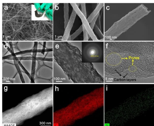
Fig. 1. Morphology characterization of porous NCNF-800. (a-c) SEM images. Inset of (a) is an optical image. (d, e) TEM images. Inset of (e) is a SAED pattern. (f) HRTEM image. (g-i) STEM-HAADF image and the corresponding STEM-EDS mapping for C and N elements.
