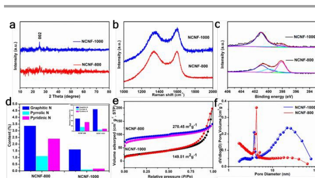
Figure 2. Structure characterization of porous NCNF-800 and NCNF-1000 samples. (a) XRD patterns. (b) Raman spectra. (c) High-resolution N 1s XPS spectra. (d) The corresponding contents of graphitic N, pyrrolic N and pyridinic N from (c). (e, f) BET and BJH curves.
