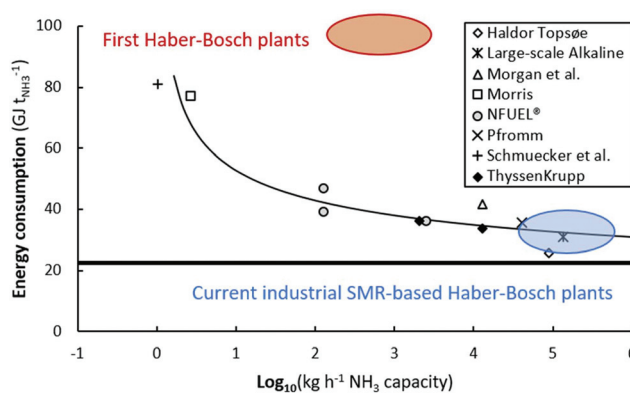
Fig. 4 Energy consumption of various electrolysis-based Haber–Bosch processes (academic and industrial estimates). The bold line represents the thermodynamic minimum energy consumption (20.1 GJ\ t-NH_3^{-1} ). 100 kg\ h^{-1} ammonia corresponds to approximately 1 MW. Original references. 56–65 Reproduced from ref. 20.
