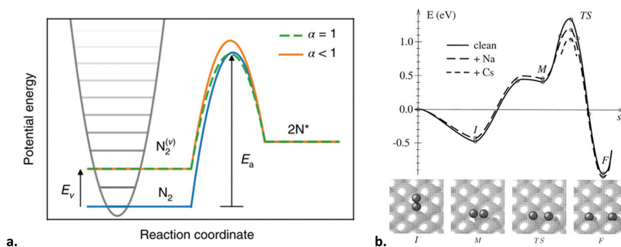
Fig. 12 (a) Proposed impact of vibrational excitation on dissociation barrier of N_2 . Reproduced from ref. 131. (b) Minimum energy path for N_2 dissociation over Ru(0001), without and with alkali promoters. Reproduced from ref. 40.
