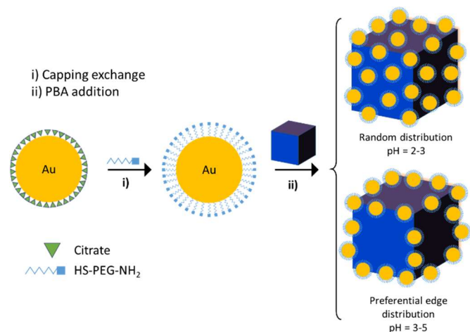
Figure 1. Schematic illustration for the preparation of a heterostructure formed by Au nanospheres decorating PBA NPs. First step involves a capping substitution and the second step the attachment of the Au onto the PBA surface. Two different Au decoration can be achieved by adjusting the pH solution: a random and a preferential distribution along the edges.
