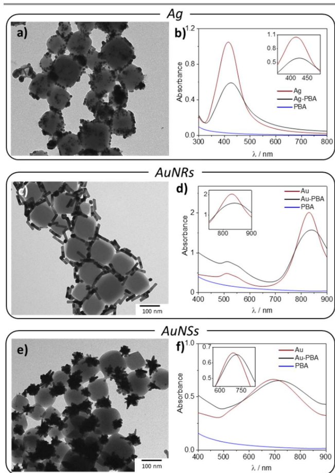
Figure 3. TEM images and UV-Vis spectra obtained for the heterostructures: Ag-PBA, AuNRs-PBA and AuNSs-PBA. The insets show the plasmon band shift.
