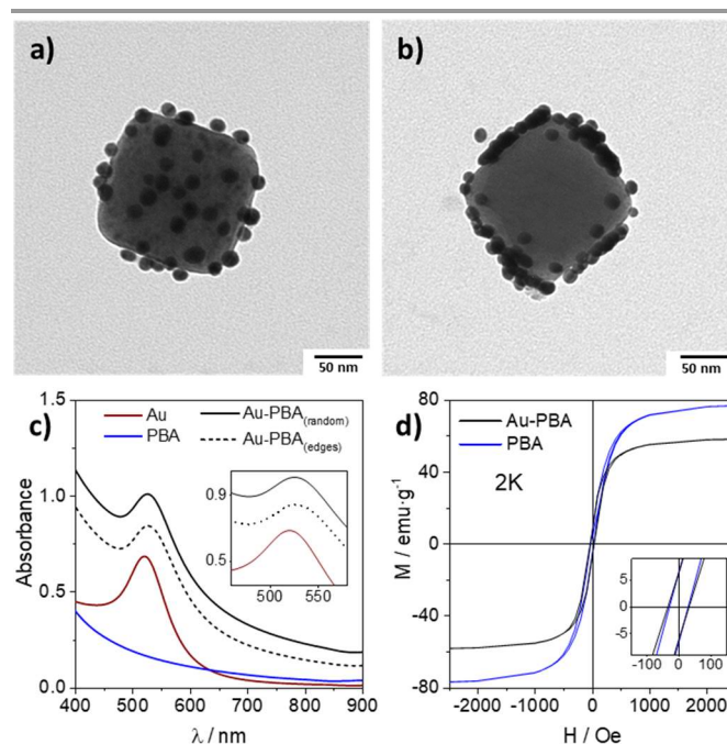
Figure 2. TEM images obtained for a single NP of the heterostructure of Au NPs with (a) random and (b) preferential edge decoration onto NiCr PBA. c) Spectra of Au NPs and Au-PBA heterostructures in the visible region. Inset: magnified image of the plasmon bands. (d) Hysteresis loop at 2K of PBA and Au-PBA.
