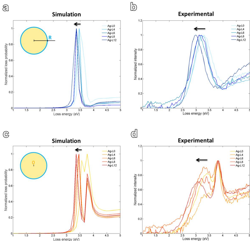
Figure 5: Simulated spectra with impact parameter R (a) and 0 (c). Experimental obtained EELS spectra show a similar trend for both impact parameters.
