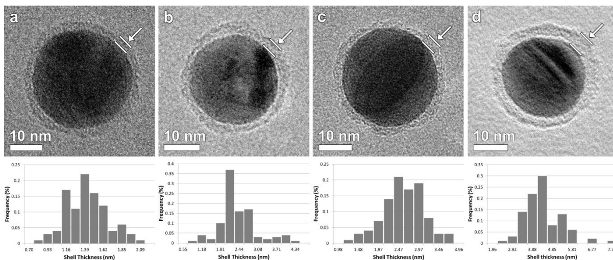
Figure 2: BF-TEM images of (a) Ag-L4, (b) Ag-L6, (c) Ag-L8 and (d) Ag-L12 and corresponding distribution of the shell thicknesses.
