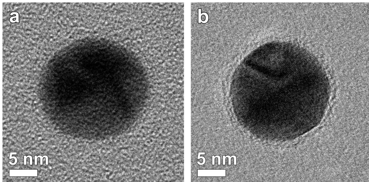
Figure 1: Silver nanoparticles encapsulated by 4 layers of polymer deposited on (a) a commercial Cu TEM grid and (b) ultrathin carbon film coated TEM grid. Only when using an ultrathin support, the polymer shell can be visualized.
