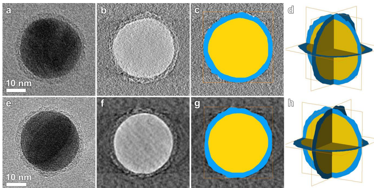
Figure 3: (a, e) BF-TEM projection at 0^\circ for respectively Ag-L4 and Ag-L8. (b, f) Slices through the reconstructed 3D volumes obtained by the weighted back projection and (c, g) superimposed segmentation. Figures (d, h) show the result of the 3D segmentation. The polymer shell (blue) is encapsulating the complete particle (yellow). A 3D visualization is shown in supplementary information.
