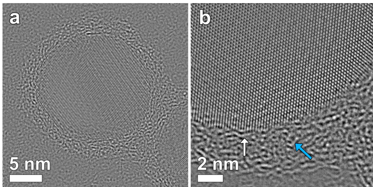
Figure 4: A focal series of 15 HRTEM images is used to perform exit wave reconstruction. Phase images of the reconstructed exit wave of different particles show clearly the presence and position of the polymer shell around the particles. The white arrow indicates the presence of parallel oriented polymer chains, while the blue arrow shows the presence of chains in different orientations.
