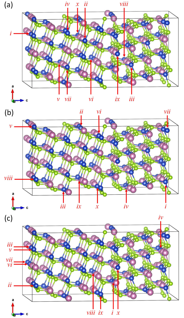
FIG. 9: Location of the ten lowest energy positions for (a) V_{Cu} , (b) In_{Cu} , and (c) Na_{Cu} . The numbering is such that E_i < E_{ii} \dots < E_x . (a) The V_{Cu} with the lowest energy ( i ) is at the side GB, but the other nine lowest energy locations occur throughout the supercell. (b) The ten In_{Cu} lowest energy locations occur at the GBs or supercell edges. (c) All ten Na_{Cu} lowest energy locations are at the GBs. See Supplementary Information† for an illustration of the GBs with the defects at their lowest energy locations.
