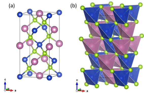
FIG. 1: (a) CuInSe 2 conventional tetragonal cell. Blue, pink, and green indicate the Cu, In, and Se atoms, respectively. Each cation is tetrahedrally coordinated by four Se atoms. (b) Plot of the conventional tetragonal cell explicitly showing the Se tetrahedra surrounding the cations. The Se-(112) planes are those facing the origin of coordinates in the plot.
