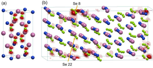
FIG. 4: (a) Probability density isosurfaces, in dark red, medium red, and light red, of the VBM state in the tetragonal unit cell of bulk CuInSe 2 (for clarity, the bonds between cations and anions are not depicted). The total probability of finding an electron in the VBM state within the volume enclosed by the dark red isosurface is 1/8. The corresponding probability is 1/4 for the medium red isosurface, and 1/2 for the light red isosurface. The probability density is equally distributed among all Se atoms, i.e., the state is delocalized. The isosurfaces also clearly reveal the predominant Se 4 p character of the VBM state. (b) Similar plot for the VBM state in the Σ3 GB supercell. It has a predominant Se 4 p character as well, but in this case the probability density is highly localized around specific Se atoms, among which Se atom 8 (see main text). Se atom 22 is also indicated for further reference.
