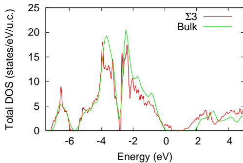
FIG. 3: Comparison of the DOS of bulk \text{CuInSe}_2 and of the \Sigma 3 (112) GB model. They are aligned so that the Cu 3d -Se 4p twin peaks and zero density in between coincide. The two curves are very close to each other, except in the gap region, where the \Sigma 3 VBM appears to be higher than in the bulk case, and the CBM appears to be lower. Energy is given with respect to the bulk VBM.
