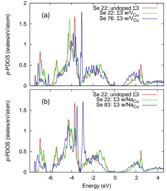
FIG. 10: (a) Comparison of the p -PDOS of Se atom 22 in the undoped \Sigma 3 supercell and Se atoms 22 and 76 (nearest neighbor to V_{Cu} ) in the \Sigma 3 supercell with V_{Cu} . (b) Comparison of the p -PDOS of Se atom 22 in the undoped \Sigma 3 supercell and Se atoms 22 and 83 (nearest neighbor to Na_{Cu} ) in the \Sigma 3 supercell with Na_{Cu} (energies referenced to the \Sigma 3 VBM).
