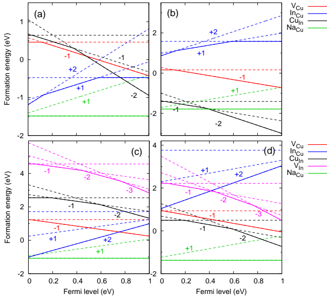
FIG. 8: Neutral and charged defect formation energies as a function of Fermi level in the CIS \Sigma 3 supercell [(a) and (b)] and in bulk CIS [(c) and (d)]. Figures (a) and (c) correspond to In-rich growth conditions and figures (b) and (d) to In-poor conditions. The continuous solid lines indicate the preferred charge state as a function of Fermi level energy.
