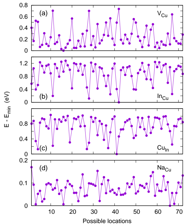
FIG. 7: Plot of the total energies of the defect-containing \Sigma 3 GB supercells vs. position of the defect, for all four point defects considered in this study.
