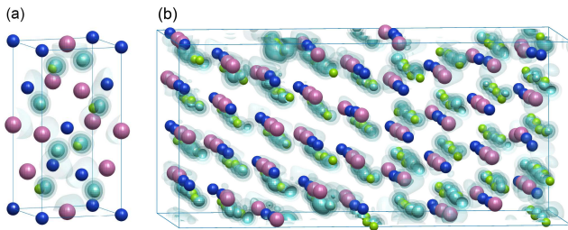
FIG. 6: Probability density isosurfaces, in dark cyan, medium cyan, and light cyan, of the CBM state in (a) bulk CuInSe 2 and (b) the \Sigma 3 GB supercell. Similar to Fig. 4, the total probabilities of finding an electron within the three isosurfaces mentioned are 1/8, 1/4, and 1/2, respectively. Both in the bulk and in the GB supercell the CBM state is predominantly of Se 4 sp character and is clearly delocalized (albeit the fact that the probability is not as uniformly distributed in the case of the GB supercell).
