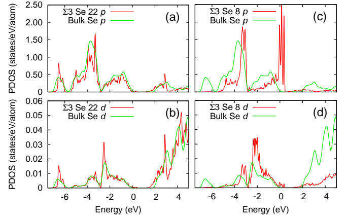
FIG. 5: Comparison of the p - and d -PDOS of a bulk CIS Se atom and of Se atoms 22 and 8 in our GB model. The energy reference is set to the bulk VBM. The plots in (a) and (b) show that Se atom 22 has essentially bulk electronic properties. In contrast, in (c), the p -PDOS of Se atom 8 presents a dramatic increase in a narrow energy range, above the bulk VBM, raising the GB VBM and effectively narrowing its band gap. In (d), the d -PDOS of Se atom 8 shows a similar, although much weaker, effect.
