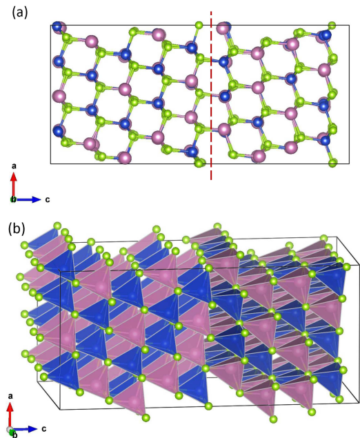
FIG. 2: (a) \text{CuInSe}_2 \Sigma 3 (112) GB 288-atom orthorhombic supercell model. The view is along the b -axis. The dashed line indicates the twin GB plane within the supercell. It is clearly a coherent GB. Because of the periodic boundary conditions, the supercell edges along the c -directions represent an analogous GB plane. (b) The tetrahedra on the right-hand side result from a rotation with respect to the tetrahedra on the left of 60^\circ around the normal to the GB plane.
