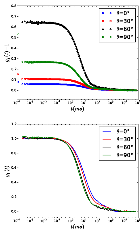
Fig. 2 Time auto correlation functions recorded during a Q_{\parallel} scan in EWDLS at \alpha_r = 60^\circ and values of \theta as indicated in the legend. Top: Intensity correlation functions g_2(t) - 1 as measured. Bottom: Field correlation functions calculated by the generalized Siegert relation, eq. 1
