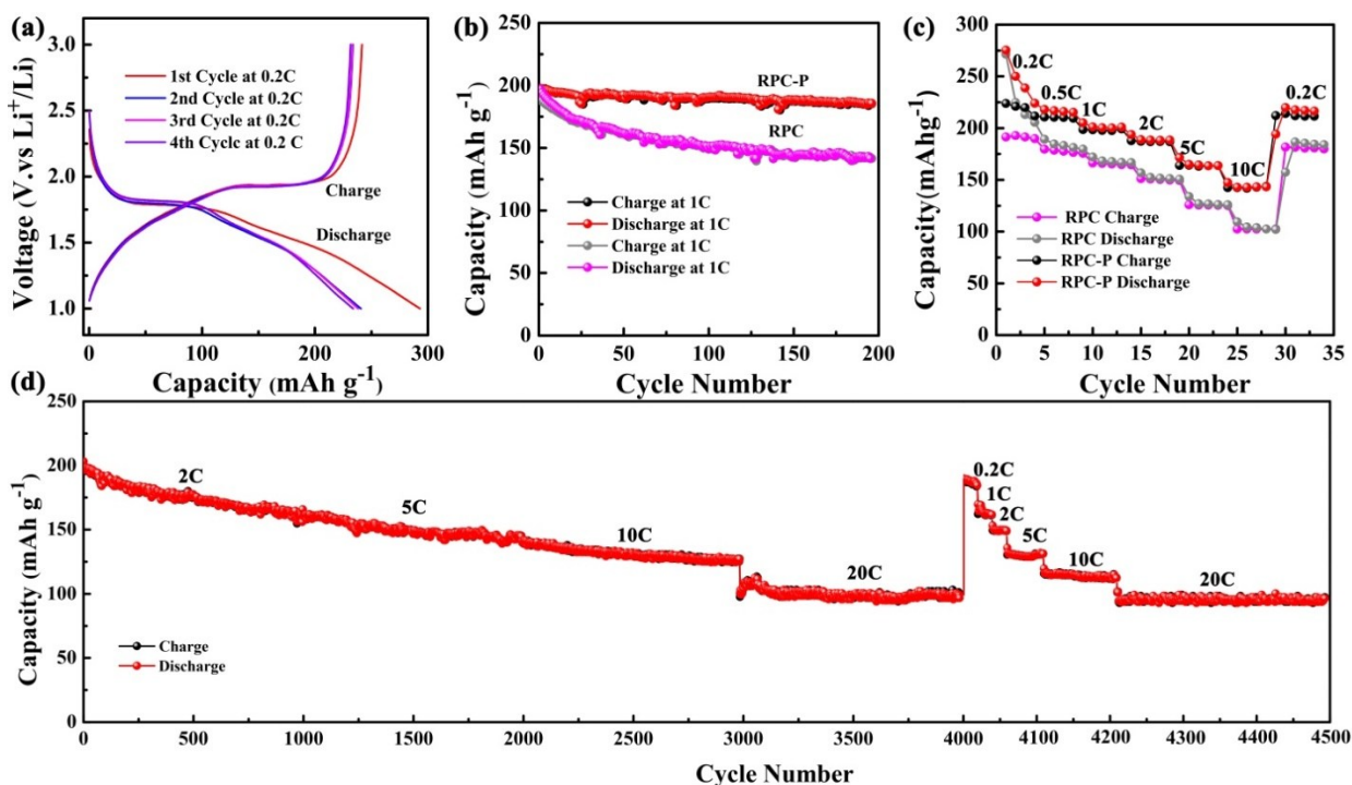
Figure 4. (a) Charge-discharge profiles of RPC-P TiO 2 at 0.2C for the first four cycles, (b) cycling performance of RPC TiO 2 and RPC-P TiO 2 electrodes at 1C for 200 cycles, (c) rate performance of RPC TiO 2 and RPC-P electrodes and (d) cycling performance of RPC-P TiO 2 at 2, 5, 10 and 20C for 1000 cycles respectively, and rate performance after cycled at 2, 5, 10 and 20C for 4000 cycles.
