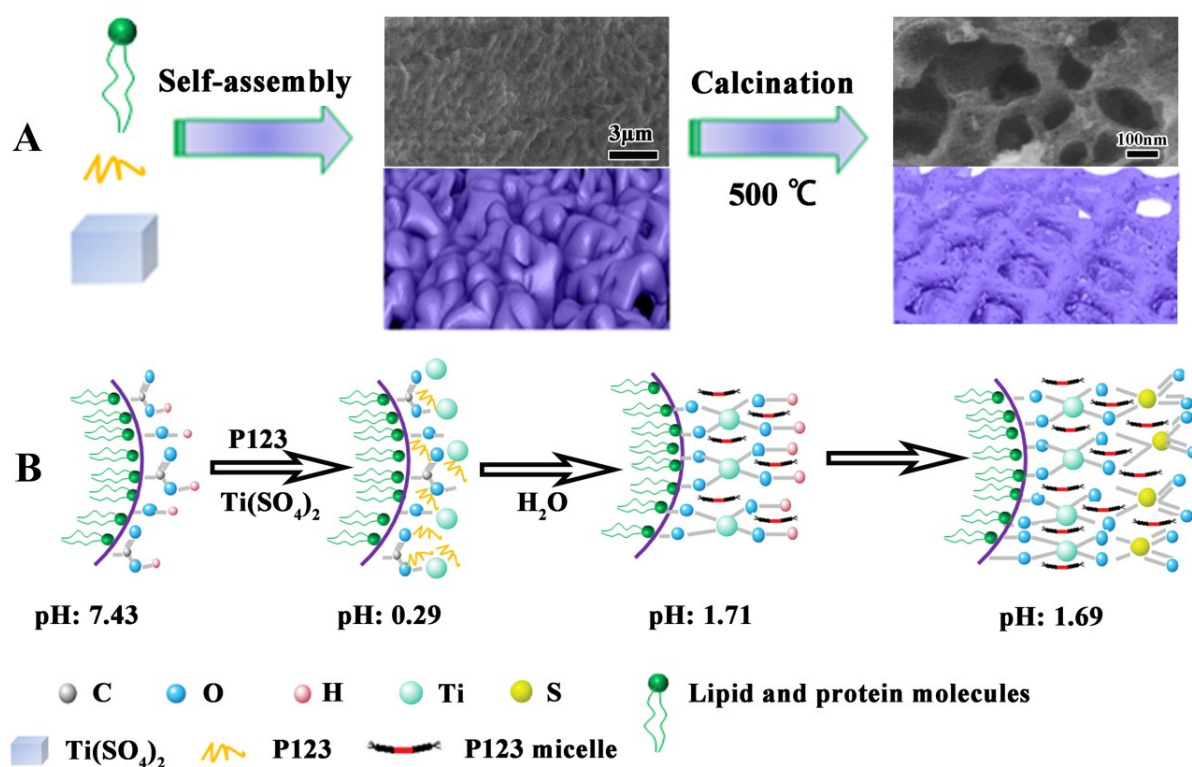
Scheme 1. A: Schematic illustration of the preparation process of RPC-P TiO 2 ; B: Schematic illustration of the self-assembly process. The grey images in A are the corresponding SEM images.
