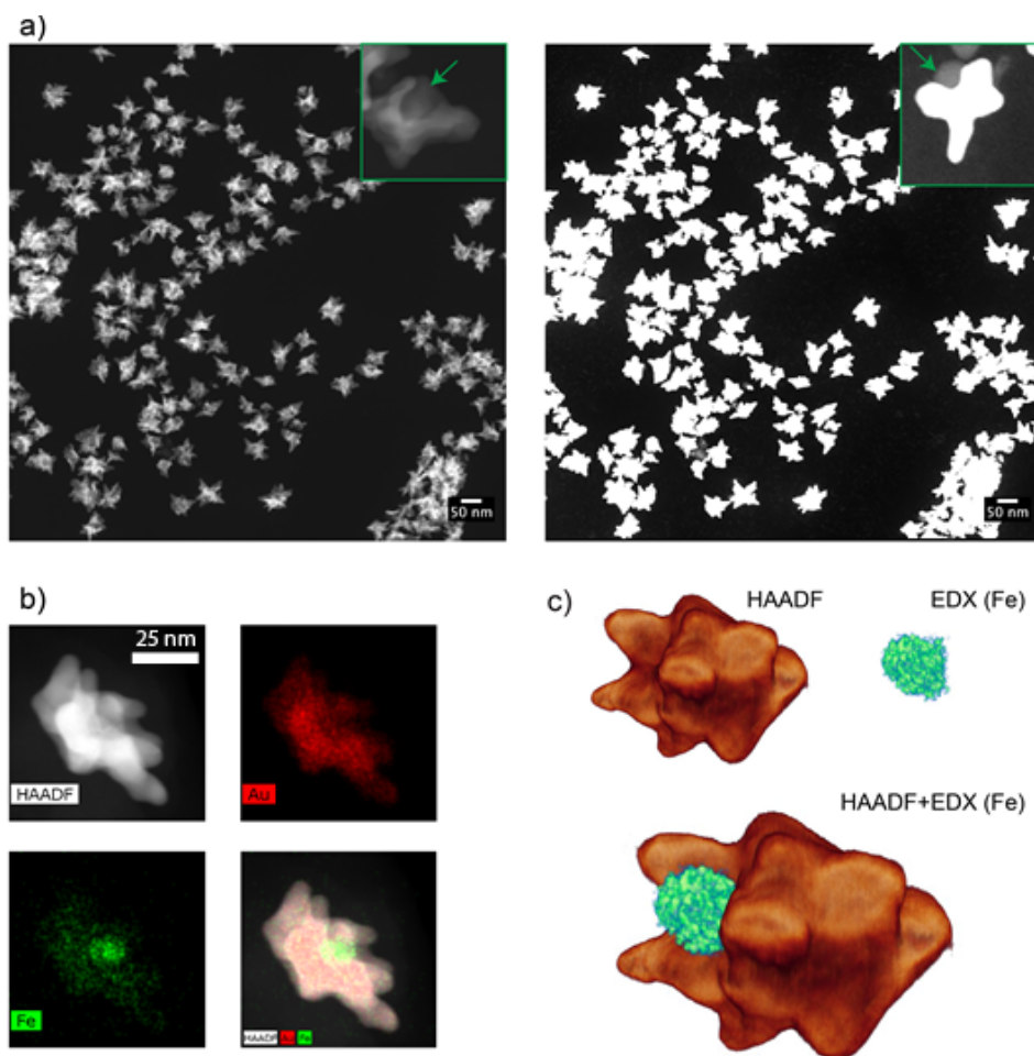
Fig. 3 a) HAADF-STEM image of JMNSs showing uniformity in size, the inset shows a nanoparticle with a cavity corresponding to the iron oxide component. The image on the right shows the same area but saturating the detector, the inset shows a nanoparticle where the iron oxide part is located at one side. b) Images of the same nanoparticle using HAADF-STEM, EDX mapping of gold atoms, EDX mapping of Fe atoms and a combination of the three. c) Tomographic reconstruction of a nanoparticle combining a HAADF-STEM tomography and EDX mapping of Fe, at different angles between -75^\circ and 75^\circ at 10^\circ intervals.
