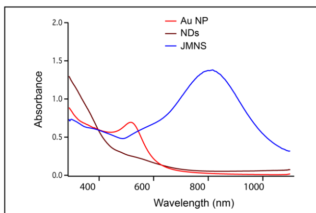
Fig 2. a) UV-Vis spectra comparing the absorbance of Au NPs (in red), NDs (in brown), and JMNS (in blue).
