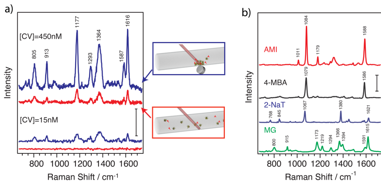
Fig. 5 a) SERS spectra of crystal violet [CV] containing JMNs in solution (red) and after magnetic concentration (blue) for two different dye concentrations [CV]=450nM (upper spectra) and [CV]= 15nM (lower spectra). Concentration of JMNs is [Au]=0.2 and 0.1 mM respectively. The spectra were shifted vertically for clarity with the scale bar corresponding to an intensity of 200 counts. b) SERS spectra of different molecules after a magnetic aggregation. AM: Acetoamidothiophenol, 4-MBA: 4-Mercaptobenzoic acid, 2NaT: 2-Naphthalenethiol, Malachite Green. Analyte concentration 4.5 mM, [Au] =0.2mM. AMI, 4-MBA and 2-NaT were measured with 785 nm excitation whereas MG was measured with 633 nm excitation wavelength. The intensity scale bar corresponds to 500 counts.
