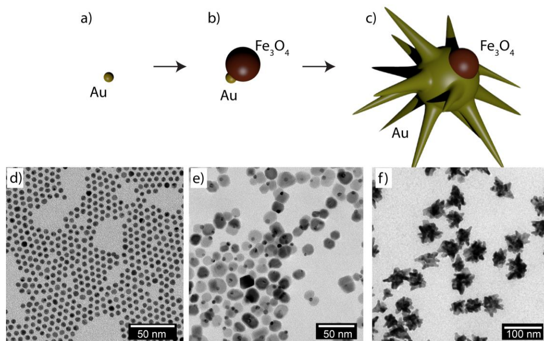
Fig 1 Scheme of the synthesis of Janus magnetic-nanostars through consecutive seed-and-growth-steps. a) Oleylamine synthesis of Au nanoparticles. b) Growth of an Iron oxide nanoparticle through the decomposition of \text{Fe}(\text{CO})_5 and subsequent oxidation. c) Growth of an Au nanostar using the Au part as seed and the PVP AuNSs synthesis method. d,e,f) TEM images of different nanoparticles corresponding to the scheme above: (d) AUNPs, (e) NDs, (f) JMNSs.
