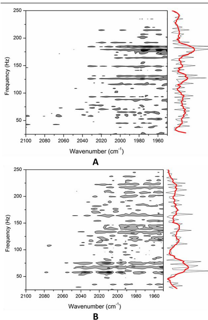
Figure 2. 2D PJAS-IR maps (at 300 °C) of CO adsorbed on Pt/ZSM-5: (A) Pt/Z-26-CIE and (B) Pt/Z-26-IWI.
