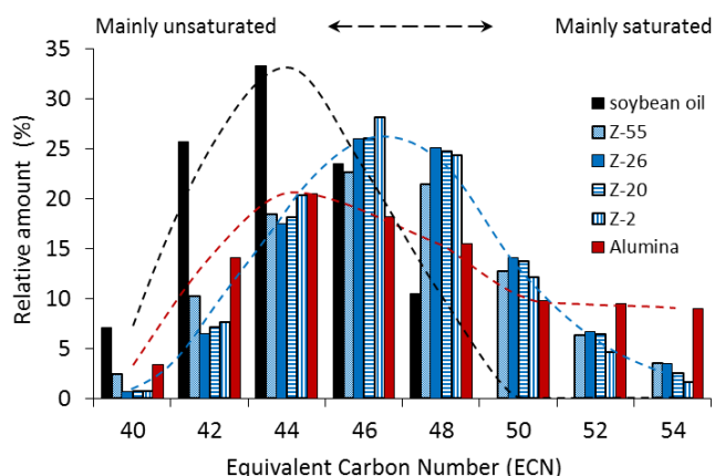
Figure 6. Triacylglycerol composition according to their equivalent carbon number (ECN) of the starting soybean oil (in black) and the fat mixtures (at IV 90) hydrogenated by different Pt catalysts. All Pt/ZSM-5 catalysts (in blue) are prepared via competitive ion-exchange, whereas Pt/alumina (in red) is prepared via incipient wetness impregnation. Lines connect the relative amount of each TAG family with certain ECN and therefore show the (shift in) TAGs distribution before (black) and after partial hydrogenation in presence of shape-selective (blue, intermediately melting fatty product) and non-selective (red, highly melting fatty product) catalysts.
