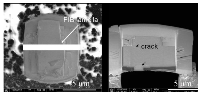
Figure 3. SEM images of (left) the large coffin-shaped Z-1 ZSM-5 crystal and (right) the FIB lamella.
