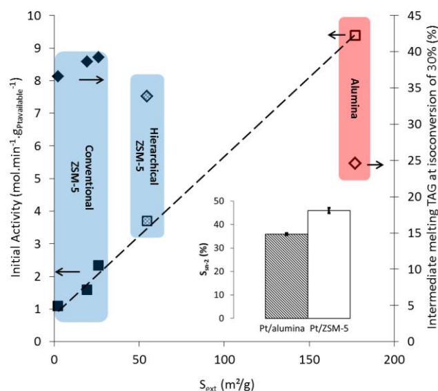
Figure 5. Influence of S_{\text{ext}} ( S_{\text{total}} in case of alumina support) of the various Pt catalysts on the initial activity (calculated as \text{mol}\cdot\text{min}^{-1}\cdot(\text{g}_{\text{Pt}}\cdot\text{D}_{\text{Pt}})^{-1} ) and the hydrogenation selectivity, here expressed as the level of intermediately melting TAGs at 30% conversion (IV 90) and the selectivity S_{\text{sn-2}} for the hydrogenation of the fatty acids located at the central sn -2 position, calculated as the conversion on sn -2 / (conversion on sn -2 + conversion on sn -1/3).100%, at a total conversion of \pm 25 mol% (IV = 100). All Pt/ZSM-5 catalysts are prepared via competitive ion exchange, whereas Pt/alumina is prepared via incipient wetness impregnation.
