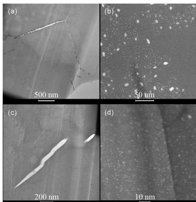
Figure 4. FIB-(S)TEM images of the Pt/Z-1-IWI sample, (a) showing Pt particles as dark spots agglomerated at interfaces and (b) the inhomogeneous distribution of small and large Pt particles as bright spots; and of the Pt/Z-1-CIE sample, (c) showing few Pt particles as dark spots and (d) homogeneously distributed small Pt particles as bright spots.
