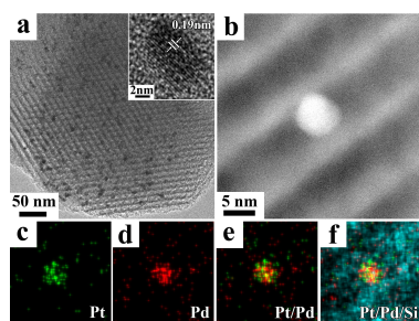
Fig. 1 (a) TEM image and (b) high magnification HAADF-STEM image of PtPd/SBA-15; (c–f) corresponding EDX elemental mapping results: (c) Pt, (d) Pd, (e) Pt and Pd, and (f) Pt, Pd and Si overlaid color mapping.
