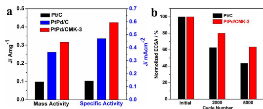
Fig. 4 (a) Mass activity and specific activity at 0.9 V versus RHE for commercial Pt/C, PtPd/C and PtPd/CMK-3. (b) Loss of ECSA of commercial Pt/C and PtPd/CMK-3 after potential sweep cycles.
