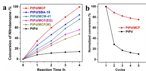
Fig. 3 (a) The time-domain conversion of nitrobenzene by different PtPd catalysts. (b) A comparison of conversion for PtPd/MCF and PtPd during the five reaction cycles. The reaction time is 4 h.
