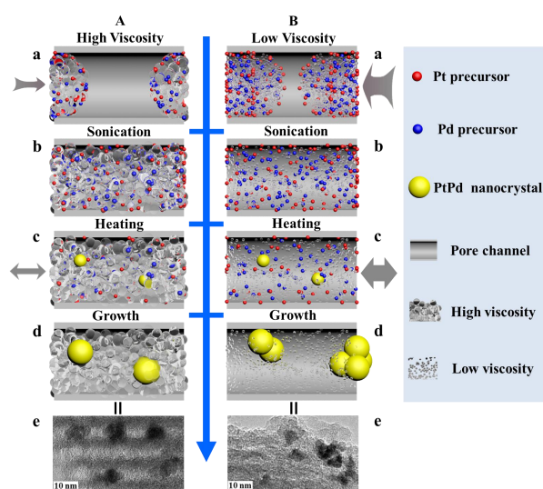
Fig. 2 Schematic illustration of the proposed formation mechanisms of nanometals synthesized in (A) high viscosity solvent and (B) low viscosity solvent: Diffusion amounts and rates of metal precursors in different viscosity solvents (Aa and Ba); Full impregnation of the reaction solution after sonication (Ab and Bb); Forming of metal nanoclusters after heating (Ac and Bc); growth, dispersion (Ad) and aggregation (Bd) of nanocrystals and corresponding TEM images of PtPd/SBA-15 (Ae and Be). Arrows indicate directions and rates of mass exchange.
