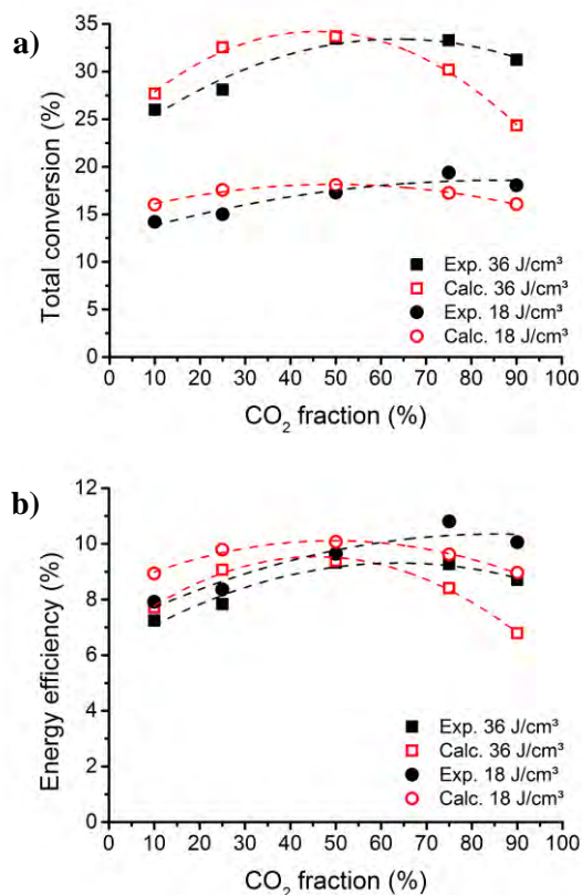
Figure 1. Calculated and experimental total conversion (a) and energy efficiency (b) as a function of CO 2 fraction, for a SEI of 18 and 36 J/cm 3 .
