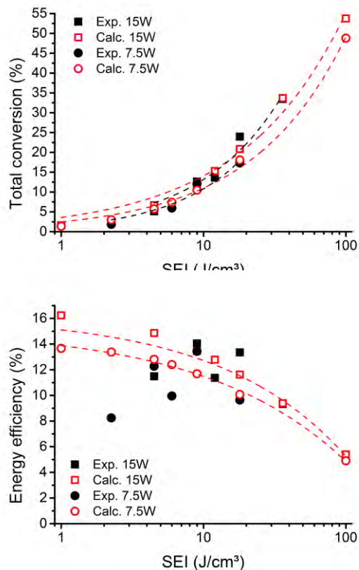
Figure 3. Calculated and experimental total conversion (a) and energy efficiency (b) as a function of SEI, for a 50-50 CH 4 -CO 2 mixture, and a plasma power of 7.5 and 15 W.
