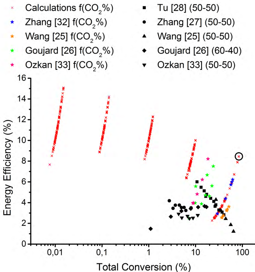
Figure 6 Comparison between our calculated values of energy efficiency vs total conversion, for all conditions investigated, with experimental data (obtained for different SEI or as function of CO 2 fraction) collected from literature, as indicated in the legend.
