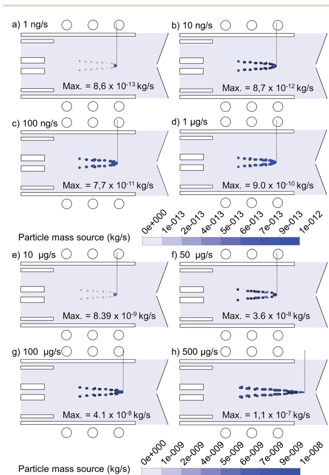
Fig. 7 Effect of mass loading flow rate on the 2D mass transfer rate of 1 \mu\text{m} copper droplets to the gas phase, introduced from the whole 1.5 \text{ mm} width of the central inlet, with flow rate of (a) 1 \text{ ng s}^{-1} , (b) 10 \text{ ng s}^{-1} , (c) 100 \text{ ng s}^{-1} , (d) 1 \mu\text{g s}^{-1} , (e) 10 \mu\text{g s}^{-1} , (f) 50 \mu\text{g s}^{-1} , (g) 100 \mu\text{g s}^{-1} and (h) 500 \mu\text{g s}^{-1} . For each case, the exact value of the maximum mass transfer rate is also indicated, for clarity.
