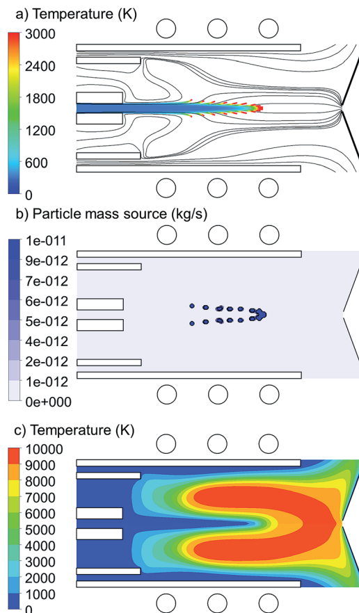
Fig. 1 General properties of copper droplet introduction, with diameter of 1 μm and flow rate of 100 ng s -1 injected from the whole width of the central inlet: (a) 2D trajectories of injected copper droplets, colored according to temperature, as well as the Ar gas flow path lines originating from the central, intermediate and outer inlets, colored in black, (b) 2D mass transfer rate of copper droplets to the gas phase and (c) 2D plasma temperature profile. The applied power is 1000 W. The carrier gas, auxiliary gas and cooling gas flow rates are 1.0, 0.4 and 12 L min -1 , respectively. The injector inlet diameter and sampler orifice diameter are 1.5 mm and 1.0 mm, respectively.
