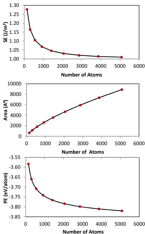
Figure 1 - Calculated surface energies (top panel), surface area (middle panel) and the potential energy per atom (bottom panel) for icosahedral clusters as a function of size.
