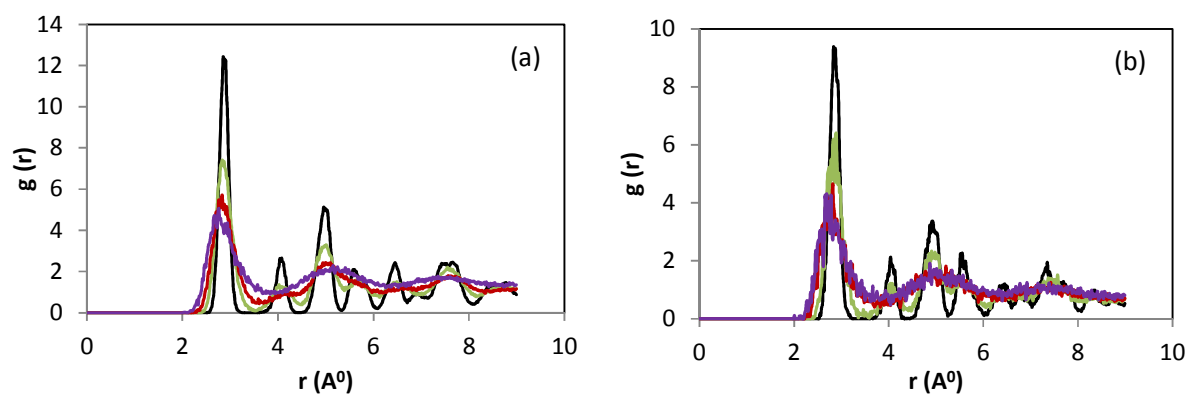
Figure 6 – The radial distribution function of the icosahedral clusters \text{Au}_{3871} (a) and \text{Au}_{561} (b) at 100 (black), 500 (green), 900 (red) and 1300 K (purple).
