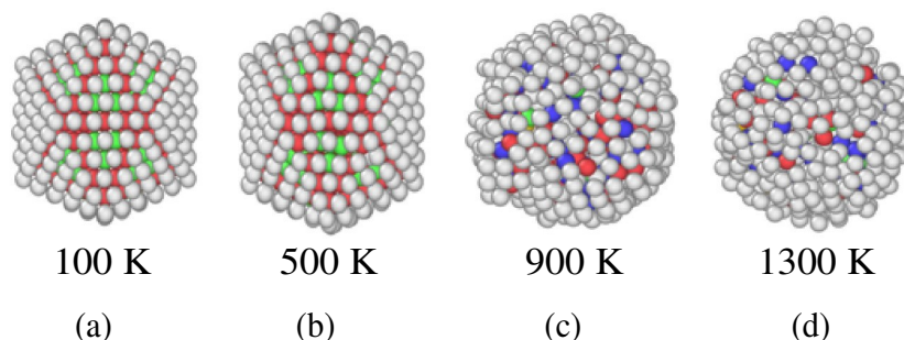
Figure 4 - Icosahedral structure of \text{Au}_{561} cluster at (a) T=100 K (b) T=500 K (c) T=900 K (d) T=1300 K. Green, red and blue represent fcc, hcp and amorphous core, respectively, while white shows other undefined coordinations.
