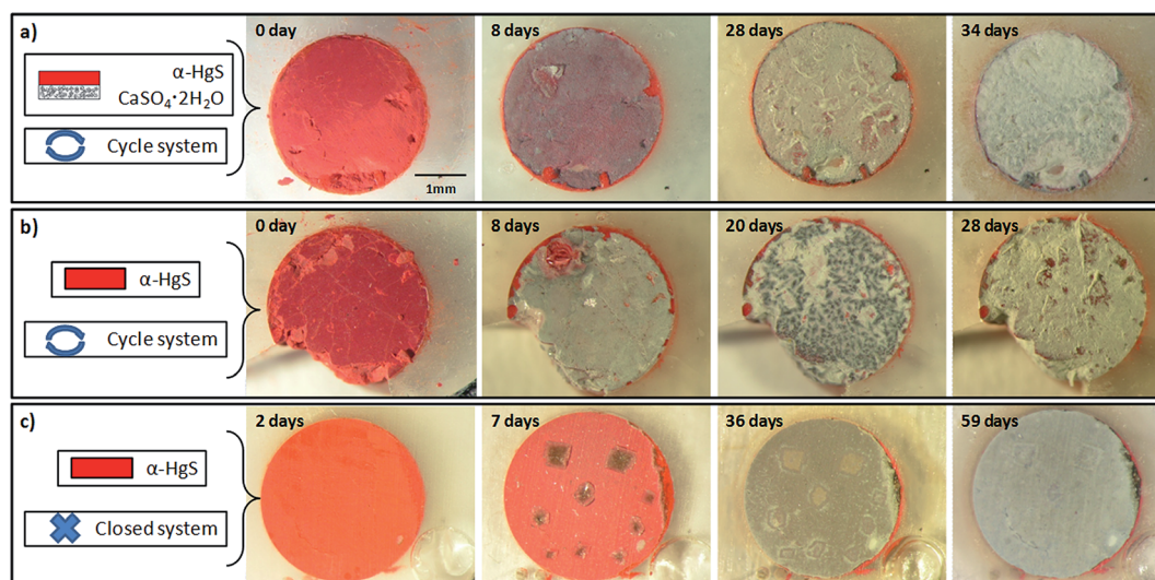
Fig. 7 Pellets aged with NaOCl solution and light at different times of ageing: (a) two-layered pellet of gypsum/vermilion in cycle system; (b) pellet of vermilion in cycle system; (c) pellet of vermilion in closed system.
