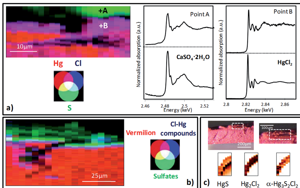
Fig. 9 Images and spectra of 3 cross-sections of different pellets aged with a NaOCl solution and light in a closed system: (a) elemental maps obtained by \mu -XRF at 2.9 keV on a two-layered calcite/HgS pellet showing in purple a layer containing Hg and Cl and in green a layer with sulfur on top of the sample (sulfates), both presences being confirmed by XANES spectra performed on the points A (S K-edge) and B (Cl K-edge) compared to corresponding references; (b) chemical maps obtained by combined \mu -XRF/ \mu -XANES on a two-layered NaCl/HgS pellet showing an intermediate layer of Cl–Hg compound; (c) phase maps obtained by \mu -XRD performed on the dashed rectangle represented on the visible picture of the HgS pellet, showing the co-localization of the two degradation compounds (the distortion of the maps is due to technical problems during the experiment).
