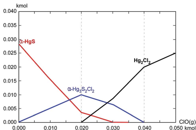
Fig. 5 Thermodynamic simulation of reactions occurring when adding \text{ClO}_{(\text{g})} to \alpha\text{-HgS}_{(\text{s})} at 25 °C.
