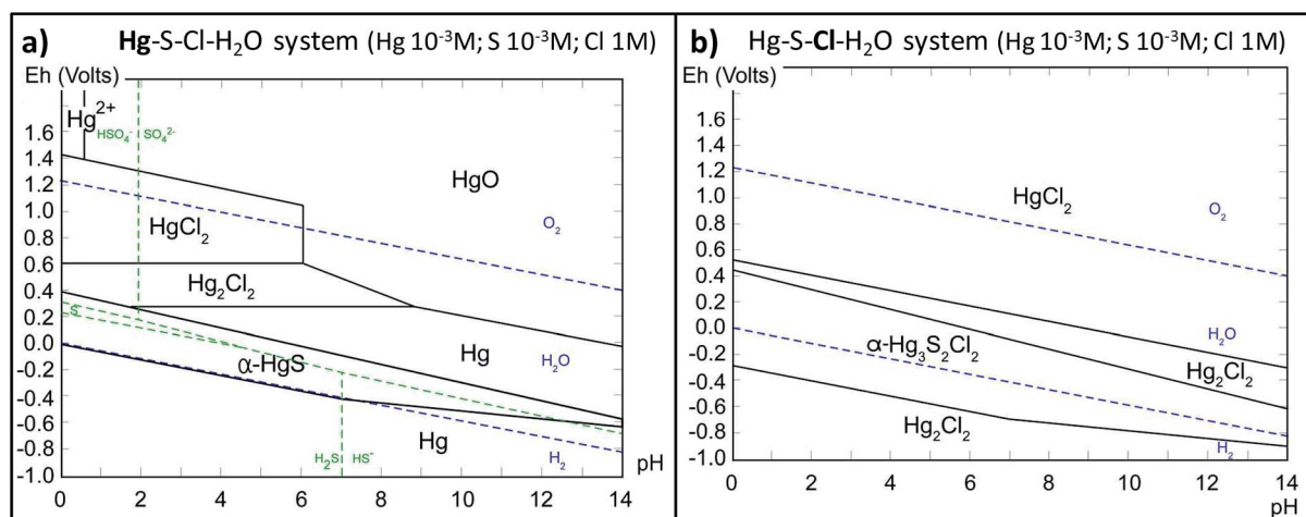
Fig. 4 Potential-pH diagrams at 25 °C for the Hg-Cl-S-H 2 O system with in bold predominant species and in brackets activities of corresponding elements.
