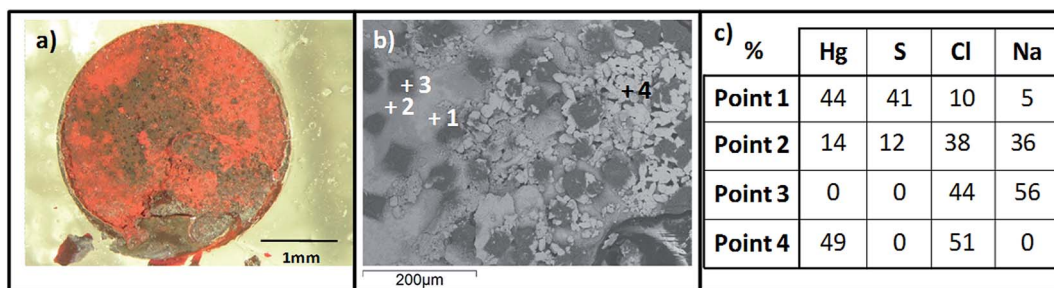
Fig. 8 Two-layered NaCl/vermilion pellet aged with NaOCl solution and light in a closed system: (a) visible image of the pellet; (b) BSE image of a part of the surface, obtained by SEM; (c) results of quantitative SEM analyses performed on the four points shown in (b) (in atomic percentage; Hg, S, Cl and Na concentrations were normalized to a total of 100%; C, O and Al datas not shown here).
