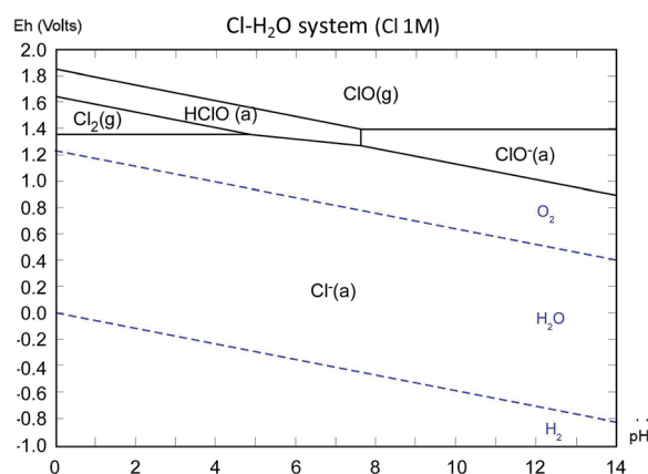
Fig. 2 Potential-pH diagram at 25 °C for Cl-H 2 O system with in brackets activity of chlorine.
