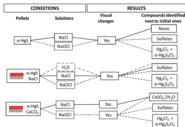
Fig. 6 Summary of some of the ageing experiments performed on pellets (without any binder) in front of light and showing modifications in the visual aspect of the pellets or/and appearance of new compounds at the surface identified by XRD or \mu\text{-XANES} .
