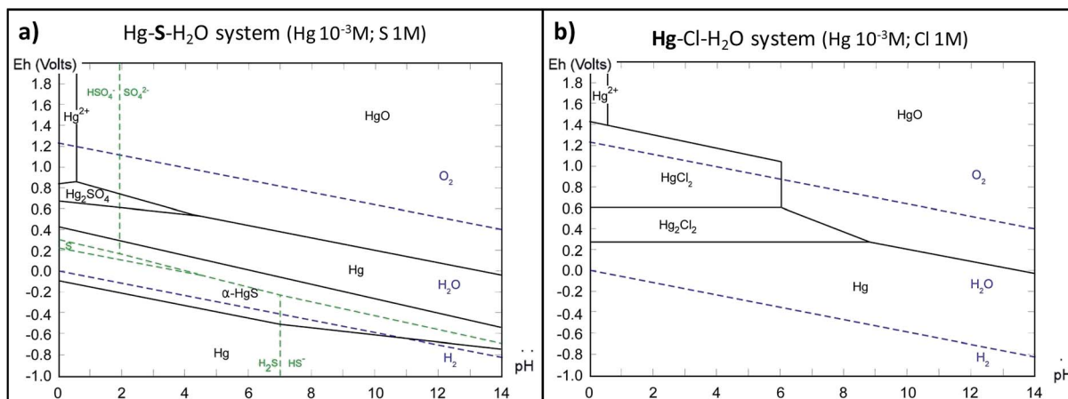
Fig. 3 Potential-pH diagrams at 25 °C for different systems with in bold the predominant species and between brackets the activities of corresponding elements.
