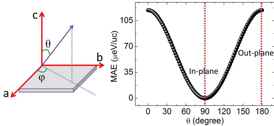
Figure S12 | DFT based tight binding calculation of MAE of single unit cell LSMO slab.
