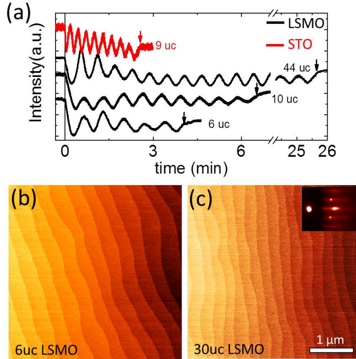
Figure S1 | Growth and characterization of LSMO and STO films. a, RHEED intensity oscillations during the growth of LSMO (6, 10, 44 uc) and STO (9 uc). The growth started at t = 0 and stopped at the time indicated by arrows. AFM images of 6 uc (b) and 30 uc (c) LSMO layers.
