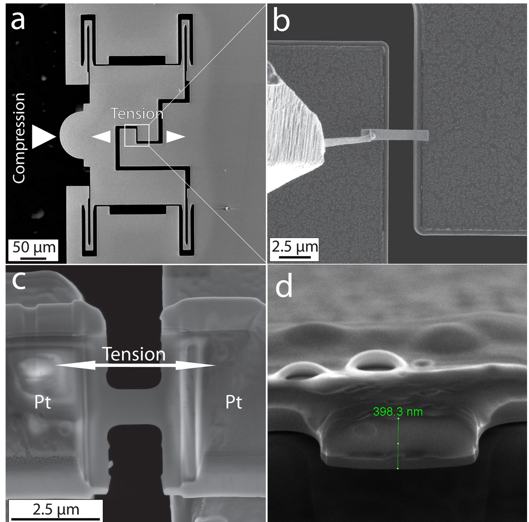
Figure 1. In situ TEM nanomechanical testing (a) optical image of the PTP device used for quantitative in situ TEM tensile experiments. The compression, with the diamond flat punch indenter, of the semicircular end on the left opens the middle gap shown in (b) and (c), inducing uniaxial tension in the test specimen; (b) scanning electron microscope (SEM) image showing the transfer of a FIB-prepared specimen onto the PTP device; (c) SEM image showing the specimen mounted in the middle gap using electron beam-deposited platinum (Pt); (d) SEM measurements of the cross-sectional area of the tensile test specimen after fracture. Two antigorite samples (Ant624-10 and AntCu65) have been used to prepare the in situ TEM specimens; see section 2 for more details.
