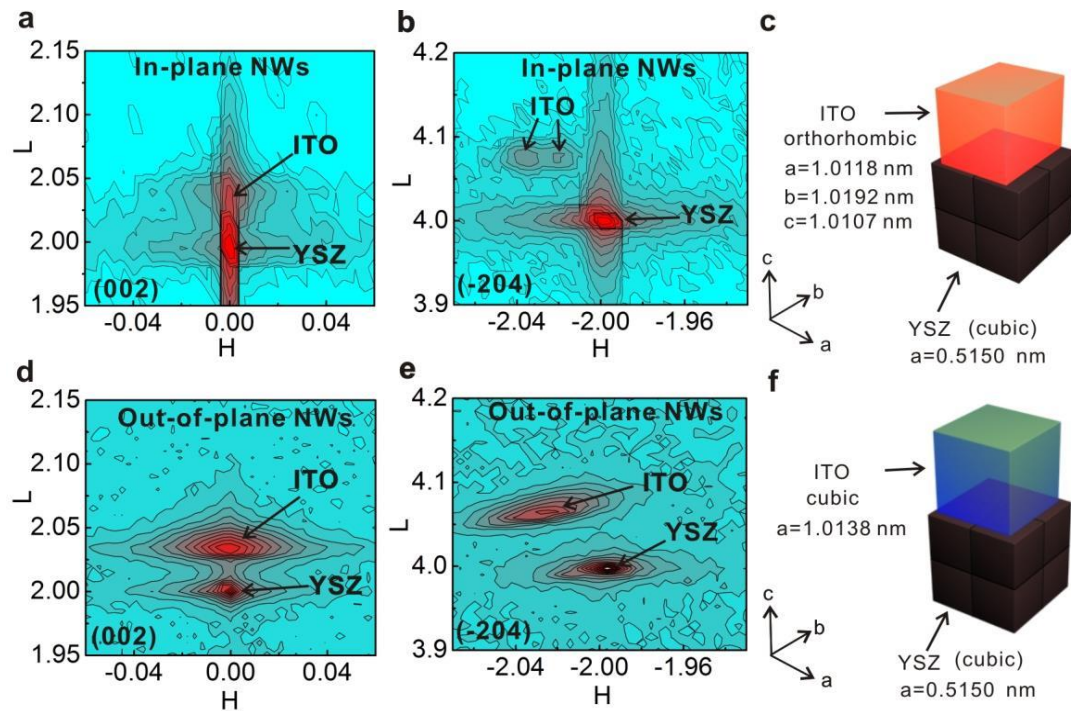
Figure 4. Reciprocal space maps of planar and vertical ITO NWs. (a-b) (002) HL and (-204) HL reciprocal space mapping data of the planar ITO NWs grown on the (100) YSZ substrate. KL mapping data (not shown) are similar with the same distribution of diffraction intensities. (c) Schematic illustration of the deformed orthorhombic ITO unit cell on the cubic YSZ. For clarity, the structural deformation is exaggerated. For ITO NWs, there are two equivalent variants of deformation with orthogonal orientations. (d-e) (002) HL and (-204) HL reciprocal space mapping data of the vertical ITO NWs grown on the (100) YSZ substrate. (f) Schematic illustration of the cubic structured ITO unit cell on the cubic YSZ substrate. The lattice constants for both planar and vertical ITO NWs were calculated from the coordinates of their diffraction peaks in the reciprocal space mapping data with the YSZ substrate as the reference.
