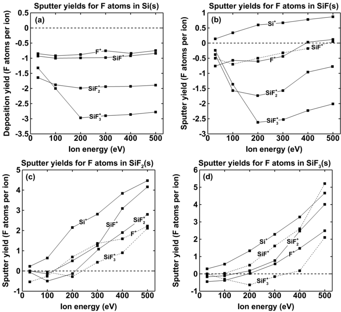
Figure 2. Calculated sputter yields of F atoms by various impinging ions on Si:100 (a), SiF (s) (b), SiF 2(s) (c) and SiF 3(s) (d). A negative sputter yield corresponds to atom deposition, where the ion impacts did not result in removal of atoms from the surface but in a net incorporation of atoms into the top surface layers. No significant difference was found between the sputter yields obtained at 300 K and 173 K. SiF 4 + and F 2 + are not considered as their density in the plasma are close to zero and thus have insignificant fluxes.
