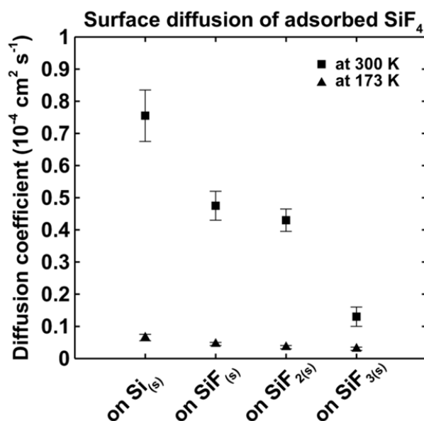
Figure 5. Calculated diffusion coefficients for physisorbed \text{SiF}_4 on different \text{SiF}_x surfaces, obtained at 173 K and 300 K.
