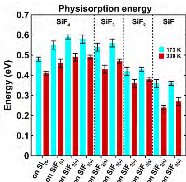
Figure 4. Calculated energy for desorption (i.e., physisorption energy) of physisorbed SiF 1-4 on different surfaces, obtained for 173 K and 300 K. Not all combinations could be obtained as explained in detail in the text.
