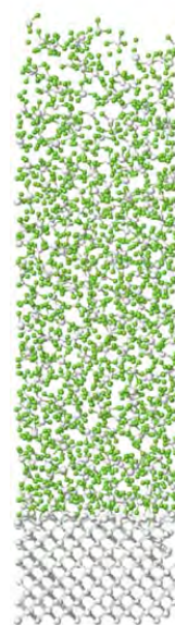
Figure 6. Illustration of an accumulated layer of physisorbed \text{SiF}_4 molecules on a \text{Si}(100) surface at 173 K. There are no chemical bonds between the \text{SiF}_4 molecules (i.e. no network). The layer is kept together only by weak dispersion forces and its height fluctuates strongly.
