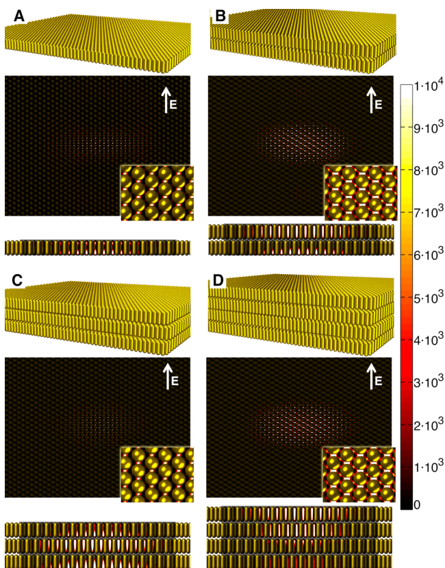
Figure 3. Simulation of hotspot distribution within supercrystals. (A–D) SERS performance (calculated as |E(633 \text{ nm})|^4 ) of GNR supercrystals with different number of layers, simulated by MLMFA-MoM. In each case, the hotspot distribution is represented both as top view and cross section: (A) monolayer; (B) bilayer; (C) trilayer; (D) tetralayer. Arrows on top view images indicate in-plane polarization direction.
