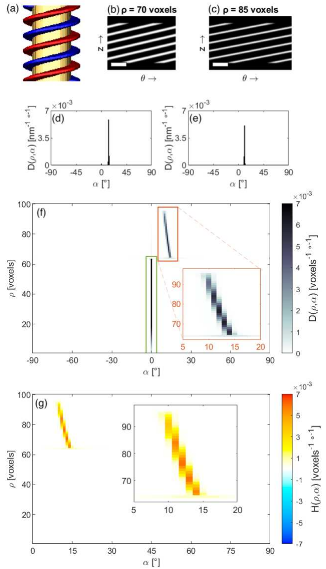
Figure 2. A simulated helix (a) with two of its cylindrical sections at \rho = 70 voxels (b) and \rho = 85 voxels (c), the scalebars are 100 voxels wide. The model consists of an achiral core (yellow) enveloped by two helices (blue and red). The directionality for the two cylindrical sections is shown in (d) and (e) respectively, and the directionality of all cylindrical sections is combined in a histogram (f), to obtain the directionality of the 3D helix in cylindrical coordinates. Two main features in (f) are marked by green and orange boxes, and the orange region is enlarged in the inset. (g) Helicity function H(\rho, \alpha) histogram and zoomed view (inset) of the peak corresponding to the helical shell of the model. Note that the line is not vertical due to the different angles involved in the model helix.
