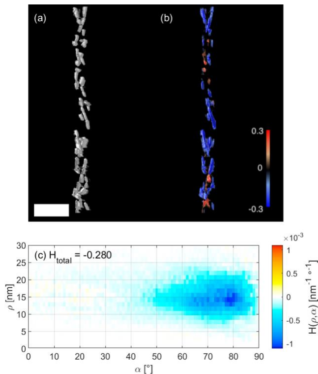
Figure 5. Quantitative analysis of the helicity of a helical arrangement of Au NRs around an amyloid fibril. An isosurface rendering of the NRs is shown in (a), the helicity map is shown in (b) as a semi-transparent 3D color-coded volume rendering, where red indicates right-handed helicity and blue indicates left-handed helicity, the window size was chosen to encompass each individual NR. The helicity function H(\rho, \alpha) and total helicity H_{total} are given in (c). The scale bar is 100 nm.
