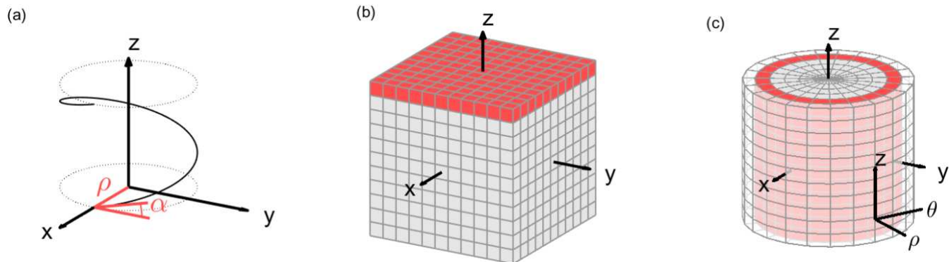
Figure 1. Illustration of the base geometries used in our method: (a) a helix around the z-axis with radius \rho and inclination angle \alpha ; (b) a discrete voxel grid in Cartesian coordinates, where each cube is a voxel; and (c) a discrete voxel grid in cylindrical coordinates, where the voxels are no longer cubes, but trapezoidal prisms. An orthoslice at constant z and a cylindrical section at constant \rho are highlighted in red in (b) and (c), respectively.
