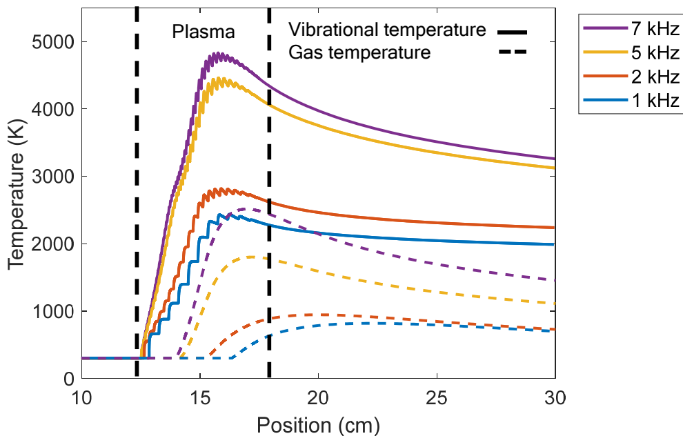
Figure 7: Calculated vibrational and gas temperature as a function of position, in a pulsed MW plasma of 50 \mu\text{s} pulse width, for four different pulse frequencies. The plasma length, which is equal to the width of the waveguide (cf. figure 1), is 5 cm, and is indicated by the vertical dashed lines.
