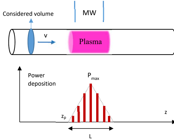
Figure 2: Schematic overview of the setup and power deposition profile used in the 0D (or quasi-1D) model. The plasma is formed between position z_p and position z_p + L . P_{max} is the maximum applied power at the center of the plasma.
