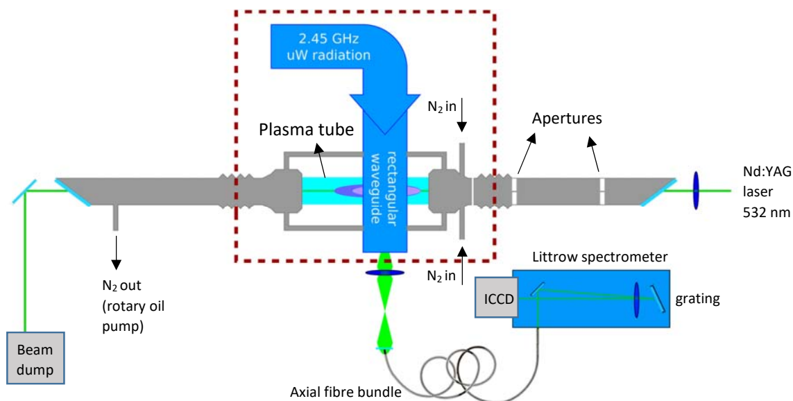
Figure 1: Schematic overview of the Raman scattering setup, installed at the MW setup (highlighted by the dashed red contour).
