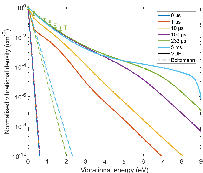
Figure 4: Calculated VDFs at five different times during the 233 \mu s pulse (0 – 233 \mu s) and in the afterglow (5 ms) (solid lines), as well as the Boltzmann distribution functions at the corresponding gas temperature (dashed lines), to indicate the strong degree of vibrational non-equilibrium. In addition, the measured VDF of the first eight vibrational energy levels at 233 \mu s is also shown (green data points)
