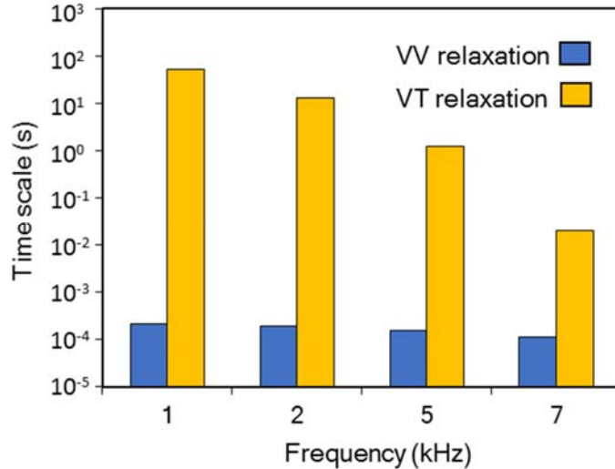
Figure 9: Time scale of VV and VT relaxation for 50 μs pulses at four different pulse frequencies at the experimental conditions (25 mbar), calculated using equations 15 and 16 above.
