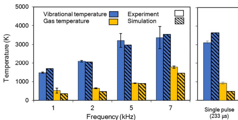
Figure 6: Measured and calculated vibrational and gas temperatures in the center (radial direction) of the plasma, spatially- and time-averaged over the length of the pulse, for a pulsed MW plasma with a pulse width of 50 μs, at four different frequencies. As a reference, we also show the spatially- and time-averaged vibrational and gas temperatures for the isolated 233 μs pulse of the previous section.
