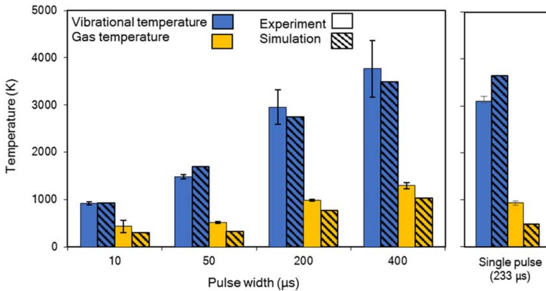
Figure 11: Measured and calculated vibrational and gas temperatures in the center (radial direction) of the plasma, spatially- and time-averaged over the length of the pulse, for a pulsed MW plasma, at four different pulse widths and a pulse repetition frequency of 1 kHz. As a reference the spatially- and time-averaged vibrational and gas temperature is shown for the isolated 233 \mu\text{s} pulse.
