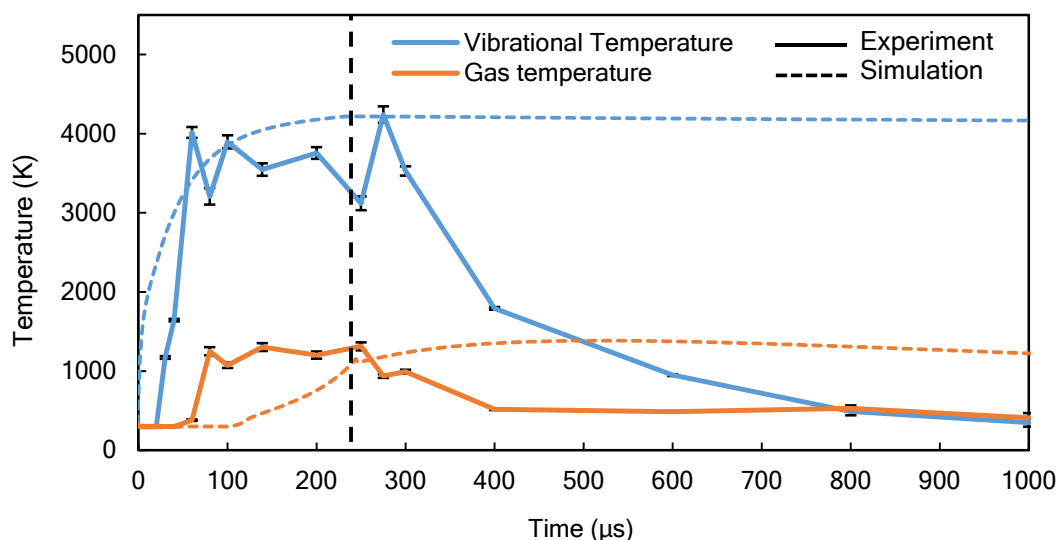
Figure 3: Time-evolution of the measured (full lines) and calculated (dashed lines) vibrational and gas temperature through a 233 \mu\text{s} pulse. The error bars of the experimental values are the errors resulting from the fitting procedure. The measured values are obtained in the center of the plasma. The end of the pulse is indicated with a vertical dashed line.
