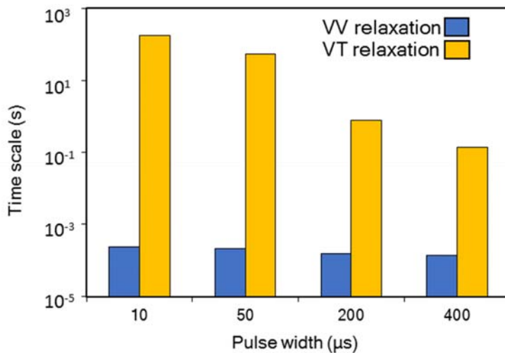
Figure 14: Time scale of VV and VT relaxation for a 1 kHz pulsed plasma at four different pulse widths, calculated using equations 15 and 16 above.
