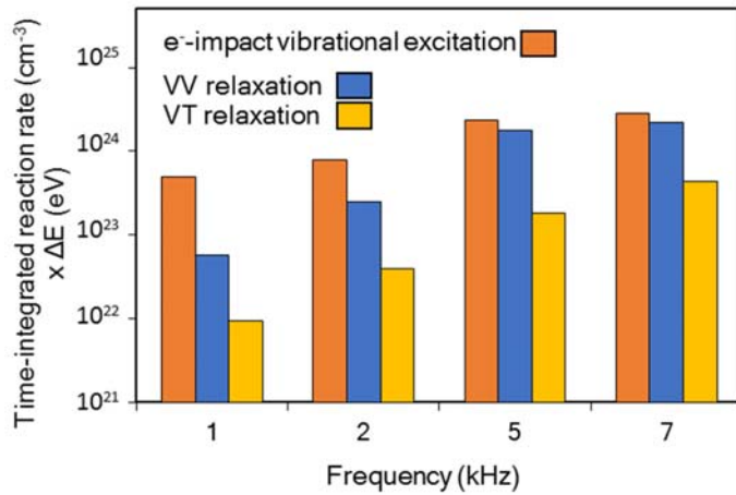
Figure 8: Time-integrated reaction rates of electron impact vibrational excitation, VV and VT relaxation, in a pulsed MW plasma with a pulse width of 50 μs, at four different frequencies, summed over all 43 vibrational levels and multiplied with the energy difference of the transitions.
