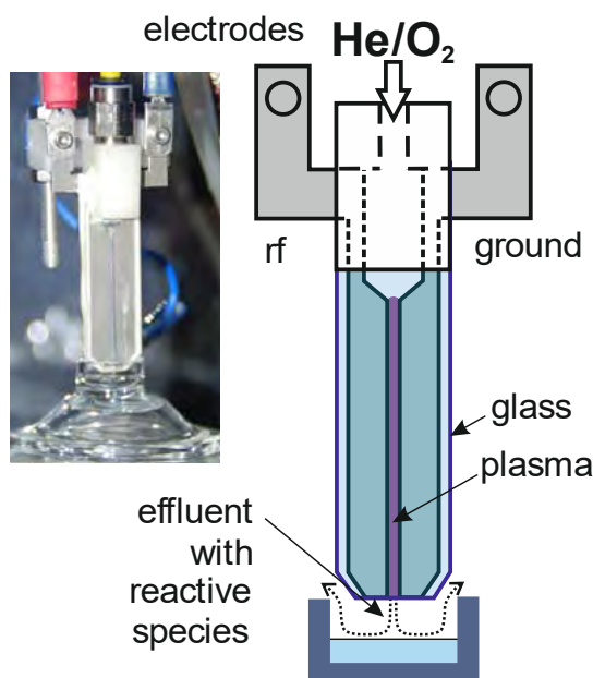
Figure 3. The photograph and a scheme of the \mu -APPJ used in the treatment of the test solutions.
