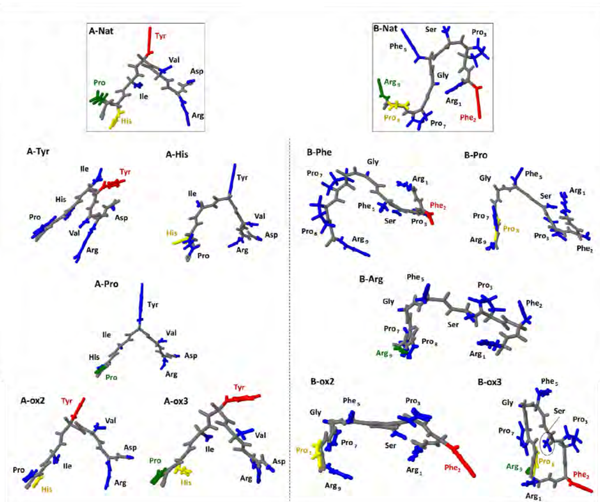
Figure 9. Representation of the average structures of the native peptides (black boxes) and their oxidized structures. On the left side the structures of peptide A are shown, on the right side the structures of peptide B. The peptide backbone is depicted in grey using a stick model in all structures. Un-oxidized side groups are depicted in blue. Red indicates the oxidation of Tyr for peptide A and Phe for peptide B. Yellow indicates the oxidation of His for peptide A and Pro for peptide B. Green indicates the oxidation of Pro for peptide A and Arg for peptide B.
