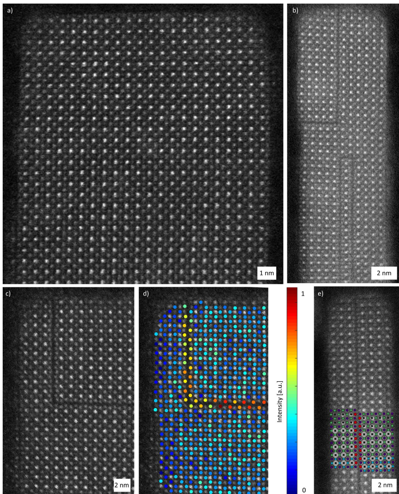
Figure 4. HAADF-STEM analysis of Cs(Cl:Br:I) 3 NCs. HAADF-STEM images of Cs(Cl:Br:I) 3 NCs, showing (a) the perovskite lattice and (b and c) NCs with several plane shifts. (d) The volume of the fitted Gaussian peaks of the halide columns of the NC as shown in (c), indicates increased intensity values of the halide columns around the RPP planes, confirming an increased concentration of iodide ions at these positions. (e) RPP plane shift model (Cs + = purple, Pb 2+ = black, Cl - /Br - = blue, I - = red, and grey corresponds
