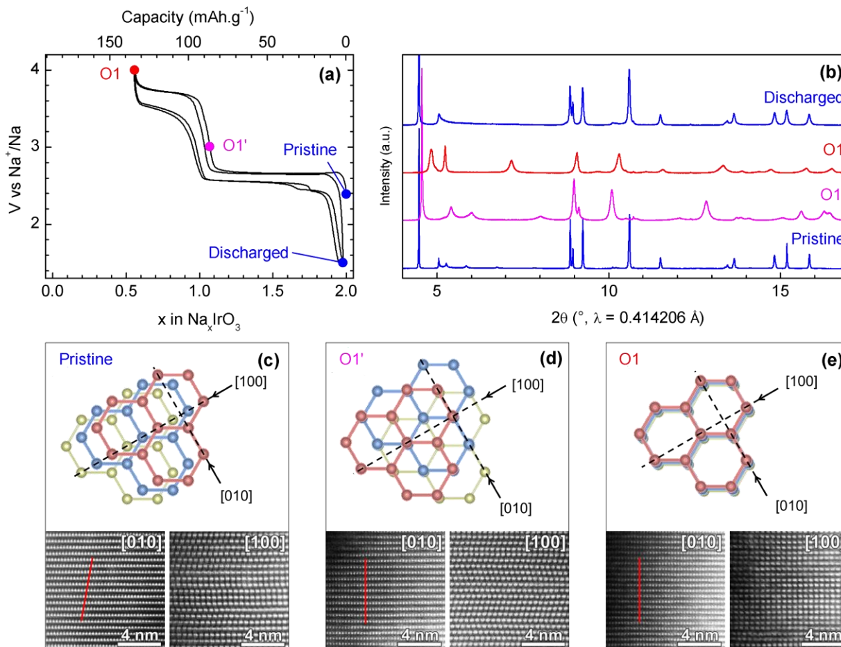
Figure 1. First and second galvanostatic cycles of Na 2 IrO 3 vs Na (a), SXRD patterns (b) and high resolution HAADF-STEM images (c-e) of samples at different states of charge. Different stackings of the transition metal layers are found and represented here. For clarity, only the Ir honeycombs are represented in the sketch, and the crystallographic directions corresponding to the TEM observations are indicated. The red lines on the HAADF-STEM images highlight the perfect cubic close-packed ABCABC (c) and hexagonal close-packed ABAB (d, e) stacking of oxygen.
