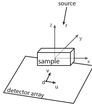
Figure 3: Scheme depicting the projection geometry of a single projection direction.
