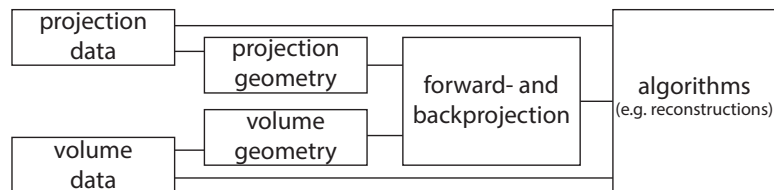
Figure 2: Schematic overview of the basic ASTRA Toolbox objects and their relations.
