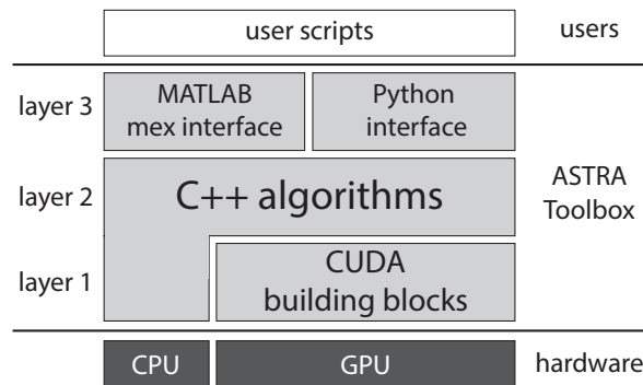
Figure 1: Schematic overview of the ASTRA Toolbox design.
