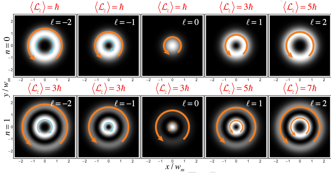
Figure 10: Same as in Figs. 5(b) and 6(b) but for the Landau states (2.33)–(2.42) with different values of (\ell, n) in a uniform magnetic field \mathbf{B} = B\bar{\mathbf{z}} [here \sigma = \text{sgn}(B) = +1 ]. Although the probability density distributions of the Landau modes is entirely similar to those of the LG beams, Fig. 6(b), their current densities and angular-momentum properties differ significantly. In particular, the kinetic OAM of Landau states, \langle \mathcal{L}_z \rangle , cannot be zero or negative even for \ell < 0 , and its minimum value is \hbar . This is because of the always-positive (for \sigma = +1 ) vector-potential contribution to the azimuthal probability current, Eqs. (2.38) and (2.39).
