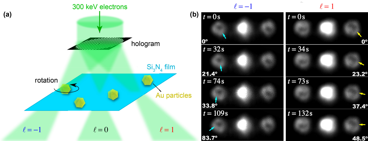
Figure 27: Angular-momentum transfer from electron vortex beams to nanoparticles [306]. (a) Schematic of the experiment. Vortex beams with different topological charges \ell , generated with a holographic mask, are focused on the sample, so that only one of the beams impinges on the selected gold nanoparticle. (b) Experimental images displaying clockwise and counter-clockwise rotations of a nanoparticle (indicated by arrows) in the \ell = -1 and \ell = 1 vortex beams.
