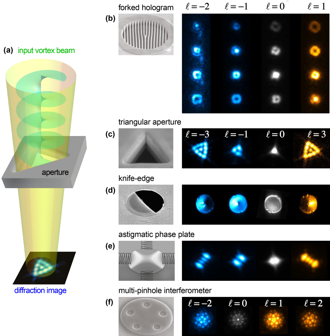
Figure 21: Diffraction-based methods for measurements of the topological charges of electron vortex beams [242, 243]. (a) Schematic diagram of the main idea. The vortex beam impinges on a specially-shaped aperture (or a phase plate) producing the far-field diffraction pattern which reveals the value of \ell . In (b–f) the patterns produced by different elements are shown, with the yellow and blue far-field images corresponding to the \ell > 0 and \ell < 0 beams. The fork hologram (b) reveals the topological charge of the beam by observing which diffraction order does not have a doughnut profile. The triangular aperture (c) yields a triangular lattice of spots where the number of spots along one side is \ell + 1 . The knife-edge aperture (d) causes a transverse deformation and shift of the beam intensity that depends on the sign and value of the OAM. The astigmatic phase plate (e) also causes a multi-lobed pattern where the number of lobes is proportional to \ell + 1 . The multi-pinhole interferometer (f) produces patterns which are related to the topological charge of the original wave function. Furthermore, the autocorrelation function of these patterns allows one to obtain an approximate OAM spectrum of the incoming wave [243].
