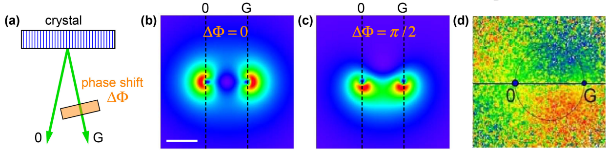
Figure 25: (a) Schematic picture of the energy loss magnetic chiral dichroism (EMCD) technique. The crystalline specimen acts as a beam splitter creating a Bragg-scattered copy of the outgoing wave in the energy-filtered diffraction pattern (b) (the rainbow color scheme is used for the intensity). Here, “G” and “0” denote the reciprocal lattice points. The waves interfere destructively in the center, independently of the excited state ( p^+ or p^- ). (c) Inducing a relative phase shift of \Delta\Phi = \pi/2 between the two waves yields an asymmetric diffraction pattern that reveals which of the two states was excited. Here it is p^+ , while the opposite transition to p^- would result in a mirrored intensity distribution with intensity shifted to the upper half-plane. The phase shift can be set by tuning the excitation error, i.e., the orientation of the reflecting lattice planes with respect to the beam. The simulations in (b) and (c) correspond to the incident electrons with energy 200 keV inducing dipole-allowed transitions, and the scale bar indicates the scattering angle of 10 mrad. (d) Experimental EMCD L_3 pattern of crystalline Fe showing the asymmetry corresponding to (c) [281].
