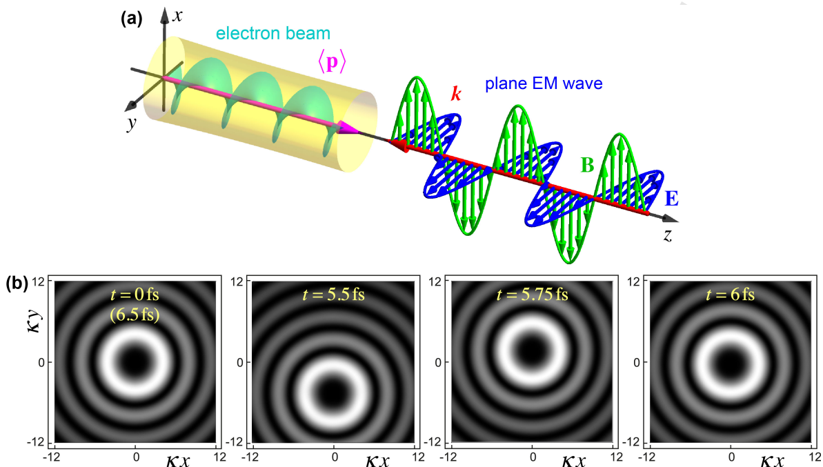
Figure 28: (a) Schematics of the Volkov–Bessel problem: a Bessel-beam solution for the Dirac electron and the field of an electromagnetic (EM) plane wave. Here the electron vortex beam and the EM wave counterpropagate with the mean electron momentum \langle \mathbf{p} \rangle and the EM wave vector \mathbf{k} . The EM wave is linearly y -polarized. (b) Temporal variations of the transverse probability-density distribution in a paraxial Volkov–Bessel beam shown in the panel (a) [109]. Here, the electron parameters are: azimuthal vortex index \ell = 3 , energy E = 300 keV, and opening angle \theta_0 = 0.02 rad. Instead of a plane EM wave, here a five-cycle laser pulse was used with the central frequency \omega_c = 10^{16} Hz and electric-field amplitude E_0 = 10^8 V/cm. The time range of 6.5 fs approximately corresponds to the duration of the pulse.
