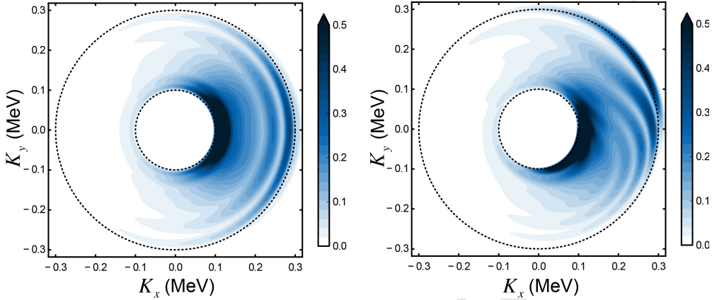
Figure 31: Differential cross-section, in arbitrary units, as a function of the total momentum \mathbf{K} = \mathbf{k}_1 + \mathbf{k}_2 , for fixed \mathbf{k}'_1 , for purely real Born-level elastic scattering amplitude (left), and for the momentum-transfer-dependent Coulomb phase (4.32) (right) [122]. The parameters used here are: E_1 = 2.1 MeV, k'_1 = 500 keV with \mathbf{k}'_1 = k'_1 \hat{x} , J_{z1} = 1/2 , J_{z2} = 13/2 , and \kappa_1 and \kappa_2 are Gaussian-distributed around the values of 200 and 100 keV with the widths 10 and 5 keV, respectively. The results are averaged over different helicities of the incoming particles. In the right-hand panel, the fine-structure constant \alpha is artificially set to 10 to enhance the visibility of the up-down asymmetry.
