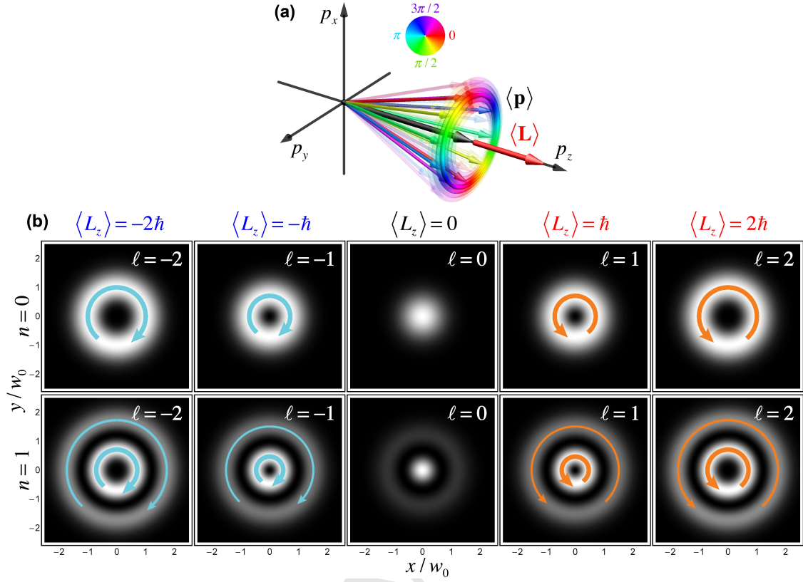
Figure 6: Same as in Fig. 5 but for the Laguerre–Gaussian (LG) beams (2.9)–(2.11) and (2.14). The transverse real-space distributions in panels (b) are shown for the beam-waist plane z = 0 . The Bessel and LG beams have similar azimuthal and OAM properties. However, the LG beams are also characterized by the momentum spectrum with radial distribution of the wave vectors (a). This provides the radial confinement of the electron, which is characterized by the additional radial quantum number n . In this manner, (n + 1) is the number of radial maxima (rings) in the intensity distribution (b).
