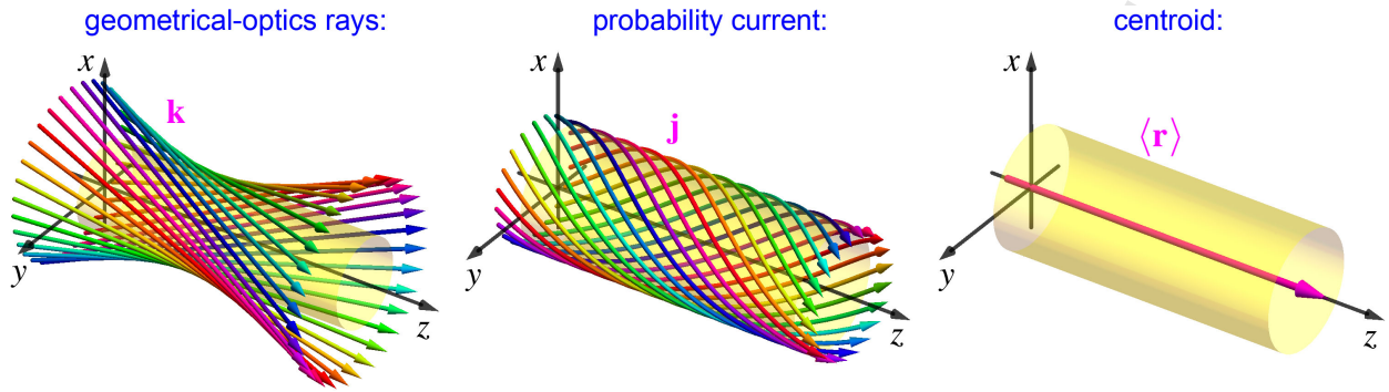
Figure 7: Geometrical-optics rays, streamlines of the probability current, and centroid trajectory in a Bessel beam with \ell = 2 (see Figs. 3 and 5). The rays form a two-parameter family of straight lines which are tangent to a cylindrical surface (here we show rays touching the cylinder at a given z and different azimuthal angles \varphi ) [70]. The directions and color-coded phases of the rays correspond to the wave vectors \mathbf{k} in the beam spectrum, Fig. 5(a). In contrast, the streamlines of the probability-current \mathbf{j} , Eqs. (2.12) and (2.13), (Bohmian trajectories) are curvilinear [68, 8]. For Bessel beams, these are spirals lying on the cylindrical surface [70]. The azimuthal component of this current generates the OAM of the beam, Eq. (2.15)–(2.17). Finally, the centroid \langle \mathbf{r} \rangle , Eq. (2.19), obviously coincides with the beam axis and corresponds to the rectilinear motion of the classical electron.
