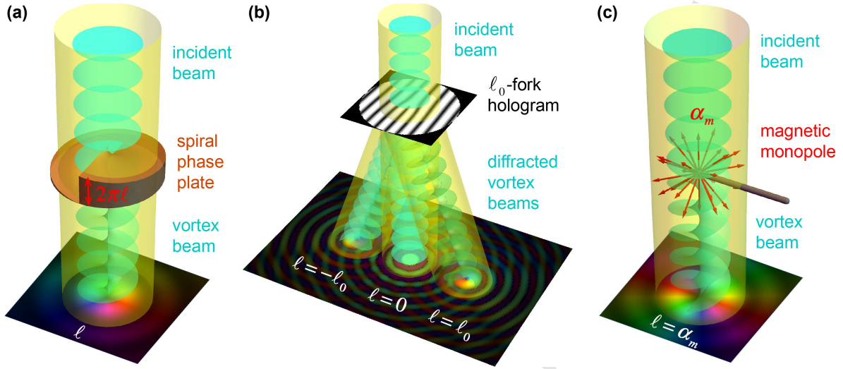
Figure 8: Schematics of basic methods for the generation of electron vortex beams: (a) a spiral phase plate with a 2\pi\ell phase-shift increment around its center (here \ell = 1 ); (b) a diffraction grating (hologram) with a fork-like edge dislocation of order \ell_0 (here \ell_0 = 1 ); and (c) a magnetic monopole of dimensionless charge \alpha_m (here \alpha_m = 2 ). See also explanations in the text.
