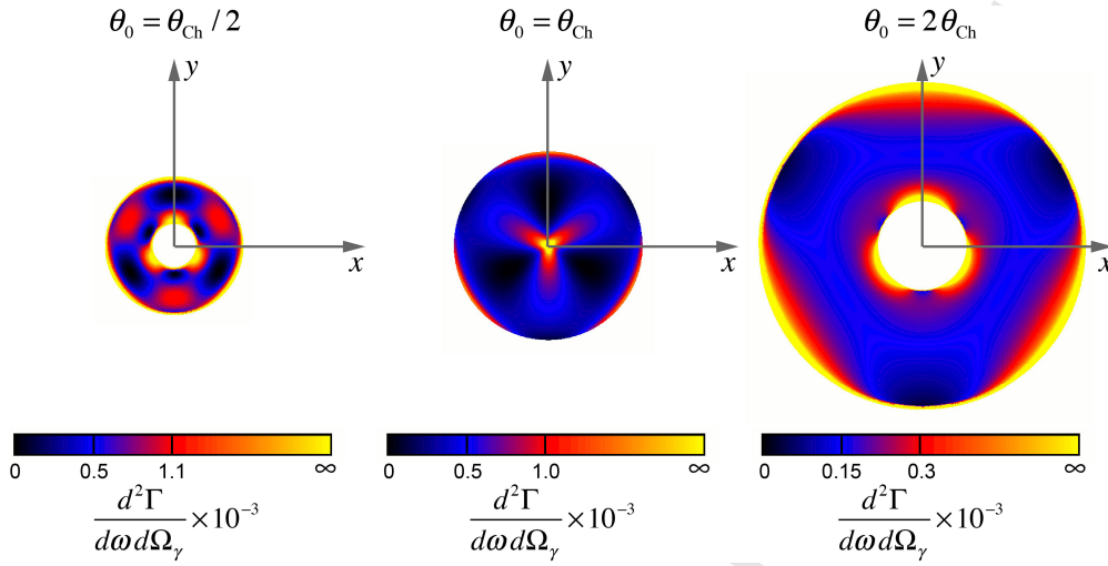
Figure 33: The spectral-angular distribution of the photon emission rate \Gamma as a function of the emitted-photon spherical angles \theta_R and \phi_R (mapped onto the (x, y) plane of the far-field detector) for an electron in a superposition of two vortex states with (J_z)_1 - (J_z)_2 = 3 and equal amplitudes [111]. The radii of the annular region of the radiation are determined by Eq. (5.3).
