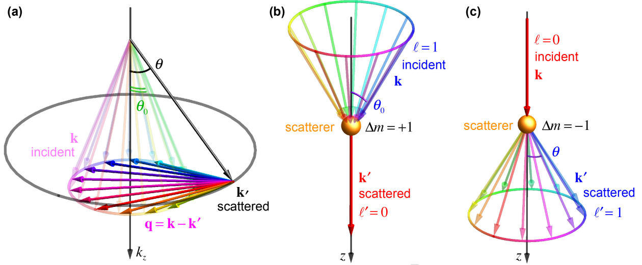
Figure 24: (a) Schematic of the electron Bessel-beam scattering by an atom into a plane wave. The incident Bessel beam consists of multiple plane waves with the \mathbf{k} -vectors conically-distributed with the polar (convergence) angle \theta_0 (shown semitransparent here). These are scattered into a single plane wave with the wave vector \mathbf{k}' (polar scattering angle \theta ). The corresponding momentum-transfer vectors are \mathbf{q} = \mathbf{k} - \mathbf{k}' . (b,c) Examples of the inelastic electron scattering accompanied by the angular-momentum exchange with the atom [274, 275]. The OAM difference between the incident and scattered electron waves, \ell - \ell' , corresponds to the change in the magnetic quantum number of the atom, \Delta m . The examples shown here correspond to the reciprocal cases of “vortex \rightarrow plane wave” (b) and “plane wave \rightarrow vortex” (c) scatterings with \theta = \theta_0 and equal probability amplitudes.
