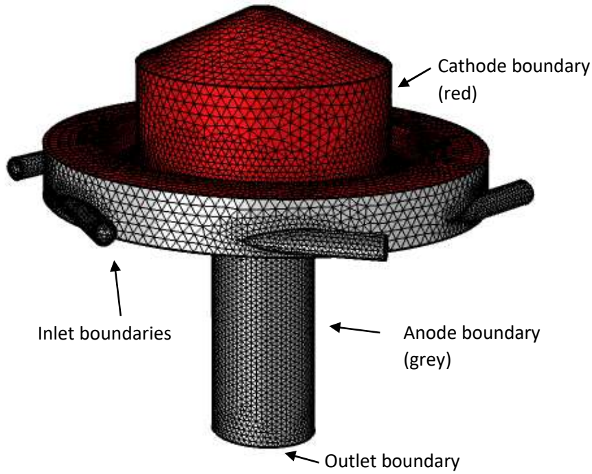
Figure 3: Computational domain of the plasma arc model. The inlets, outlet, cathode and anode boundaries are indicated.
