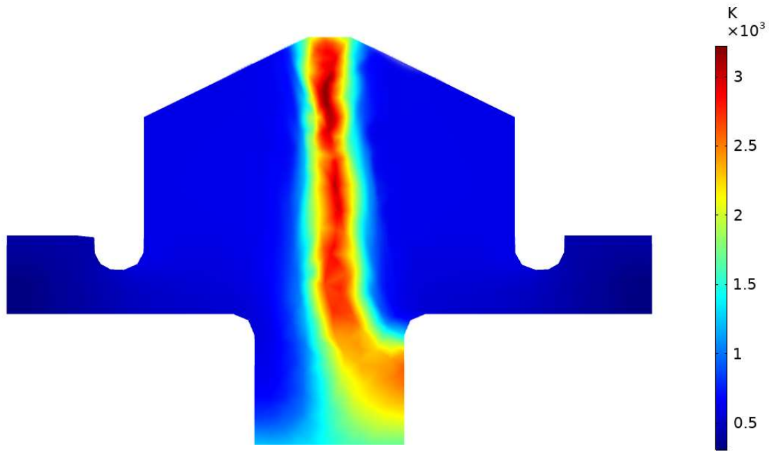
Figure 9: Calculated 2D gas temperature profile in the GAP for a pure (50/50) CO 2 -CH 4 plasma, at 10 L/min and 0.3 A electric current.
