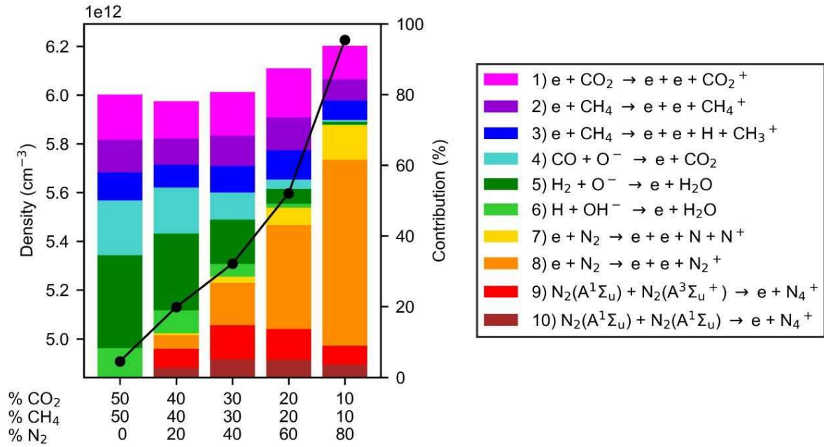
Figure 11: Calculated electron density (black line, left y-axis) as a function of N 2 fraction, at a constant gas temperature of 3500 K and power density of 4.5 kW cm -3 . The coloured bars (right y-axis) show the contribution of the dominant electron formation reactions across the different gas mixtures. The values are determined for a plasma residence time of 1 ms, which is comparable to the residence time in the plasma obtained in the 3D simulations based on the experimental conditions.
