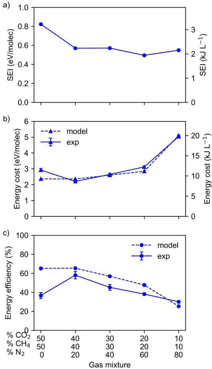
Figure 6: a) Experimental SEI at a constant plasma current of 0.3 A, (b) experimental and calculated energy cost, and (c) experimental and calculated energy efficiency, as a function of \text{N}_2 fraction. For all three figures, the experiments were performed in triplicate, but the error bars on the experimental results are mostly too small to be visible.
