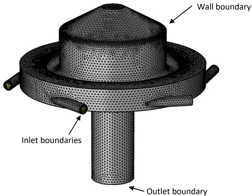
Figure 2: Computational domain of the turbulent flow model. The inlets, outlet and wall boundaries are indicated.
