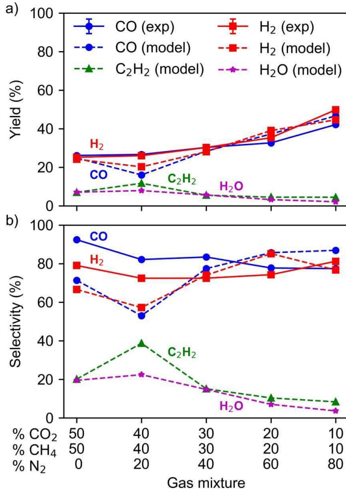
Figure 5: Experimental and calculated product (a) yields and (b) selectivities, as a function of N_2 fraction. The experiments in both figures were performed in triplicate, but the error bars on the experimental results are too small to be visible.
