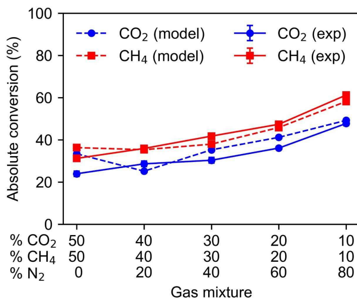
Figure 4: Experimental and calculated absolute CO 2 and CH 4 conversion as a function of N 2 fraction.
