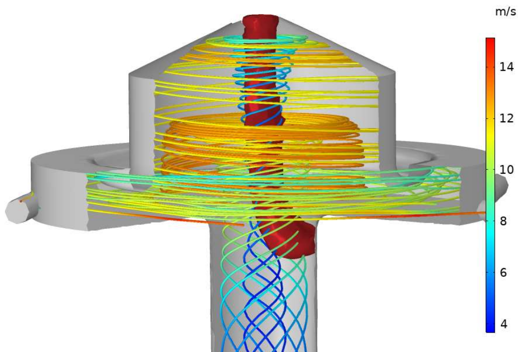
Figure 8: Calculated gas velocity streamlines (see colour scale at the right) and arc formation in the GAP reactor for a 10 L/min 50/50 CO 2 /CH 4 flow. The results look the same for all gas mixtures investigated.
