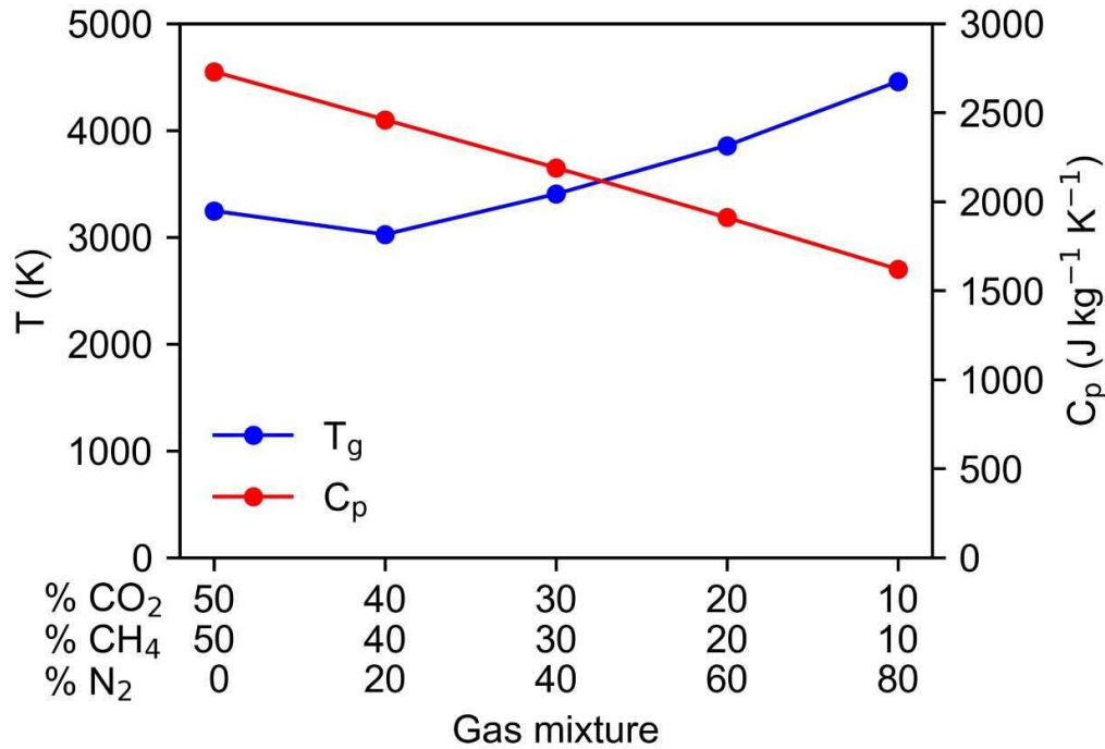
Figure 10: Maximum calculated gas temperature in the plasma (arc centre) (blue) and isobaric heat capacity of the CO 2 -CH 4 -N 2 gas mixture at 3000 K (red), as a function of the N 2 fraction.
