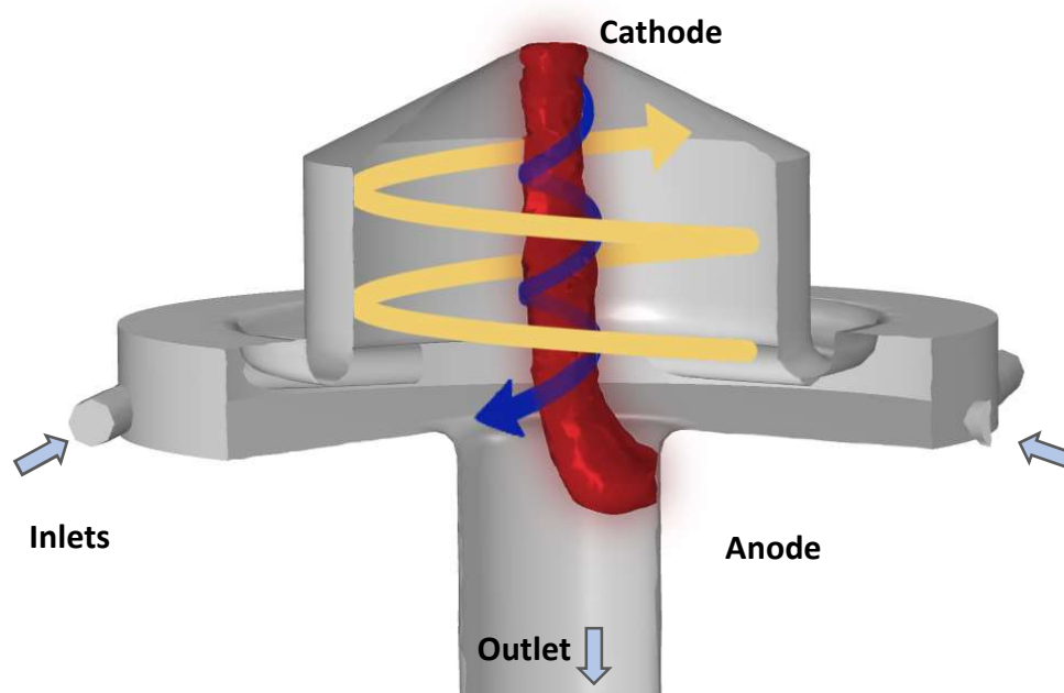
Figure 1: Schematic picture of the GAP reactor, with illustration of the outer and inner vortex gas flows (yellow and blue arrows), and the plasma arc (red). The reactor body is at cathode potential while the outlet functions as anode. The arc is formed between the top of the cathode (top of the reactor body) and anode (outlet). The tangential gas inlets and the outlet of the reactor are indicated with arrows.
