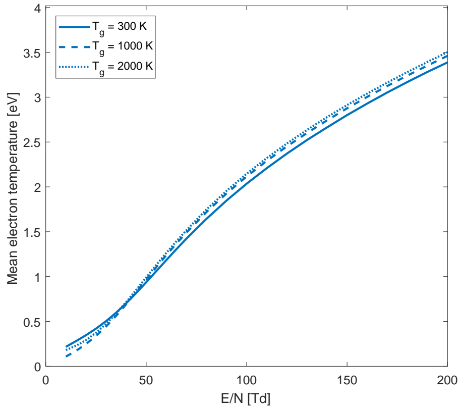
Figure 4: Mean electron temperature averaged over the plasma for an ionization degree \alpha_i = 10^{-6} and three different gas temperature (300 K, 1000 K and 2000 K).
