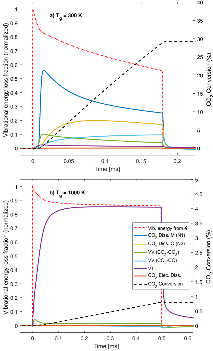
Figure 3: Vibrational energy loss processes (left y-axis) and CO 2 conversion (right y-axis) as a function of time for a reduced electric field of 50 Td, an ionization degree of 10^{-6} , a pressure of 100 mbar and a gas temperature of 300 K (panel a, top) and 1000 K (panel b, bottom). The energy loss is normalized to the maximum of the total energy that the CO 2 vibrational levels received from the electrons.
