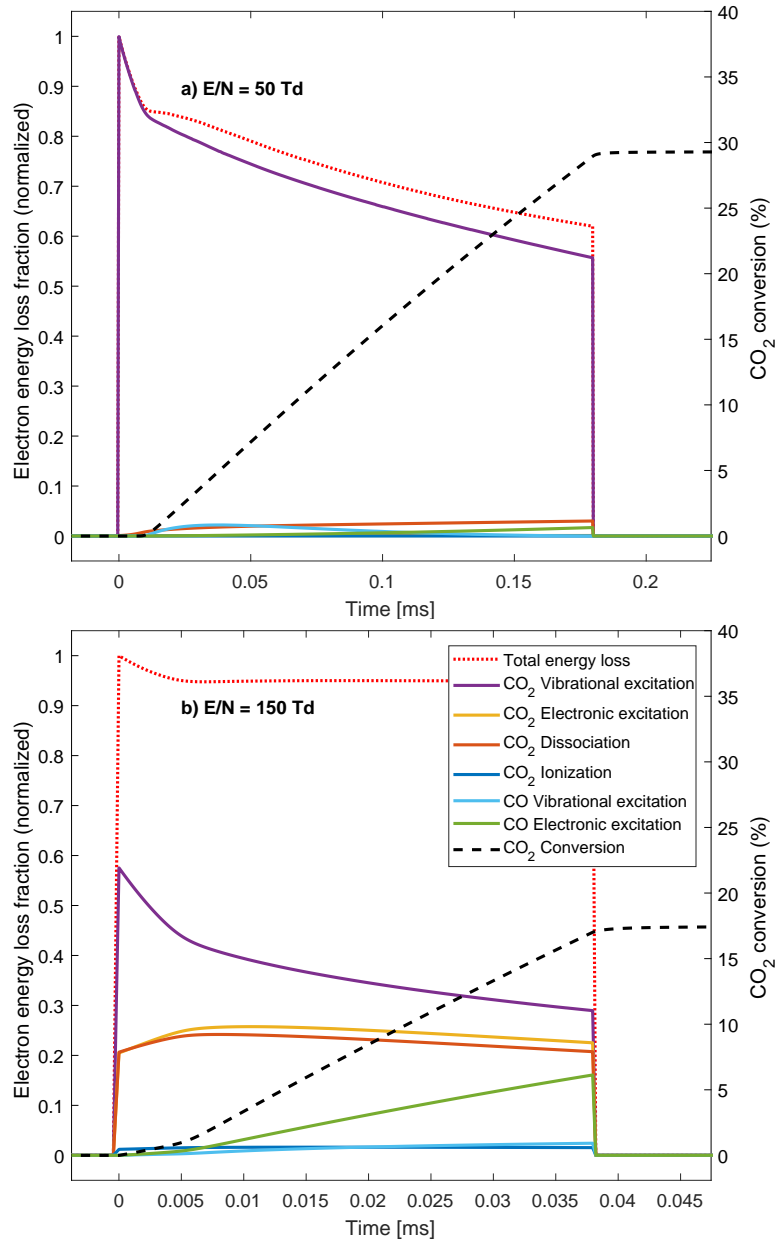
Figure 2: Electron energy loss fractions (left y-axis) and CO 2 conversion (right y-axis) as a function of time for a gas temperature of 300 K, an ionization degree of 10^{-6} , a pressure of 100 mbar and a reduced electric field of 50 Td (panel a, top) and 150 Td (panel b, bottom). The energy losses are normalized to the maximum of the total energy applied to the electrons.
