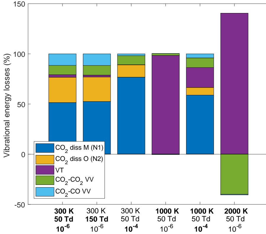
Figure 6: Relative contribution of the main processes responsible for the vibrational energy losses integrated over time, for different conditions of gas temperature, reduced electric field and ionization degree, and at a pressure of 100 mbar. The parameters written in bold indicate the differences with the first case.
