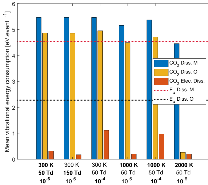
Figure 9: Mean vibrational energy consumption per dissociation event for different conditions (as in figure 6), integrated over time, and at a pressure of 100 mbar. The parameters written in bold indicate the differences with the first case. The dotted lines show the activation energy of reactions (N1) and (N2), i.e. dissociation upon impact by any molecule M and upon O atom impact, in red and in black, respectively.
