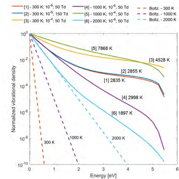
Figure 7: Vibrational distribution functions (VDFs) of the asymmetric mode vibrational levels of \text{CO}_2 at half of the 'plasma residence time', for various conditions, as also presented in figure 6. The legend of each curve indicates the gas temperature, the ionization degree and the reduced electric field, respectively, and the numbers of the curves correspond to the cases of figure 6. The vibrational temperature is indicated next to each number. The Boltzmann distributions corresponding to the gas temperatures considered here are shown with dashed lines.
