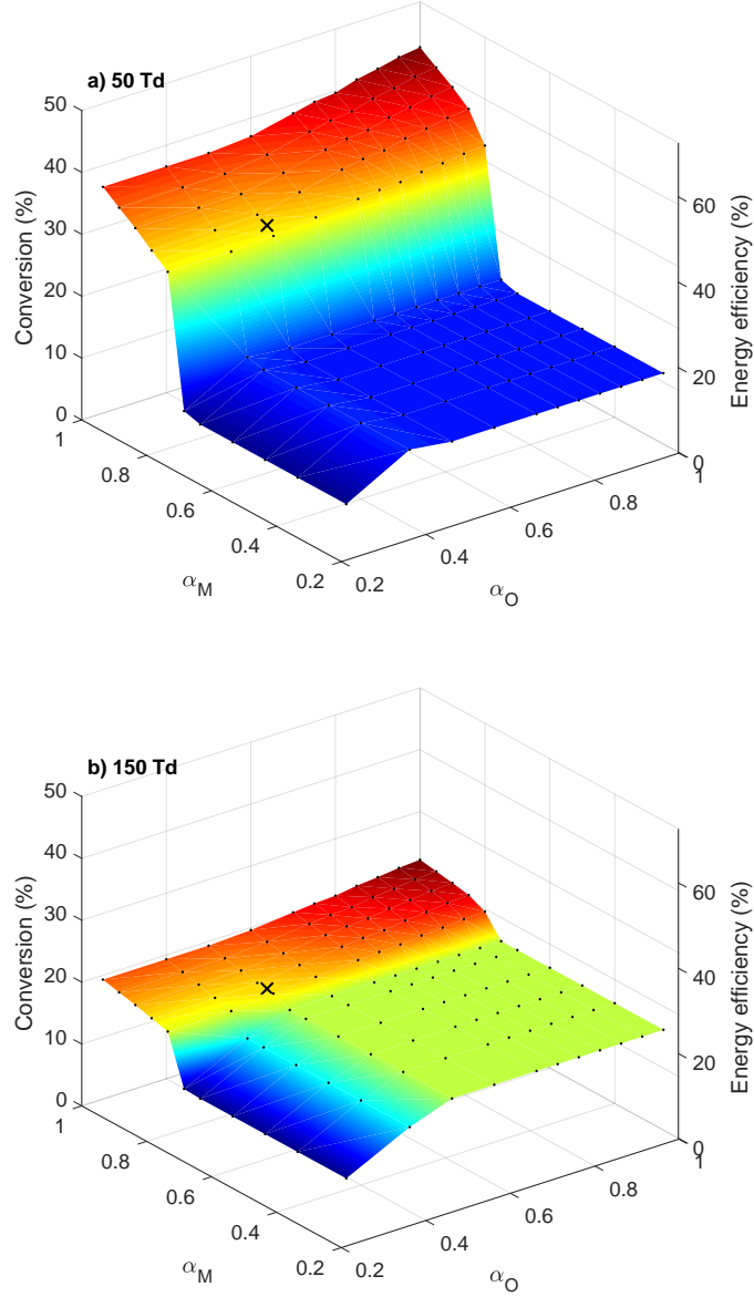
Figure 10: CO 2 conversion and energy efficiency as a function of the \alpha_M and \alpha_O parameters, for a gas temperature of 300 K, an ionization degree of 10^{-5} , a pressure of 100 mbar, and a reduced electric field of 50 Td (panel a, top) and 150 Td (panel b, bottom). The cross symbols indicate the standard values of \alpha_M and \alpha_O , used up to now in the model, i.e., \alpha_M = 0.82 and \alpha_O = 0.5 .
