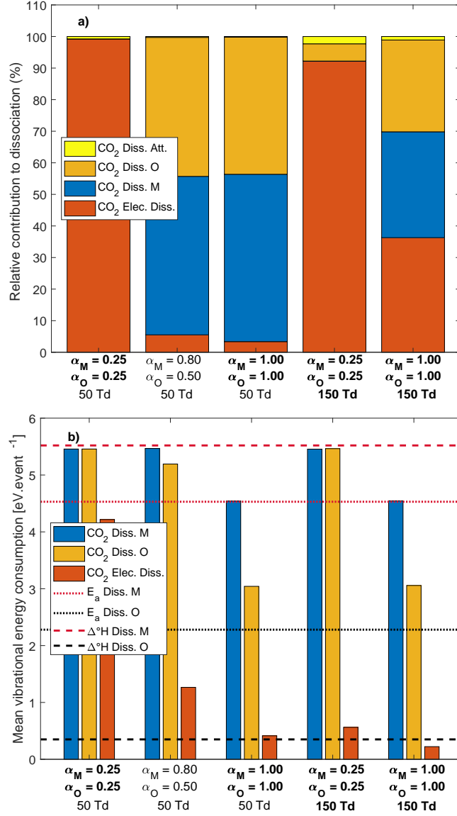
Figure 11: Main processes responsible for CO 2 dissociation (a) and mean vibrational energy consumption per dissociation event (b) for different conditions, integrated over time, for a temperature of 300 K, an ionization degree of 10^{-5} and a pressure of 100 mbar. The parameters written in bold indicate the differences with the second case. The dotted and dashed lines in (b) show the activation energy and the standard reaction enthalpy, respectively, of reactions (N1) and (N2), i.e. dissociation upon impact by any molecule M and upon O atom impact, in red and in black, respectively.
