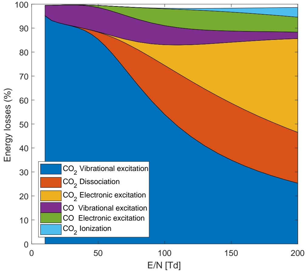
Figure 5: Relative contribution of the main processes responsible for the electron energy loss as a function of the reduced electric field E/N , for a gas temperature of 300 K, an ionization degree of 10^{-6} and a pressure of 100 mbar. The electron energy losses are integrated over the plasma for each value of E/N .
