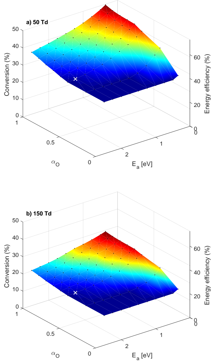
Figure 12: CO 2 conversion and energy efficiency as a function of the \alpha_O parameter and the activation energy of reaction N2, for a gas temperature of 300 K, an ionization degree of 10^{-5} , a pressure of 100 mbar, and a reduced electric field of 50 Td (panel a, top) and 150 Td (panel b, bottom). The cross symbols indicate the standard values of E_a(\text{N2}) and \alpha_O , used up to now in the model, i.e., E_a(\text{N2}) = 2.28 eV and \alpha_O = 0.5 .
