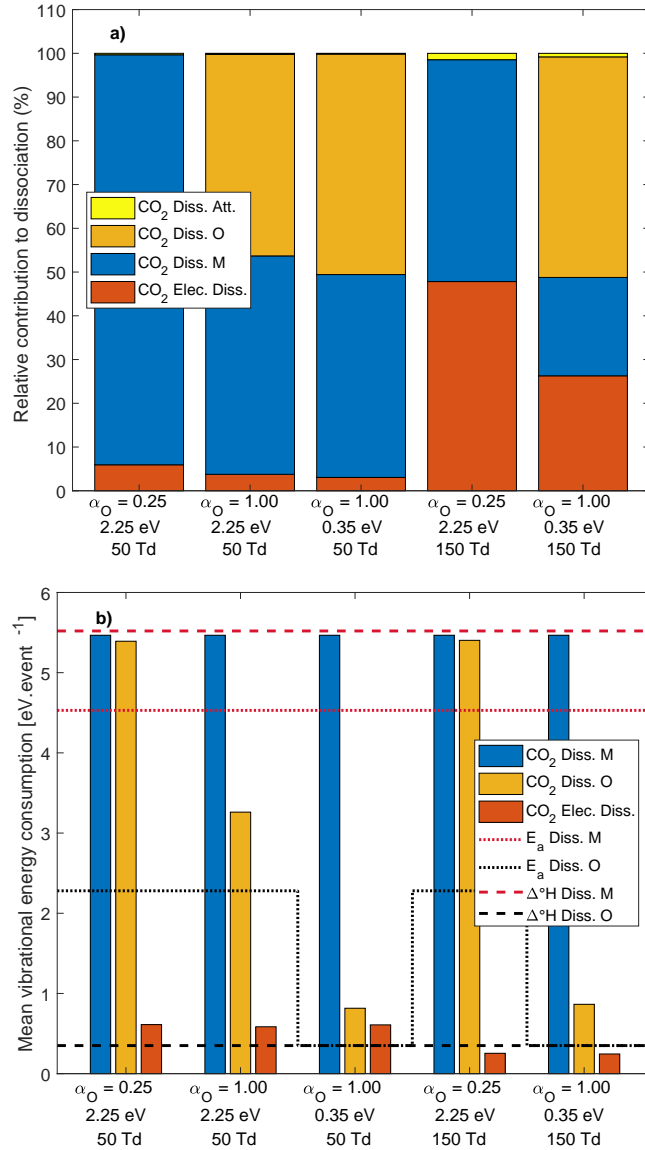
Figure 13: Main processes responsible for CO 2 dissociation (a) and mean vibrational energy consumption per dissociation event (b) for different conditions, integrated over time, for a temperature of 300 K, an ionization degree of 10^{-5} and a pressure of 100 mbar. The dotted and dashed lines in (b) show the activation energy and the standard reaction enthalpy, respectively, of reactions (N1) and (N2), i.e. dissociation upon impact by any molecule M and upon O atom impact, in red and in black, respectively. Note that the activation energy of reaction N2 is not the same for the different cases, as indicated below the x-axis for each case.
