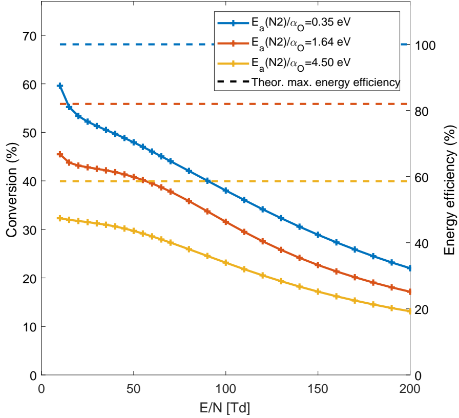
Figure 14: \text{CO}_2 conversion (left y-axis) and corresponding energy efficiency (right y-axis) as a function of the reduced electric field E/N , for three values of E_a(\text{N}_2)/\alpha_O (0.35 eV, 1.64 eV, 4.50 eV), and for a gas temperature of 300 K, and an ionization degree of 10^{-4} . The dashed lines indicate the corresponding maximum theoretical energy efficiency using equation eq. (11) in each case. The value of E_a(\text{N}_1)/\alpha_M is taken equal to 5.52 eV, as in our standard model.
