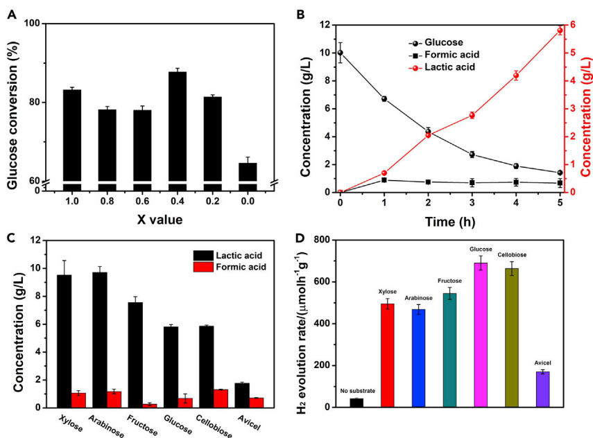
Figure 4. Glucose conversion and product analysis
