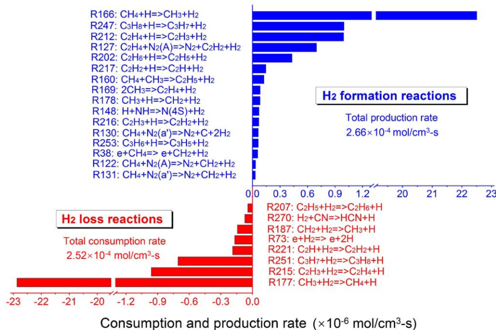
Fig. 8 Dominant pathways and corresponding reaction rates for the formation and loss of \text{H}_2 ( \text{CH}_4/\text{N}_2 = 0.10 )
