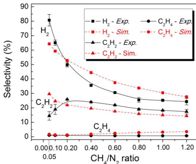
Fig. 4 Simulated and experimental selectivity of gas products as a function of \text{CH}_4/\text{N}_2 molar ratio
