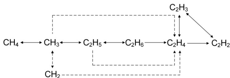
Fig. 14 Dominant reaction paths for the formation of \text{C}_2 hydrocarbons. The dashed lines represents the paths with minor contributions.
