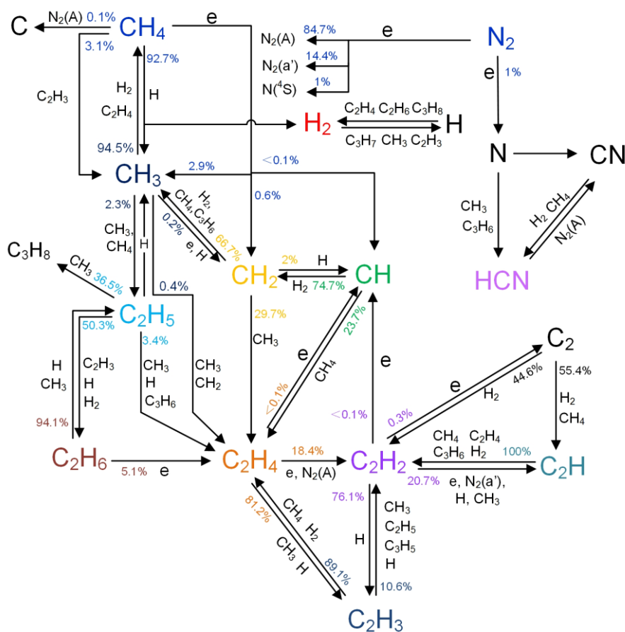
Fig. 13 Reaction scheme to illustrate the dominant pathways of the plasma chemistry in RGA plasma assisted \text{CH}_4 decomposition process in \text{N}_2 . The percentages on the arrowed lines represent the relative contributions of different paths for the depletion of corresponding species at \text{CH}_4/\text{N}_2 = 0.40 .
