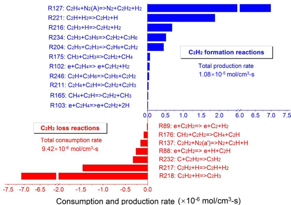
Fig. 11 Dominant pathways and corresponding reaction rates for the formation and loss of \text{C}_2\text{H}_2 ( \text{CH}_4/\text{N}_2 = 0.10 )
