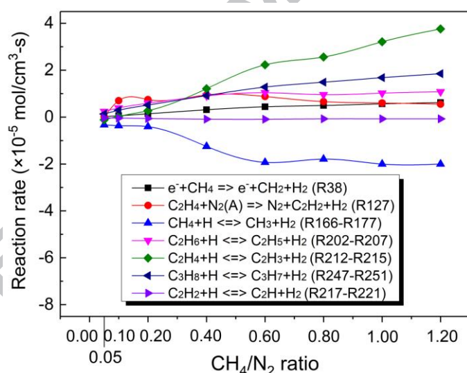
Fig. 10 Net reactions rates of various H 2 production processes as a function of CH 4 /N 2 molar ratio.
