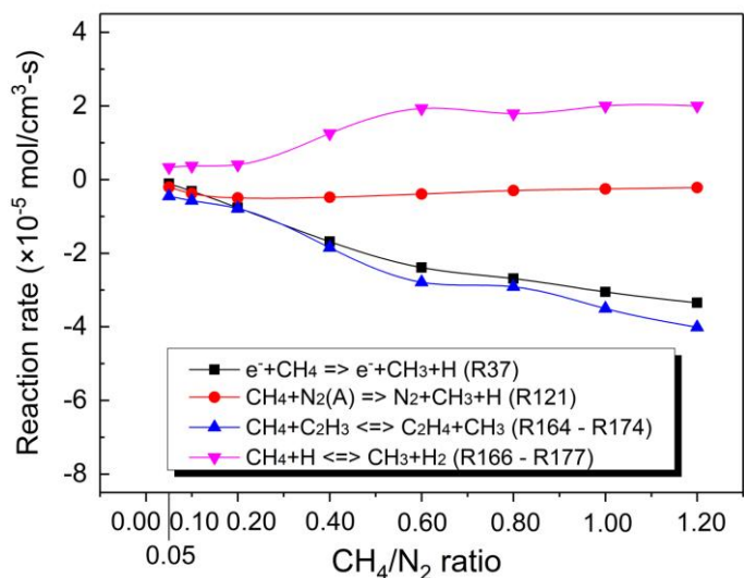
Fig. 7 Net reactions rates of various \text{CH}_4 conversion processes as a function of \text{CH}_4/\text{N}_2 molar ratio.
