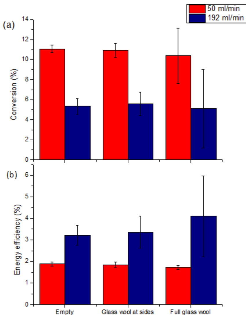
Figure 5: Conversion (a) and energy efficiency (b) in an empty reactor (left), an empty reactor with glass wool at the sides (middle) and a reactor completely filled with glass wool (right) at two different flow rates, for 100 Watt power, alumina dielectric barrier, stainless steel electrode, at 23.5 kHz and 4.5 mm gap.
