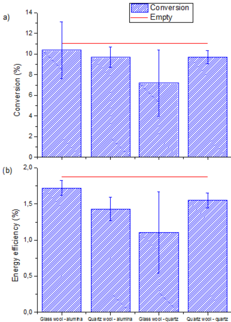
Figure 7: Conversion (a) and energy efficiency (b) for two different dielectric barriers and packing materials, as indicated in the x-axis, at 50 ml/min, for 100 Watt power, 4.5 mm gap, 23.5 kHz and a stainless steel electrode.
