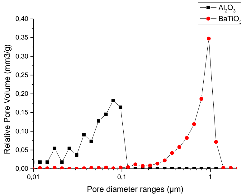
Figure 3: Relative pore volume for Al 2 O 3 and BaTiO 3 beads
