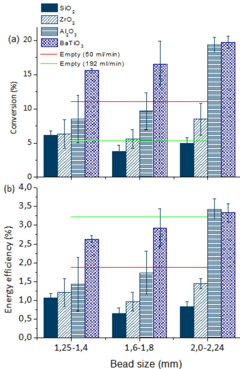
Figure 2: Conversion (a) and energy efficiency (b) as a function of bead size (diameter) for different bead materials, for an alumina dielectric barrier, 4.5 mm gap, stainless steel outer electrode, 23.5 kHz, at 50 ml/min gas flow rate, and 100 Watt power. The error bars are calculated based on 12 GC measurements. Comparison is also made with the results for an empty reactor (i.e., without packing), both at the same flow rate (50 ml/min) and the same residence time as in the packed bed reactor (i.e., 5.52 sec, corresponding to a flow rate of 192 ml/min).
