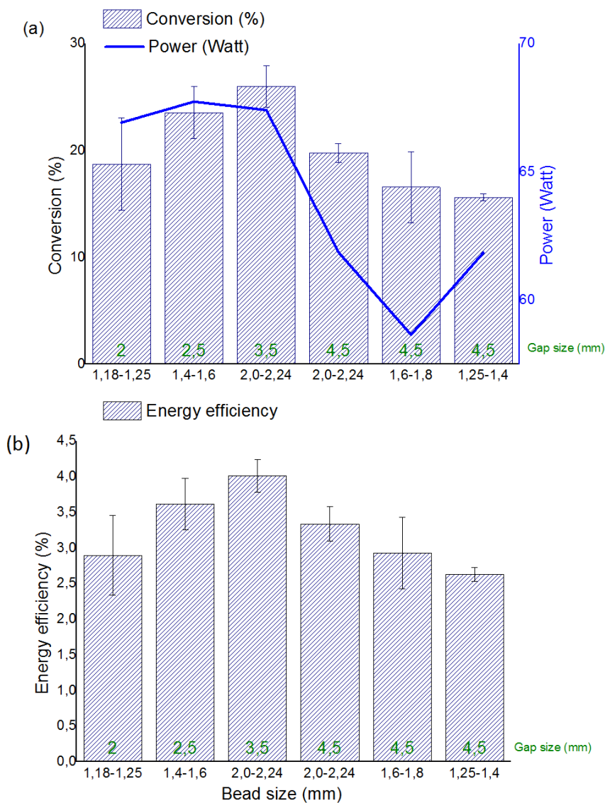
Figure 4: Conversion (a) and energy efficiency (b) as a function of bead size and gap size (indicated at the bottom of the columns, in mm), for BaTiO 3 beads, an alumina dielectric barrier, stainless steel outer electrode, 23.5 kHz, at 50 ml/min, for 100 Watt input power. The plasma power (Watt) is indicated by a blue line.
