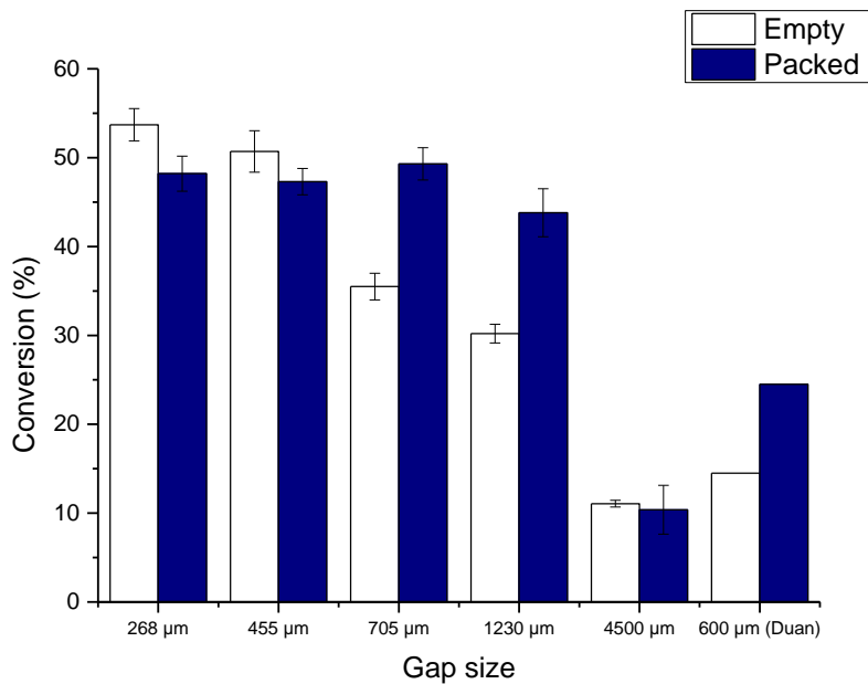
Figure 6: Effect of a glass wool packing on the CO 2 conversion, for different gap sizes, in comparison with the results by Duan et al. for a quartz wool packing
