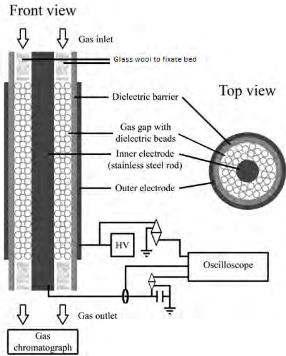
Figure 1: Setup of the packed bed DBD reactor used in this study (adapted from ref[33]) . The packing is illustrated with beads but can also be filled with glass wool or quartz wool.
