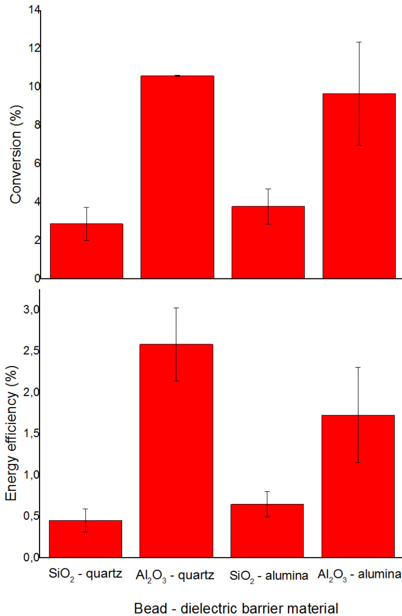
Figure 8: Conversion (a) and energy efficiency (b) for silica and alumina spheres, with quartz and alumina dielectric barriers, at 50 ml/min, for 100 Watt power, 4.5 mm gap, 23.5 kHz and a stainless steel electrode.
