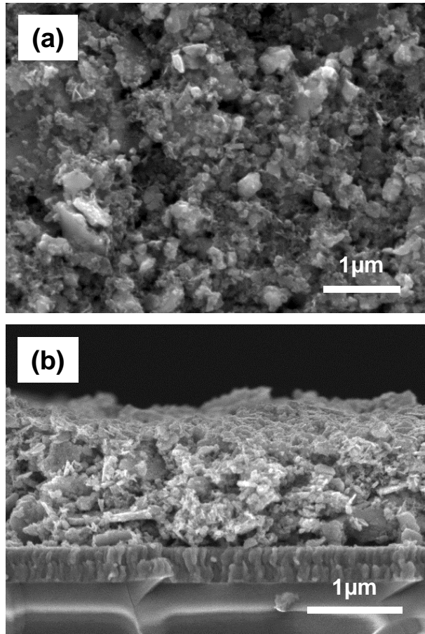
Figure 5, Top (a) and cross-sectional (b) SEM view of the Cu-In-Se alloy nanopowder coating.
