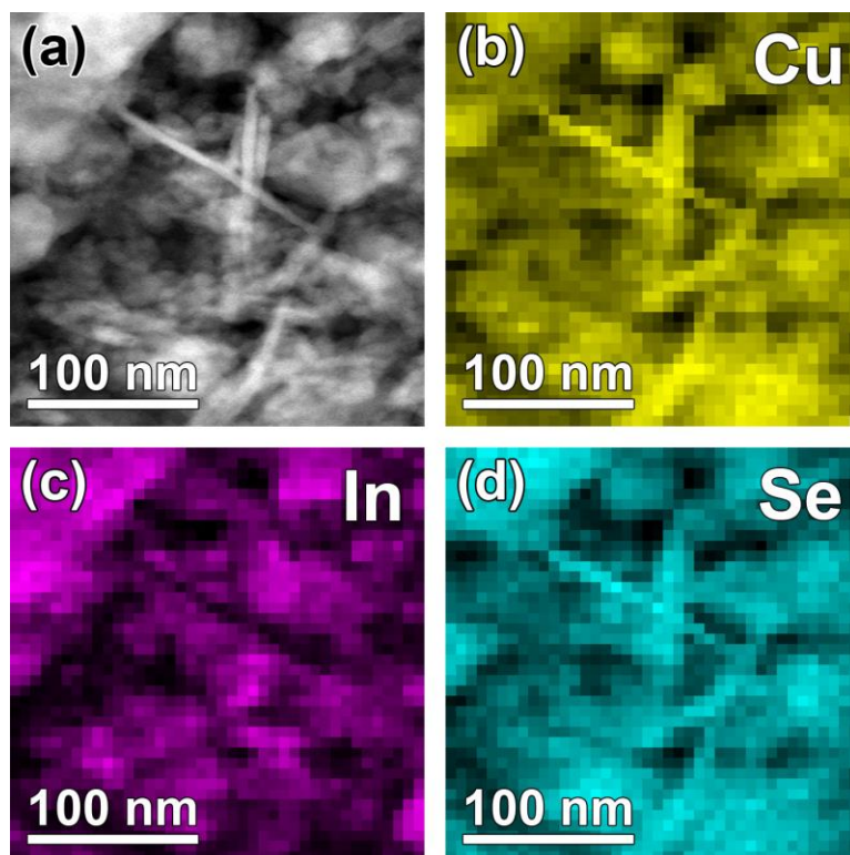
Figure 4, HAADF-STEM image from Cu-In-Se alloy nanopowder (a) and STEM-EDS elemental maps of copper (b) indium (c) and selenium (d).
