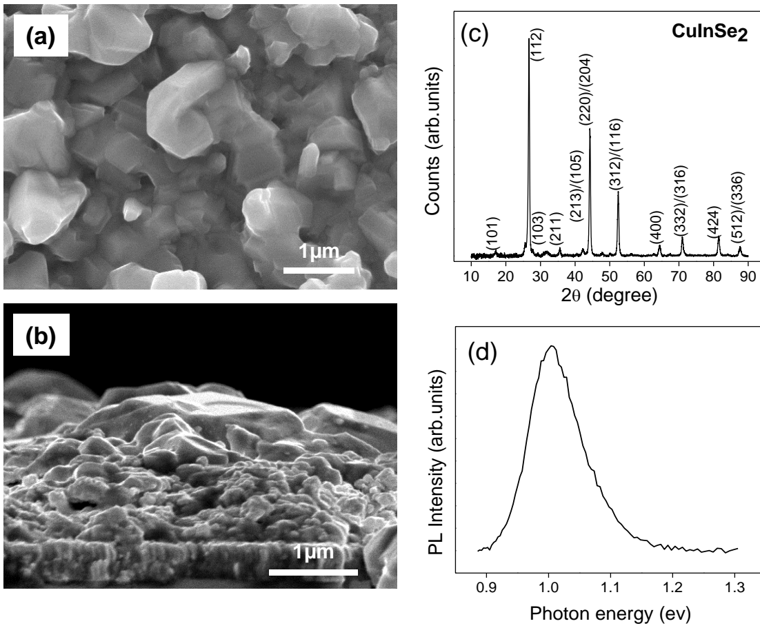
Figure 6, Top (a) and cross-sectional (b) SEM image of the CuInSe 2 film after selenization together with the XRD pattern (c) and Photoluminescence spectroscopy spectrum (d)
