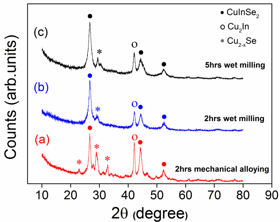
Figure 2, XRD patterns of mechanically synthesized Cu-In-Se alloy powder after dry milling for 2 hrs at 350 rpm (a) and Cu-In-Se alloy nanopowder after additional wet milled for 2 hrs (b) and 5 hrs (c) at 350 rpm.
