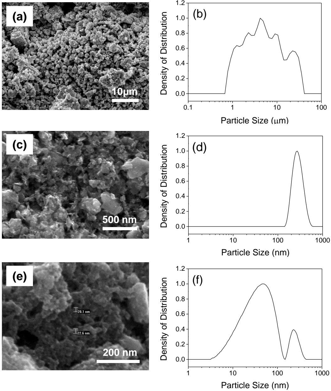
Figure 1, SEM images and particle size distributions of the Cu-In-Se alloy powder after 2 hrs of mechanical alloying (a,b), and Cu-In-Se alloy nanopowders after 2 hrs (c,d) and 5 hrs (e,f) of additional wet ball milling.
