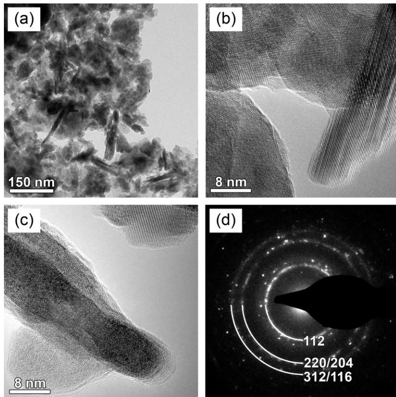
Figure 3, TEM image showing Cu-In-Se alloy nanopowder agglomerate nanostructure (a) HR TEM image from crystalline nanoparticles (b) HR TEM image from amorphous a rod-like nanoparticle (c) Electron Diffraction (ED) pattern acquired from a Cu-In-Se alloy nanopowder (d), diffraction rings correspond to the tetragonal \text{CuInSe}_2 phase, scattered reflections can be attributed to the CuSe phase.
