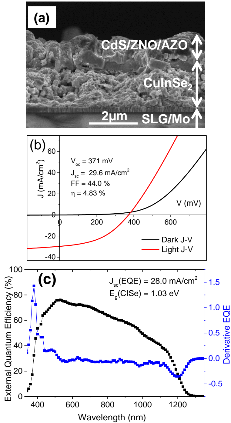
Figure 7, Cross-sectional SEM image of the SLG/Mo/ CuInSe 2 /CdS/ZnO/AZO solar cell, with the printed based CuInSe 2 absorber layer (a) Current-voltage curve of the device under dark and light conditions (b) and External quantum efficiency (EQE) of the device as function of the wavelength (c)
