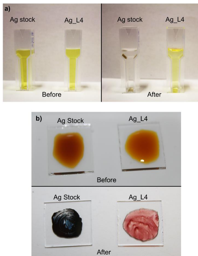
Figure 4. a) Photographic images showing the effect of salt addition on unprotected Ag versus protected Ag_L4 colloidal nanoparticles and b) Photographic images showing the effect of hot air treatment on unprotected Ag versus protected Ag_L4 nanoparticles.
