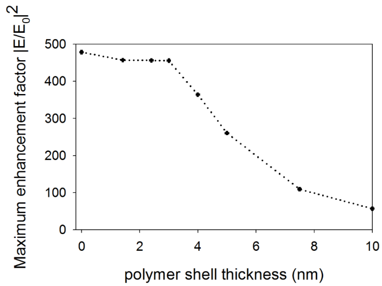
Figure 6. Effect of polymer shell thickness on maximum enhancement factor near the outer surface of core shell nanoparticle, as determined from finite element simulations.
