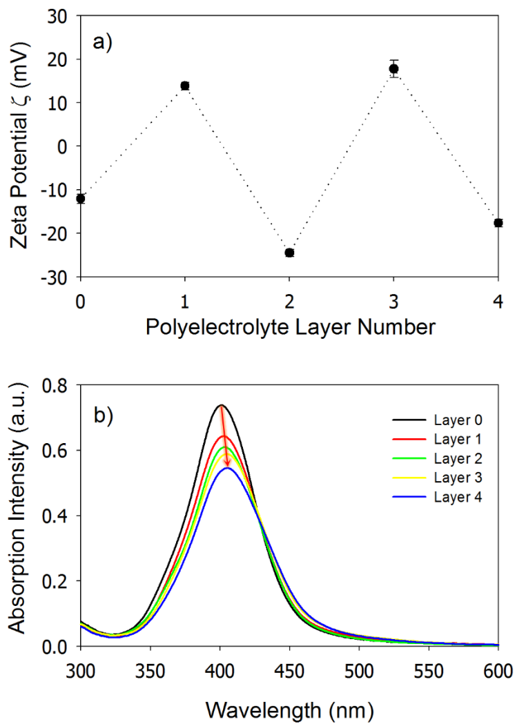
Figure 1. a) Zeta potential of core-shell silver nanoparticles \text{Ag}/(\text{PAH}/\text{PAA})_2 as a function of adsorbed polyelectrolyte layer. b) UV-vis absorption spectra of core-shell silver nanoparticles as a function of adsorbed polyelectrolyte layer. The red arrow indicates the red shift in SPR peak position.
