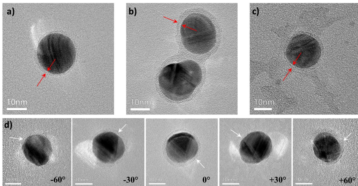
Figure 3. Silver core-shell nanoparticles with silver core and an ultrathin shell composed of a) four polyelectrolyte layers (Ag_L4) \text{Ag}/(\text{PAH}/\text{PAA})_2 of thickness 1.4 \pm 0.4 nm, b) eight polyelectrolyte layers (Ag_L8) \text{Ag}/(\text{PAH}/\text{PAA})_4 of thickness 2.4 \pm 0.6 nm, c) four polyelectrolyte layers (Ag_L4) \text{Ag}/(\text{PAH}/\text{PSS})_2 of thickness 1.6 \pm 0.4 nm, d) TEM tilt series of Ag_L8 core-shell nanoparticles. All the inset bars represent a scale of 10 nm. The shell thickness distribution is based on 100 measurements.
