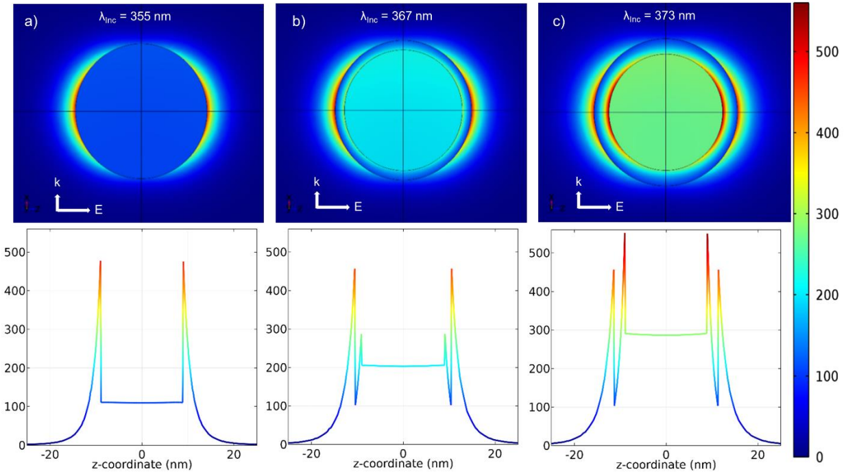
Figure 5. Electric field distribution maps (|E|/|E_0|)^2 for a) bare silver nanoparticle, b) silver encapsulated by a polymer shell of thickness 1.4 nm, alike Ag_L4 and c) silver encapsulated by a polymer shell of thickness 2.4 nm, alike Ag_L8. The field enhancement along the Z-axis, i.e. in the direction of polarization, is plotted below the corresponding field maps.
