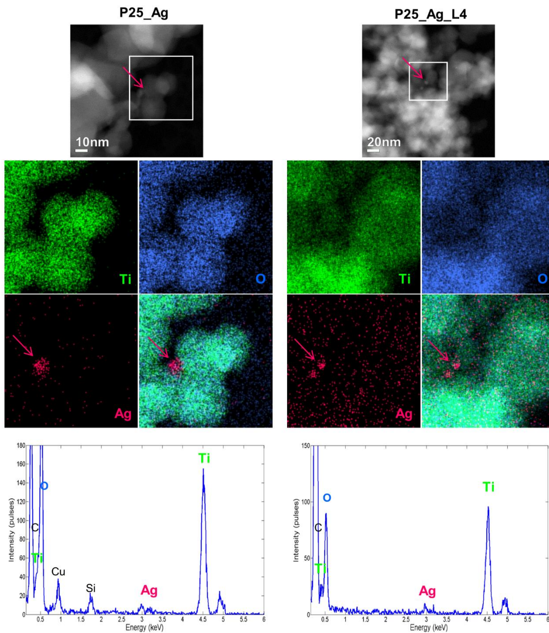
Figure 7. High angular annular dark field – STEM (HAADF-STEM) images (top) and EDX spectra (bottom) of P25_Ag (left) and P25_Ag_L4 (right) samples. The elemental maps show the presence of the Ag nanoparticles on the surface of TiO 2 .
