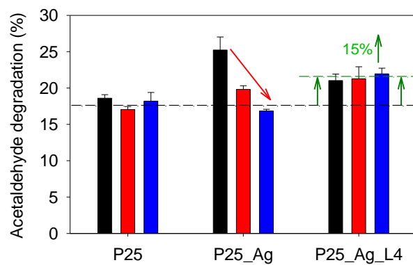
Figure 8. Long-term photocatalytic activity test. The photocatalytic degradation of gaseous acetaldehyde is evaluated at t = 0 (i.e. freshly prepared, black), after three weeks (red) and after 16 weeks (blue) of ageing in air.
