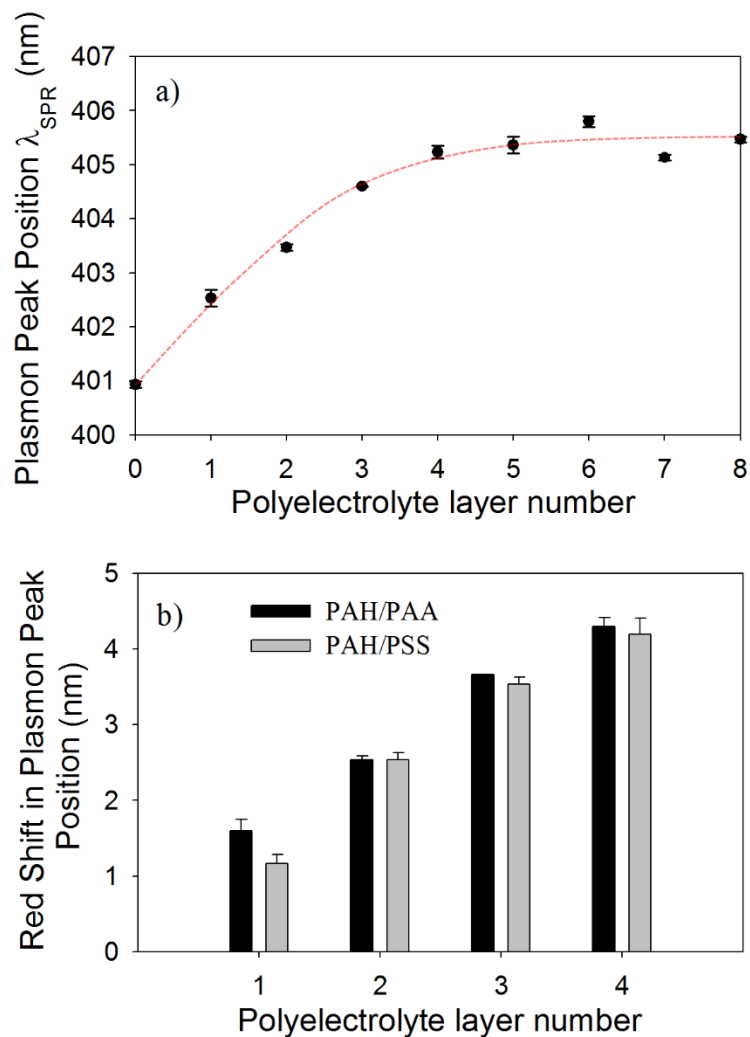
Figure 2 a). Plasmon peak position of the silver core-shell nanoparticles as a function of number of adsorbed PAH/PAA polyelectrolyte layers. b) Comparison of red shift in SPR peak position in different polyelectrolyte systems PAH/PAA and PAH/PSS.
