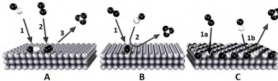
Figure 4 – The three prototypical thermal surface reaction mechanisms, A) Langmuir-Hinshelwood; B) Eley-Rideal; and C) Mars – Van Krevelen. Reproduced with permission from [57].
