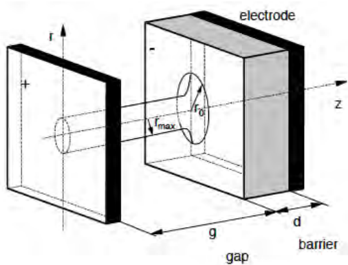
Figure 2 – Structure of a single microdischarge in a DBD. Reproduced with permission from [38].
