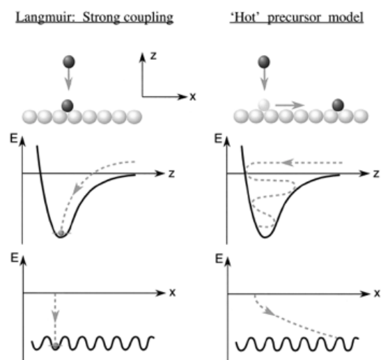
Figure 7 – Schematic dynamics for adsorption following (left panel) the Langmuir concept or strong coupling limit, and (right panel) the hot precursor model. Reproduced with permission from [52].
