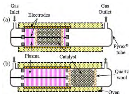
Figure 1 – Typical (a) single-stage and (b) two-stage dielectric barrier discharge setup used in plasma catalysis. Reproduced with permission from [36].
