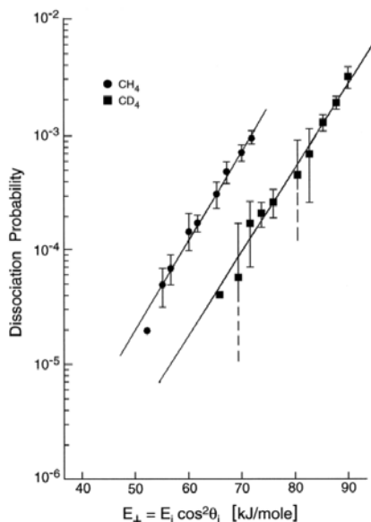
Figure 6 – Measured dissociation probabilities of CH 4 and CD 4 impinging onto a Ni(111) surface as a function of the normal component of translational energy. Reproduced with permission from [64, 65].
