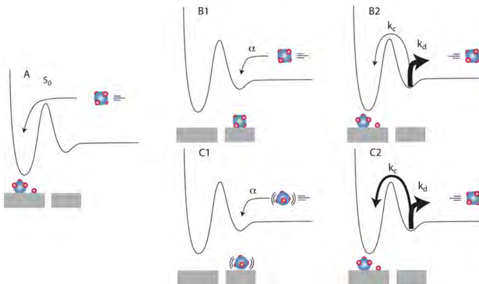
Figure 5 – Schematic representation of possible reaction mechanisms in methane adsorption. Reproduced with permission from [63].
