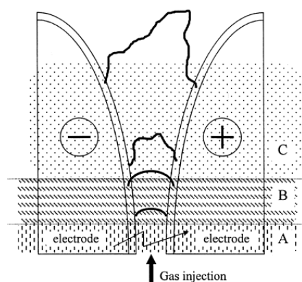
Figure 3 – Typical gliding arc setup, showing the three stages of gliding arc evolution: (A) reagent gas breakdown; (B) equilibrium heating phase; and (C) non-equilibrium reaction phase. Reproduced with permission from [47].
