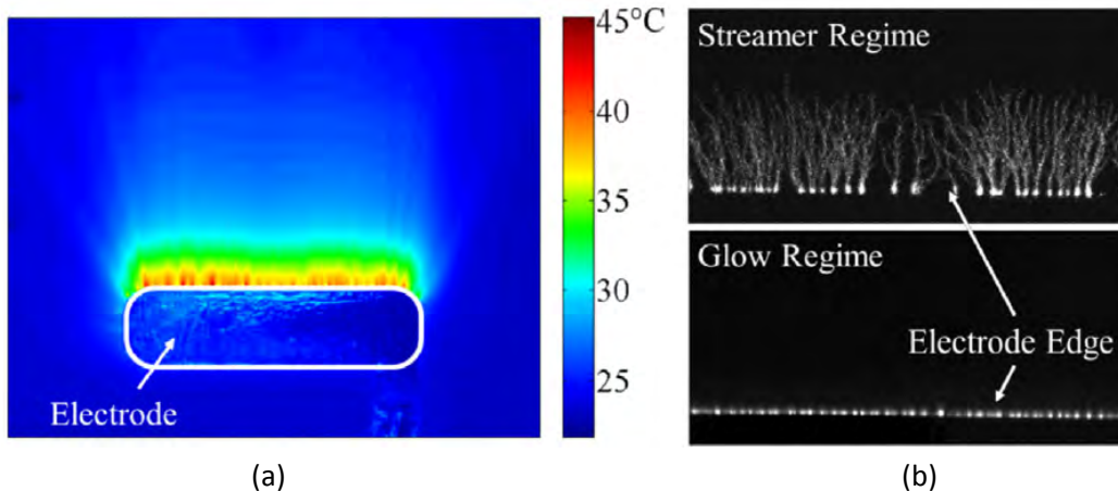
Figure 10 – (a) Absolute temperature distribution in a DBD, showing the occurrence of surface hot spots, and (b) iCCD images of the streamer and glow discharge regimes in a DBD. Reproduced with permission from [95].
