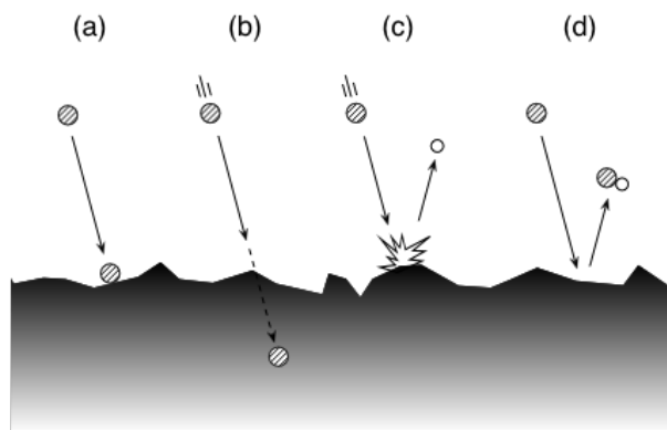
Figure 9 – Schematic representation of several surface modification processes. (a) Poisoning by strong adsorption and blocking active catalytic sites; (b) implantation of the highly energetic impinging particle in the bulk of the substrate; (c) sputtering by energetic ion impact; and (d) etching, through the formation of a volatile compound.
