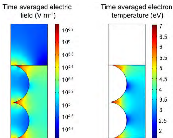
Figure 11 – Calculated (left panel) time averaged electric field and (right panel) time averaged electron temperature, showing the significant field enhancement and electron temperature resulting from the packed bed effect. Reproduced with permission from [104].
