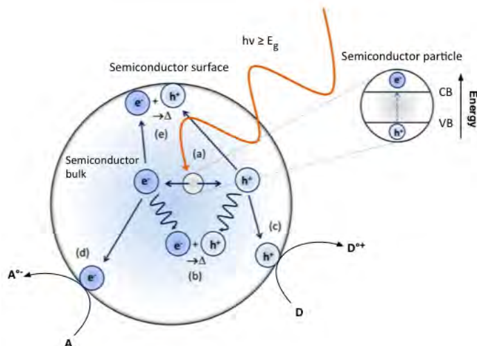
Figure 8 - Photo-excitation of a semiconducting metal oxide particle (a) and the de-excitation events; (b) electron-hole recombination within the semiconductor bulk, (c) oxidation of surface adsorbed electron donors, (d) reduction of surface adsorbed electron acceptors and (e) electron-hole recombination at the semiconductor surface. Reproduced with permission from [77].
