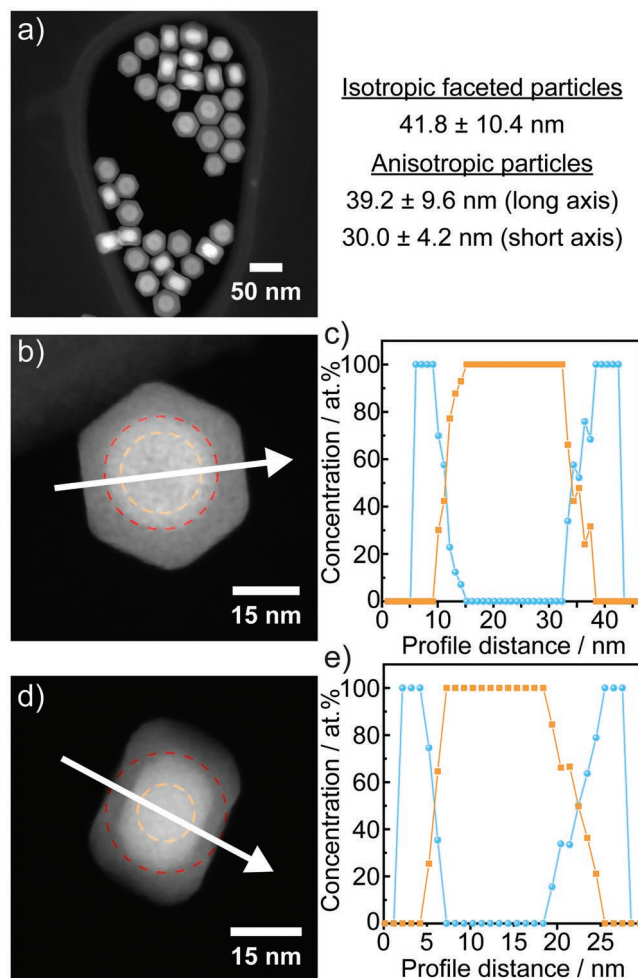
Figure 5. High-angle annular dark-field scanning transmission electron microscopy (HAADF-STEM) images (a,b,d) and chemical concentration profiles (c,e) of the particles shown in the left column. The concentration profiles were obtained from energy dispersive X-ray spectroscopy (EDXS)/STEM line profiles after implementing the subshell approach for thick-shell C^{II}S^{II} hetero-nanocrystals (HNCs) synthesized from large \beta - NaErF_4 :Yb core particles with yttrium and sodium trifluoroacetates as shell precursors for b,c) isotropic and d,e) anisotropic HNCs. The erbium/ytterbium and yttrium concentration profiles are in orange and blue, respectively. On HAADF-STEM images (b,d), white arrows indicate the EDXS scan direction while red and orange dashed circles indicate the initial size of the starting core particles together with the real size of the pure core domain (as determined by EDXS), respectively.
