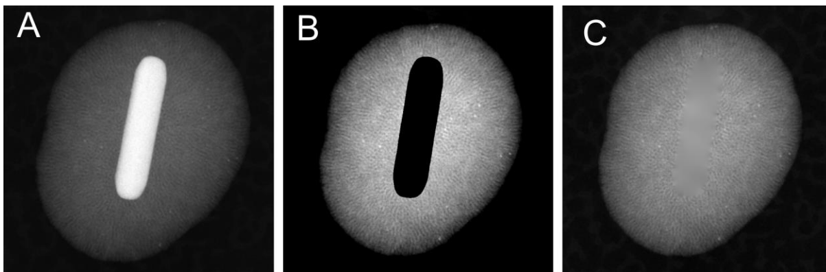
Figure 3. Different steps toward the optimization of the reconstruction of a ADF-STEM tilt series. (A) Micrograph acquired using ADF-STEM (B) After image segmentation, the pixels corresponding to the Au nanorod in \text{SiO}_2 were removed. (C) Final image after the inpainting procedure. The removed pixels were replaced by the surrounding texture.
