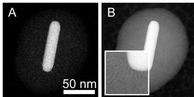
Figure 1. TEM image of a PTW Au@SiO 2 particle. (A) The micrograph was acquired using HAADF-STEM. The core can be clearly seen but the intensity from the shell is too low. (B) The micrograph was acquired using ADF STEM, showing that the intensity from the SiO 2 shell becomes prominent.
