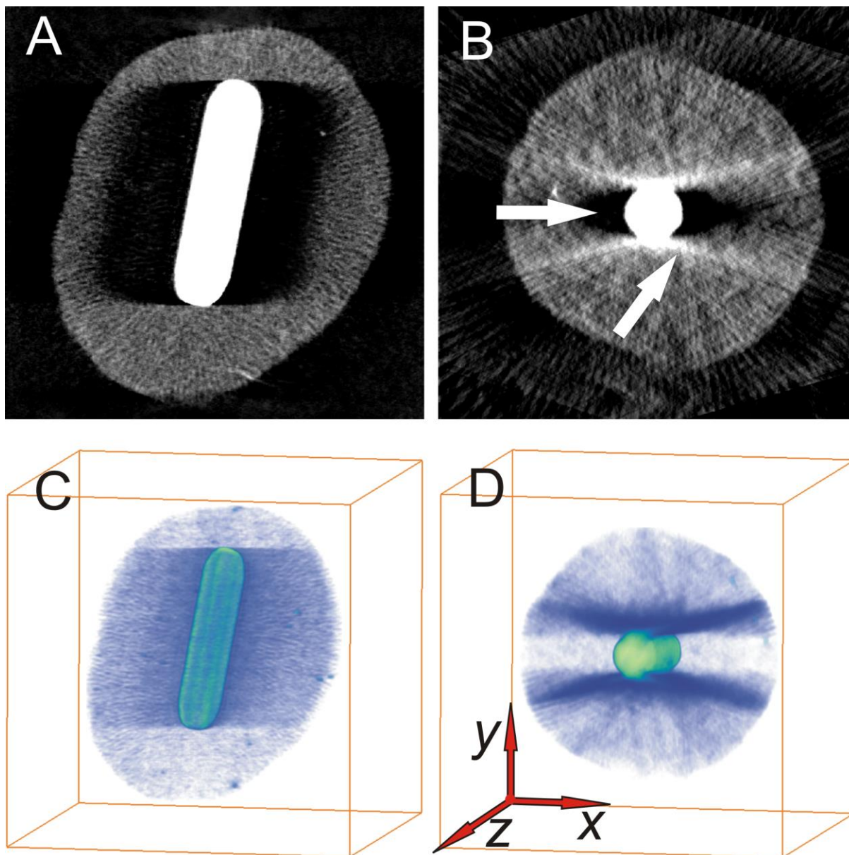
Figure 2. Reconstruction of a PTW Au@SiO 2 particle, using an ADF-STEM tilt series. (A,B) Slices through the silica coated PTW Au nanorod viewed in XZ (A) and XY (B) orientations. Dark and streaking artefacts can be observed in the vicinity of the Au nanorod and are highlighted with white arrows. (C,D) Volume renderings of the ADF-STEM reconstruction viewed along XZ and XY orientations. The Au nanorod is depicted in light green and the surrounding silica is shown in blue. Although information from silica is present in the reconstruction, the resolution of the reconstruction is limited by the artefacts.
