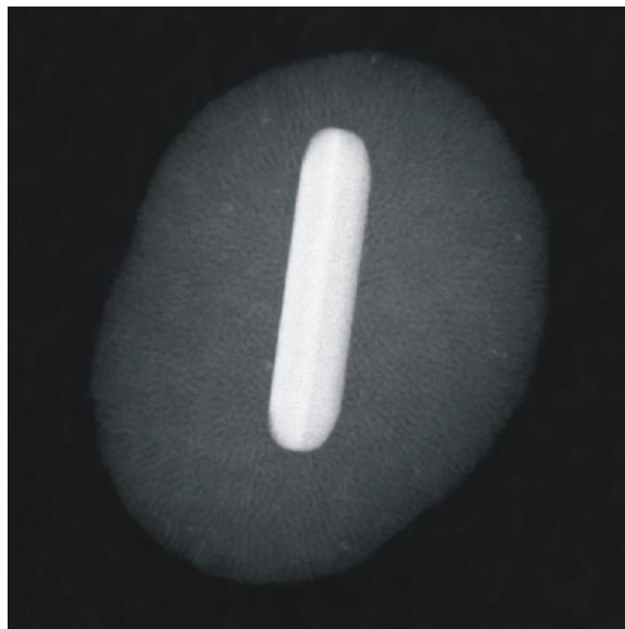
Figure S1. 2D ADF-STEM projection image of Au@mSiO 2 (See Video S1 for all projections in tilt series).
